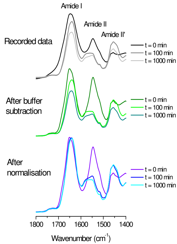
Figure 3.7: Buffer subtraction from the recorded data, and the normalization step with respect to the amide I band.
