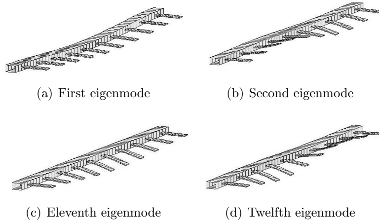
Figure 2.12: Eigenmodes of the two-scale model
