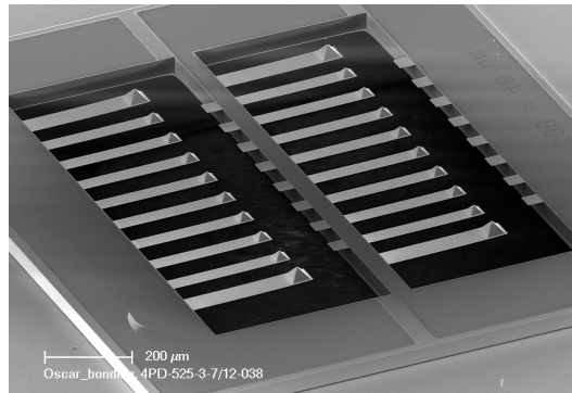
Figure 2.26: Example of an optimized design geometry. The larger cantilevers with larger and higher tip situated in the corner of the probe array are used to land and adjust the probe array onto the sample surface. Courtesy of André Meister and Thomas Overstolz, CSEM Neuchâtel Switzerland.
