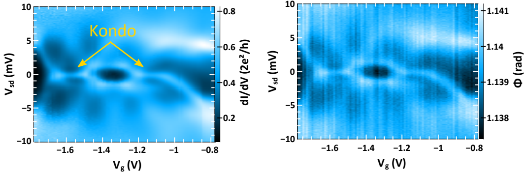
FIGURE 6.1: a : color scale plot of the differential conductance in unit of 2e^2/h in the gate voltage V_g bias voltage V_{sd} plane. Fourfold degeneracy is observable, with 2 Kondo ridges (orange arrows) corresponding to fillings N=1 and N=3 in the orbital. b : color scale plot of the transmitted RF signal's phase, simultaneously taken with (a).
