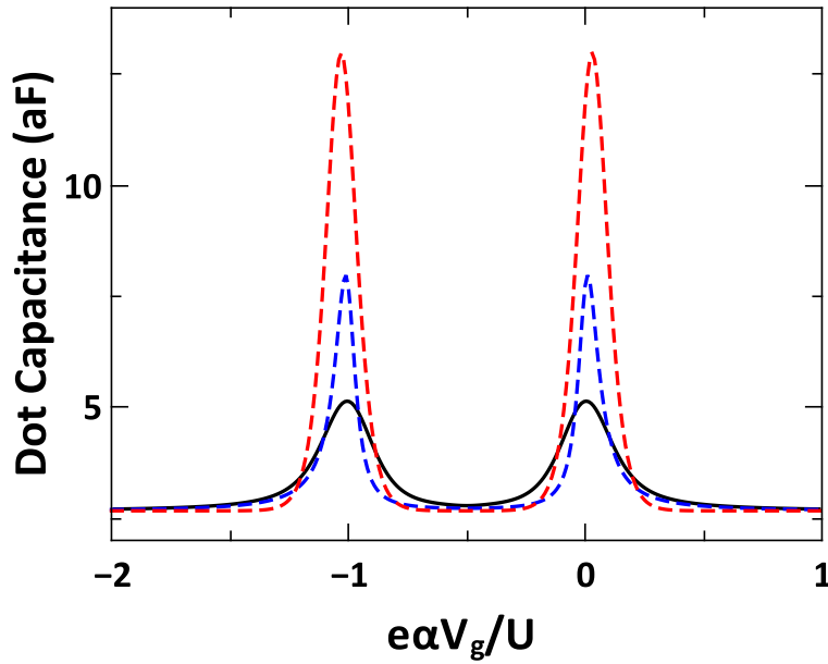
FIGURE 2.7: Mesoscopic capacitance of the QD responding to the AC voltage source in the three different situations addressed in this chapter. Full EOM calculation using numerical evaluation of equation (2.28) (black curve), EOM with Lorentzian approximation at T=0 , using analytical expression (2.34) (blue dashed curve) and sequential tunnelling regime using master equation approach (red dashed curve).
