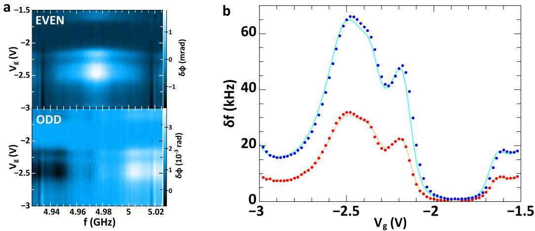
FIGURE 4.11: a : even and odd phase contrast versus gate voltage and frequency on the Kondo of figure 4.2. b : dispersive (blue dots) and dissipative (red dots) frequency shifts extracted from (a). Light blue (resp. light orange) curves corresponds to the differential conductance expressed in units of dispersive (resp. dissipative) frequency shifts.
