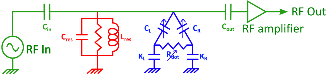
FIGURE 4.7: Equivalent electronic circuit of the QD coupled to a microwave resonator. The QD circuit (blue) is in parallel to the RLC equivalent circuit of the resonator (red). R_{dot} represents the dissipative channel of the SWNT QD (finite conductance) while C_L and C_R represents both geometrical and quantum capacitance from the QD and leads toward the cavity.
