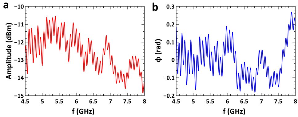
FIGURE 3.11: Calibration of the microwave table. Amplitude ( a ) and phase ( b ) of the RF demodulation setup vs frequency of the local oscillator with P = -87 dBm entering the amplification chain. The output of the up-converter (dashed pink square of figure 3.9) is directly connected to the input of the amplification chain (dashed blue square of figure 3.9).
