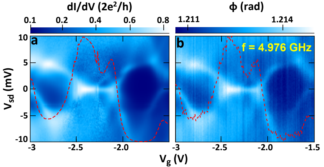
FIGURE 4.2: a : Color scale plot of the differential conductance of the SWNT QD NTRES33bZ4D in units of 2e^2/h in the gate/bias voltages plane. Three Coulomb diamonds are visible and a Kondo ridge at zero bias is observed in the middle diamond. b : Color scale plot of the phase of the microwave field transmitted through the cavity at f = 4.976\text{GHz} taken simultaneously with (a). In both colour scale plot, the dashed red line is a cut at zero bias.
