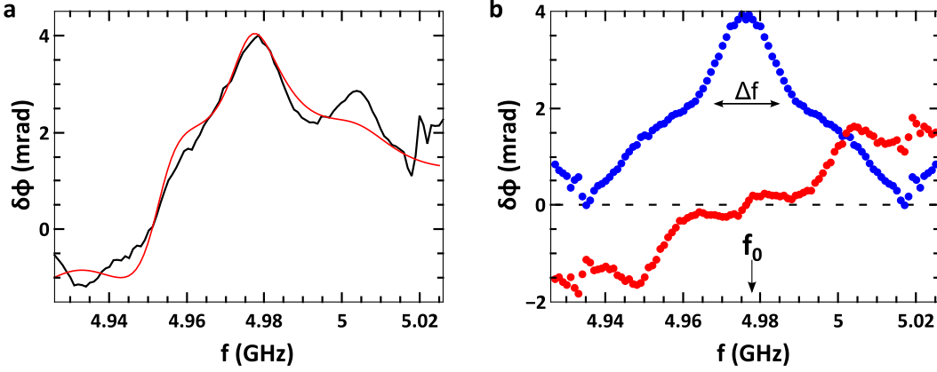
FIGURE 4.9: a : Phase contrast (black curve) along the Kondo ridge of figure 4.2. The phase reference is taken in the empty orbital at V_G = -1.85 V. Red curve, model of a QD coupled to the cavity with Fabry-Perot mode to account for the modulations of the experimental data. b : even (blue curve) and odd (red curve) parts of the phase contrast in (a) in qualitative agreement with 4.8 (b).
