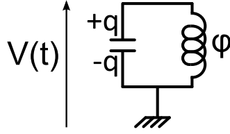
FIGURE 1.16: LC circuit under a voltage V(t) . The useful parameters to describe its behavior are the charge q on the condensator plates and the phase \phi of the inductance.
