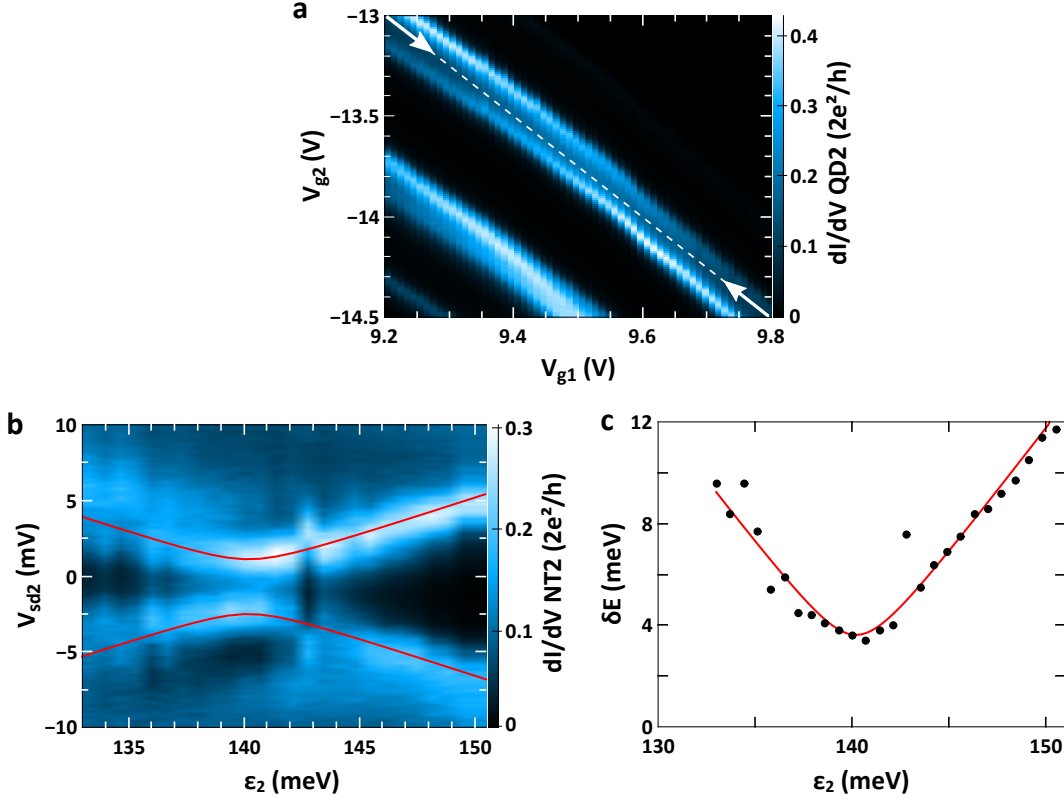
FIGURE 5.7: a : Close-up on one particular region of figure 5.2 where QD2's levels anticross. b : Color scale plot of the energy level splitting along the white dashed line of (a). For every gate voltage V_{g1} , a differential conductance scan in the gate voltage of QD2 V_{g2} bias voltage of QD2 V_{sd2} is taken. The cut in the middle of the corresponding Coulomb diamond is reported in (b). The red curves correspond to equation. c : Energy level separation \Delta E extracted from (b) (black dots) and fit with equation (red curve).
