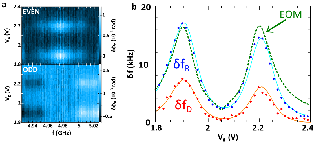
FIGURE 4.10: a : even and odd phase contrast versus gate voltage and frequency in a Coulomb blockade regime. b : dispersive (blue dots) and dissipative (red dots) frequency shifts extracted from (a). Light blue (resp. light orange) curves corresponds to the differential conductance expressed in units of dispersive (resp. dissipative) frequency shifts. The dashed green curve corresponds to a fit with the EOM model of chapter 2.
