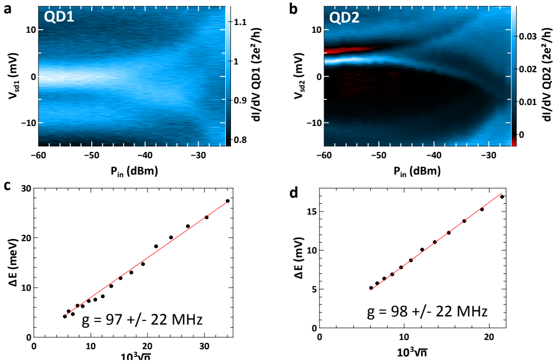
FIGURE 6: Energy level splitting versus power at the input port of the microwave cavity for a Fabry-Perot QD (a) and a Coulomb blockade QD (b). The color code is the differential conductance of the measured QD. c and d : Energy level spacing respectively taken from (a) and (b), plotted versus the square root of the mean number of photons in the cavity. The linear dependence fit of the data (in red) gives the coupling parameter g as its slope.
