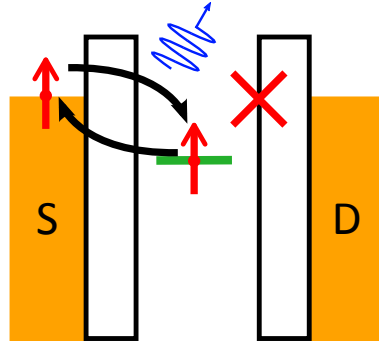
FIGURE 4.4: Scheme of a situation where the QD is contacted to one lead only. Charge fluctuations (represented by black arrows) from the contacted lead to the dot are possible, affecting the cavity field.
