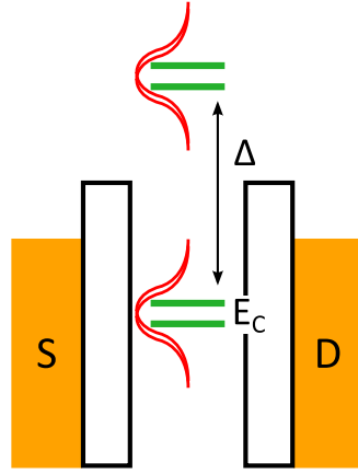
FIGURE 1.3: Scheme of the different energy scales involved the Fabry-Perot regime. Orbitals are separated by the level spacing \Delta . The level broadening \Gamma due to the coupling of the QD to the leads is much larger than the charging energy and temperature.
