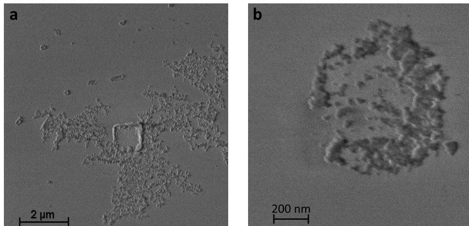
FIGURE 3.2: Catalyst deposition with (a) one layer of PMMA (500nm thickness) and (b) two layers of PMMA ( 1\mu\text{m} thickness). Catalyst spread away from the lithographed hole in the case of one layer of PMMA on an area up to 10\mu\text{m}\times\mu\text{m} .
