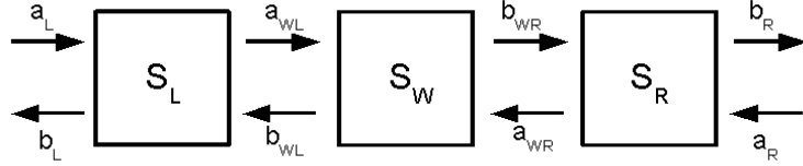
FIGURE A.1: Model of the system representing left (L) and right (R) contacts connected by a wire (W) being the nanotube.
