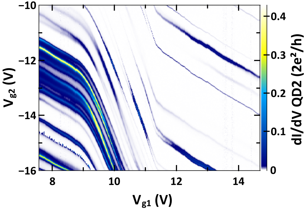
FIGURE 5.2: Color scale plot in the gate voltage of QD1 V_{g1} gate voltage of QD2 V_{g2} of the differential conductance of QD2. The energy levels of QD2 exhibits a strong dependence versus V_{g1} , showing anticrossings and crossings.
