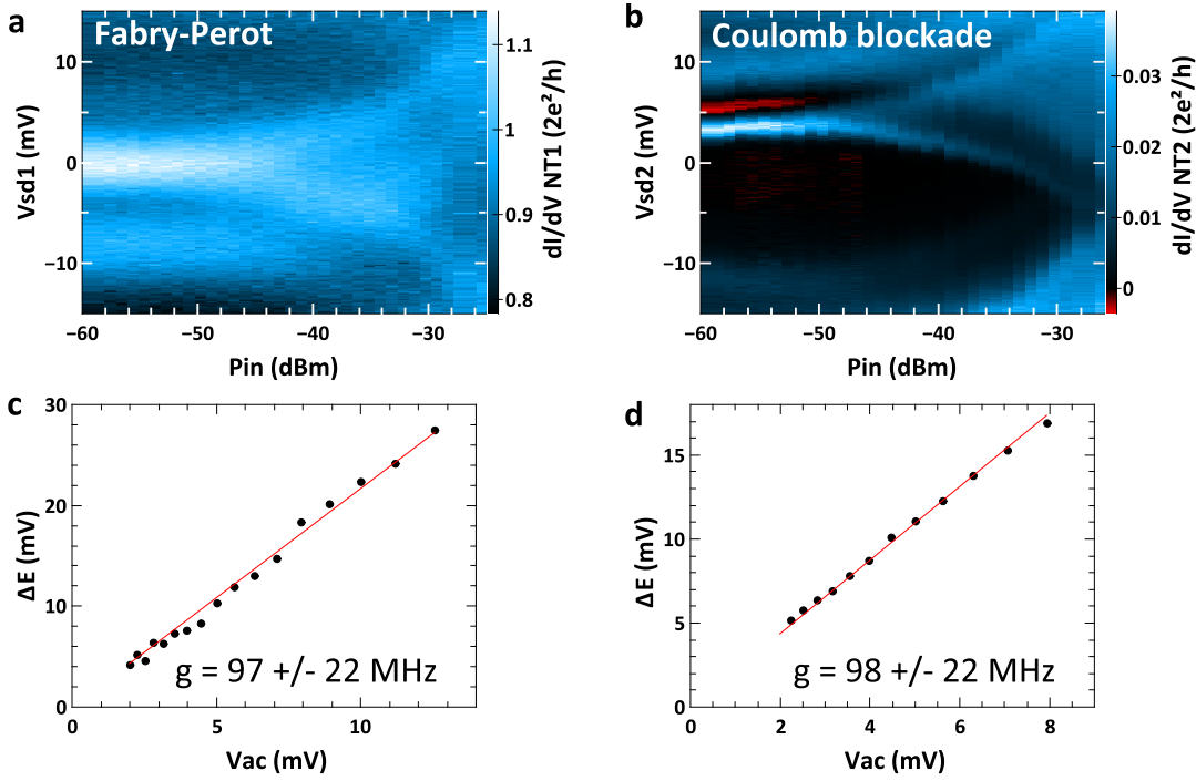
FIGURE 4.13: Energy level in bias voltage V_{sd} splitting versus RF power input P_{in} , in the case of Fabry-Perot (a) and Coulomb blockade (b) of figure 4.1. c and d, extracted energy level separation of respectively (a) and (d) versus V_{AC} . The linear dependence is directly related to the coupling g between the QD and the cavity.
