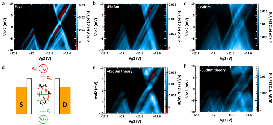
FIGURE 4.12: Evolution of a Coulomb diamond with increasing power at the input port of the microwave cavity. Input power is Off in a , -45dBm in b and -35dBm in c . d : scheme of the capacitive coupling action of the microwave field on the electronic level of the QD. The electronic level oscillates around its position without EM field E_0 with an amplitude \lambda . The averaging of this oscillation gives rise to two splitted levels at positions E_0 \pm \lambda . e and f : simulations of the averaged oscillation of the electronic level respectively for -45dBm and -35dBm.
