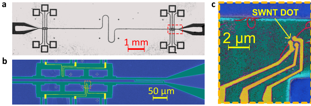
FIGURE 4: a : photograph of a CPW resonator in Nb/Pt or Al. b : optical micrograph close up in false colors of the ground plane openings where the SWNT QDs are contacted. The superconductor is in blue and the dielectric in green. c : SEM micrograph in false colors of the contacted QD with source, drain and gate electrodes. The blue represent the superconductor (transmission line and ground plane), the yellow is for the Pd electrodes, the SWNT is in red and the dielectric in green.
