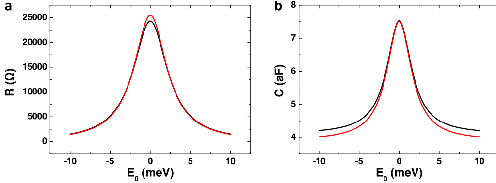
FIGURE 2.4: Simulation of the value of resistances R_L (black) and R_R (red) (a) and capacitances C_L (black) and C_R (red) (b), as defined in figure ?? in appendix ?? section ?? . C_L=2.1\text{aF} , C_R=2\text{aF} , C_G=3.9\text{aF} , \Gamma=1\text{meV} and E_0 ranges from -10\text{meV} to 10\text{meV} .
