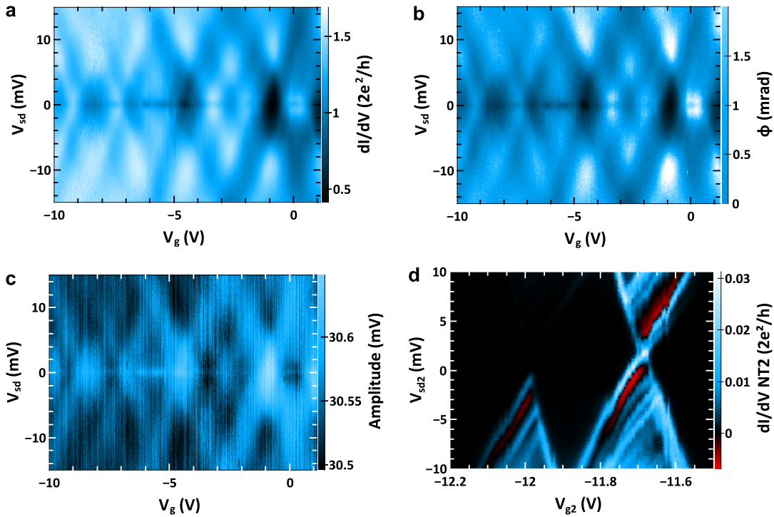
FIGURE 4.1: a : Color scale plot of the differential conductance of the SWNT QD NTRES2aZ7D in units of 2e^2/h in the gate/bias voltages plane in the Fabry-Perot regime. b(c) : Colour scale plot of the phase (amplitude) of the microwave field transmitted through the cavity at f = 5.75\text{GHz} taken simultaneously with (a). d : Color scale plot of the differential conductance of the SWNT QD NTRES2aZ6G in units of 2e^2/h in the gate/bias voltages plane in the Coulomb blockade regime. Excited states are visible as well as negative differential conductance peaks in red.
