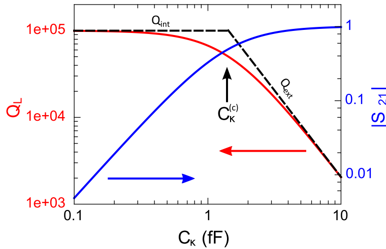
FIGURE 1.15: Loaded quality factor Q_L (red) and transmission amplitude |S_{21}| (blue) of the coupled resonator of internal quality factor Q_{int} = 10^5 versus the coupling capacitance C_\kappa . The loaded quality factor and the transmission amplitudes undergo an opposite variation versus C_\kappa giving rise to a critical coupling value C_\kappa^{(c)} .
