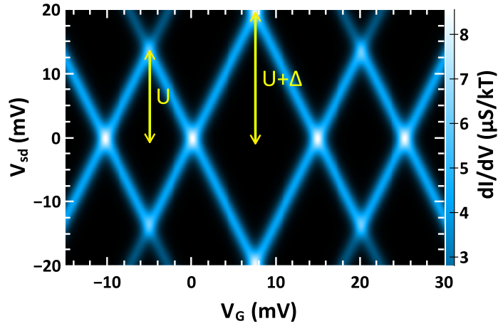
FIGURE 1.8: two levels QD with double occupancy differential conductance (b) in the gate/bias voltages plane. \Delta = 5\text{ meV} , U = 10\text{ meV} , \gamma = 100\mu\text{eV} and T = 5\text{ K} .
