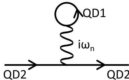
FIGURE 5.3: Diagrammatic representation of the distant interaction between QD1 and QD2 without photon renormalization. The plain lines with arrows refers to electronic propagators of QDs. The whirly line refers to photon propagator at frequency i\omega_n .
