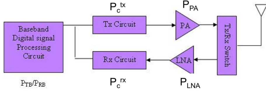
FIGURE 2.12: RF components of CC2420 chip
