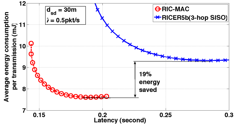
FIGURE 4.11: Energy consumption with real MAC protocol (PowWow platform) in high traffic load networks
