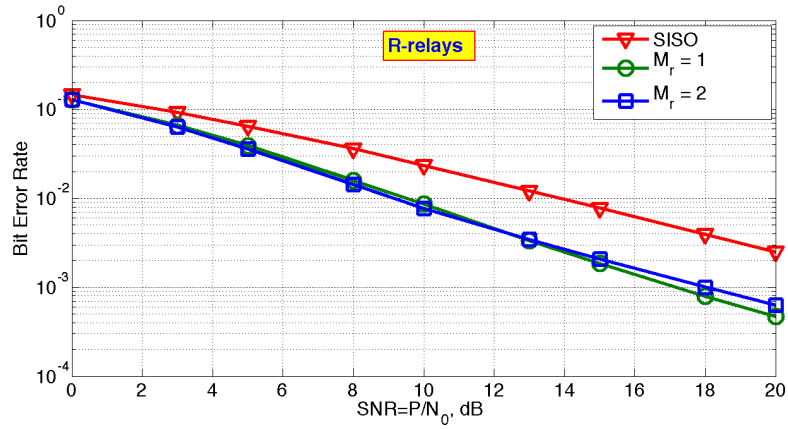
(b) R-relays
