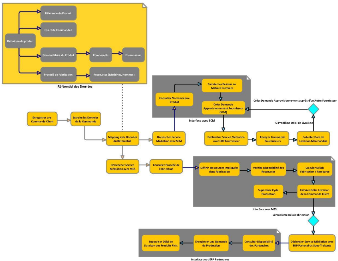
Figure 5.2. Exemple de Services Industriels
