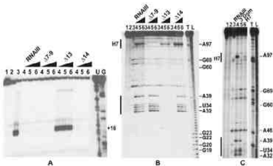
Figure 3. The RNAIII- coa mRNA complex prevents ribosome binding and promotes RNase III cleavages. (A) Formation of the ternary complex between coa mRNA (15 nM), 2.5-merit 30S ribosomal subunits (250 nM), and initiator tRNA (1 \mu M) was monitored in the absence (lane 1) or in the presence of increasing concentrations of wild-type RNAIII, RNAIII- \Delta 7-9 ( \Delta 7-9), RNAIII- \Delta 13 ( \Delta 13), and RNAIII- \Delta 14 ( \Delta 14): lane 4, 25 nM; lane 5, 50 nM; lane 6, 100 nM. The toeprint at position +16 is indicated. Lanes 1, 2: incubation controls on free RNA or RNA bound to RNAIII, respectively. Lanes U, G: dideoxy-sequencing reactions performed on coa mRNA. (B) RNase III hydrolysis of 5'-end-labeled coa mRNA, alone (lane 1) or in the presence of an excess of wild type RNAIII, RNAIII- \Delta 7-9 ( \Delta 7-9), RNAIII- \Delta 13 ( \Delta 13), RNAIII- \Delta 14 ( \Delta 14): lane 4, 25 nM; lane 5, 50 nM; lane 6, 100 nM. Lanes 1, 2: incubation controls on free coa mRNA or bound to RNAIII, respectively. Lanes T1, L: RNase T1 and alkaline ladders, respectively. (C) RNase III hydrolysis of 5'-end-labeled coa mRNA, alone (lane 1) or in the presence of an excess of wild type RNAIII (lane 4), the 3' domain of RNAIII (3' Dom), and the hairpin 7 of RNAIII (H7). Lanes T1, L: RNase T1 and alkaline ladders, respectively. doi:10.1371/journal.ppat.1000809.g005
