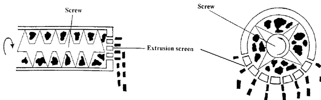
Fig. I.8: Schematic view of axial and radial type of screw extruder (adapted from Vervaeet et al., 1995)
