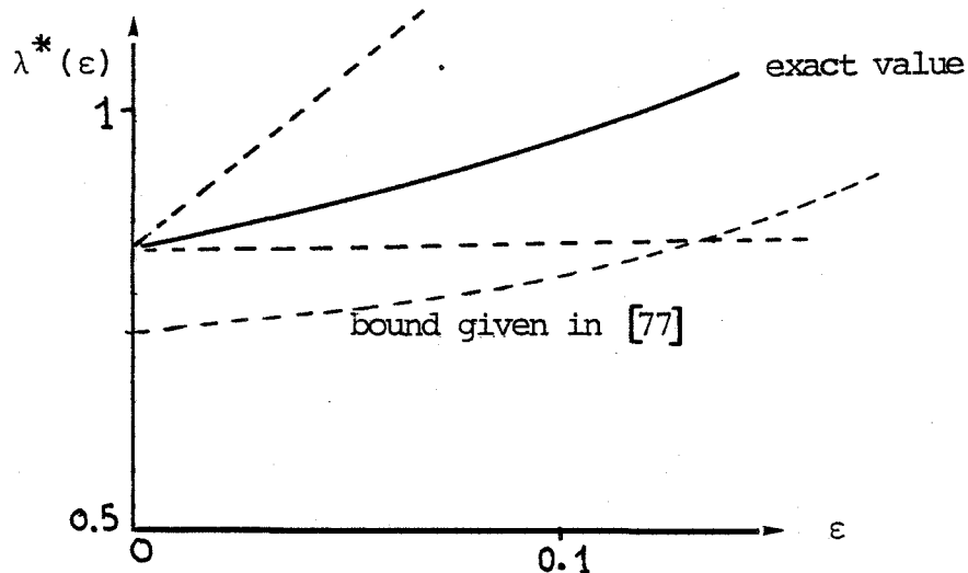
Fig.6 : comparison of the exact \lambda^*(\varepsilon) and asymptotic bounds given by (5-4).
