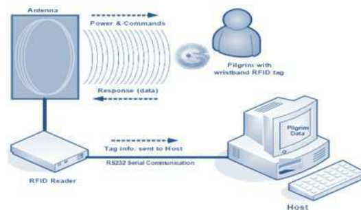
FIGURE 3.31 – RFID System for pilgrim identification
