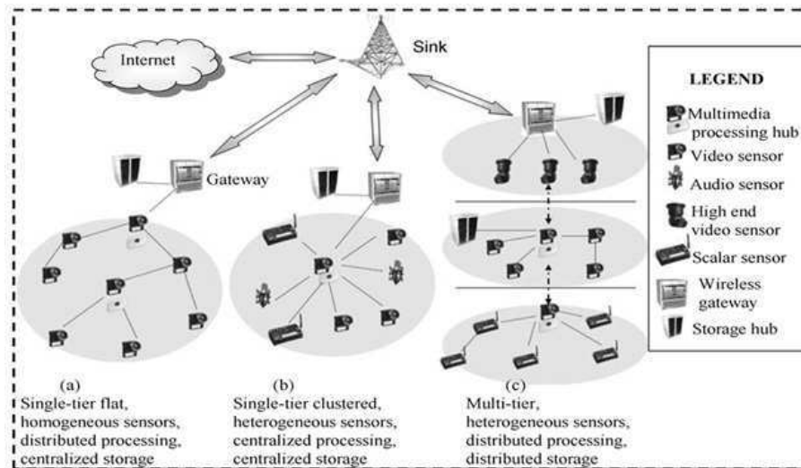
FIGURE 2.6 – WMSN Architecture
