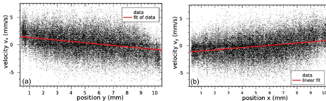
Figure 7.3: The fit (red) of the v_{x,y} vs y,x distribution. The black points are the particle positions. The picture is taken from ref. [MY1].
