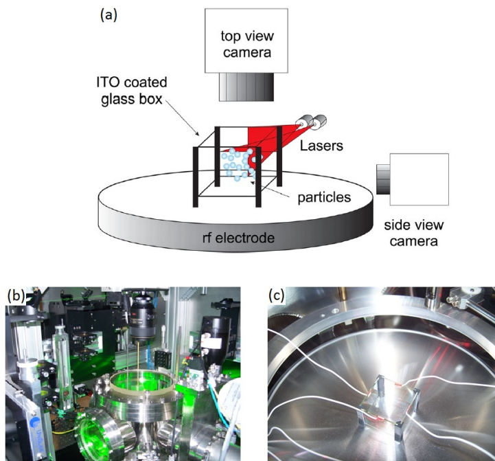
Figure 7.1: Sketch of the GEC setup with the glass box and the illumination system (a), ref. [MY1]. Picture of the chamber illuminated by the strong green laser (b) and the glass box mounted on the electrode (c). Both pictures are courtesy of V. Nosenko.
