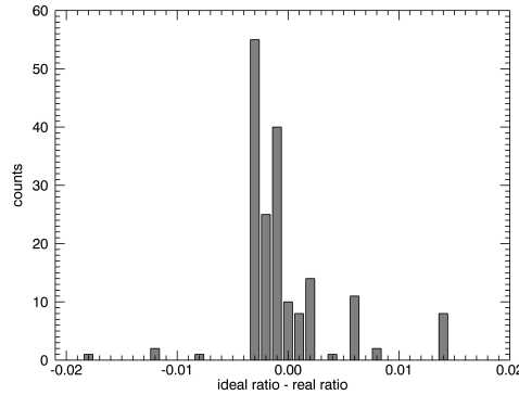
Figure A.4: Limitation to the synchronization as calculated from sequences recorded at 50 Hz. The ideal ratio of the phase set frequency to the camera frame rate minus the real ratio is displayed. The absolute mean difference between the two equals 0.00604.
