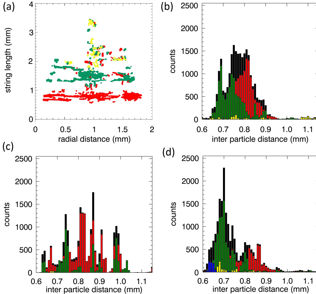
Figure 8.12: String length and in-string inter-particle distance. Distribution of the length of the strings vs. radial (XY-projected) distance to the CMS, shown for the clockwise rotating cluster (a). Two main effects can be seen immediately: (i) the discreteness of the string length distribution is well pronounced and (ii) surprisingly, the longer strings are located dominantly not in the middle of the cluster. (b, c, d) Histograms of the in-string inter particle distance \Delta l_{part} computed for: (b) the cw-rotating cluster, 5 kHz driving ac-field [same as in (a)], (c) non-rotating cluster, 1 kHz driving ac-field, (d) ccw-rotation, 5 kHz driving ac-field. Note that statistically the triplets are relatively more compact 'constructed' than the doublets, for all cases \langle \Delta l_{part}^{doublet} \rangle > \langle \Delta l_{part}^{triplet} \rangle . For longer strings the statistics is poor. Color coding: (black) all events, (red) doublets, (green) triplets, (yellow) quartets, (blue) quintets, and (orange) sextets
