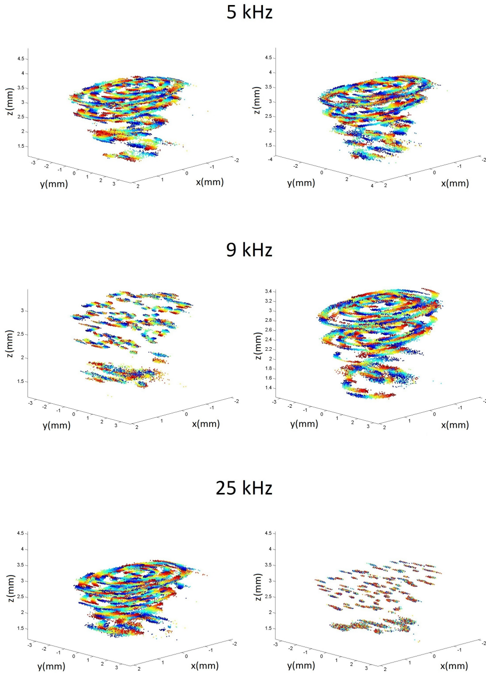
Figure 8.4: Shell rotation as seen in a cluster for different excitation electric field frequencies (Right hand side: clockwise rotation, left hand side: counter clockwise rotation). The time is displayed by the color coding. Early particle positions are given by blue, later by red colors.
