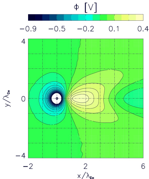
Figure 2.5: Wake field as it forms downstream a particle situated at (0,0) . In this plot the ions stream from the left to the right. Downstream the negatively charged particle a positive potential forms. This is the so-called wake field which attracts other negatively charged particles and is responsible for string formation, [151].
