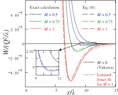
Figure 2.7: Isotropic interaction potential for different Mach numbers [109].
