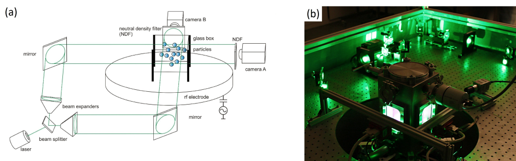
Figure 8.1: Picture (b) and sketch (a) of the chamber and the illuminations system as mounted in Kiel. The green illumination laser is in operation. In front the chamber surrounded by the two cameras can be seen. In the back the illumination system is mounted. The picture is courtesy of J. Schablinski.
