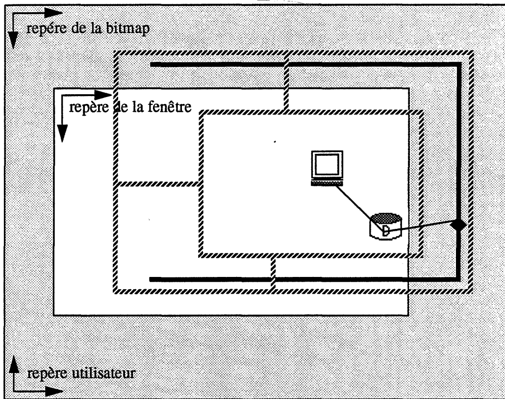
Figure 61: Les Bitmaps
