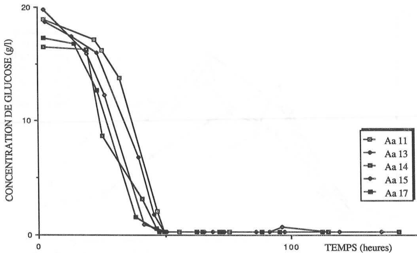
FIGURE IV.12 : GLUCOSE RESIDUEL DOSE.
