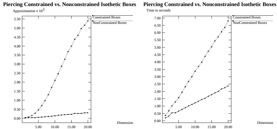
FIG. 2.5 – Impact of the dimension over a set \mathcal{S} ( c^*(\mathcal{S}) = 20 and |\mathcal{S}| = 20000 ) of constrained/nonconstrained d -boxes for 1 \leq d \leq 20 . The right chart exhibits the running time of our implementation (the slope of the lines for the constrained/nonconstrained cases are O(d + \log c^*) and O(d \log c^*) respectively).
