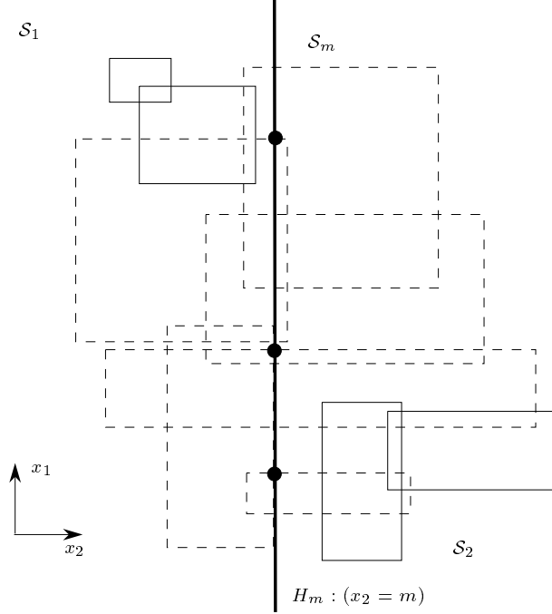
FIG. 2.1 – Partition of \mathcal{S} into three subsets depending on their location with respect to the hyperplane H_m : (x_d = m) . We denote by \mathcal{S}'_m the set of (d-1) -dimensional boxes \mathcal{S}_m \cap H_m .
