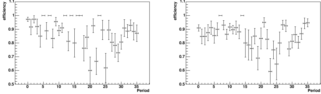
Figure 4.3: Trigger efficiency of one prong taus (left) and three prong taus (right), measured with the calibration electron sample, as a function of the run periods from very beginning of Run II until the end.
