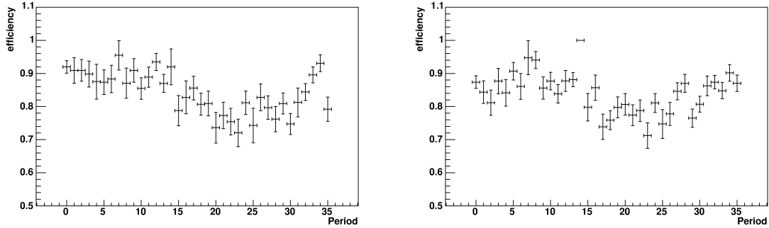
Figure 4.4: Trigger efficiency of one prong taus (left) and three prong taus (right), measured with the high- p_T electron sample, as a function of the run periods from very beginning of Run II until the end.
