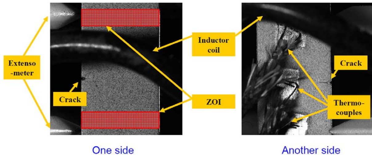
Fig. 4.6 Central part of the specimen for fracture test in the set-up, left one is one side of the specimen, right one is another side
