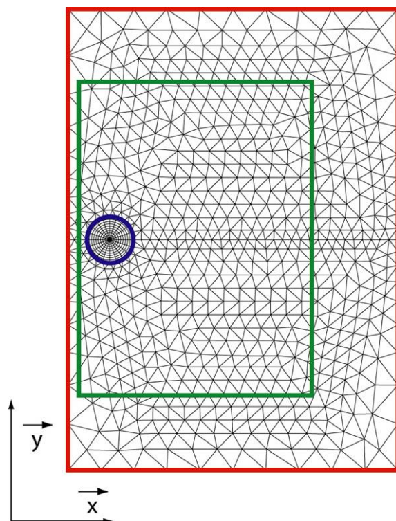
Fig. 3.13 Verification of path independent of J_{IC} obtained by modified G-theta method
