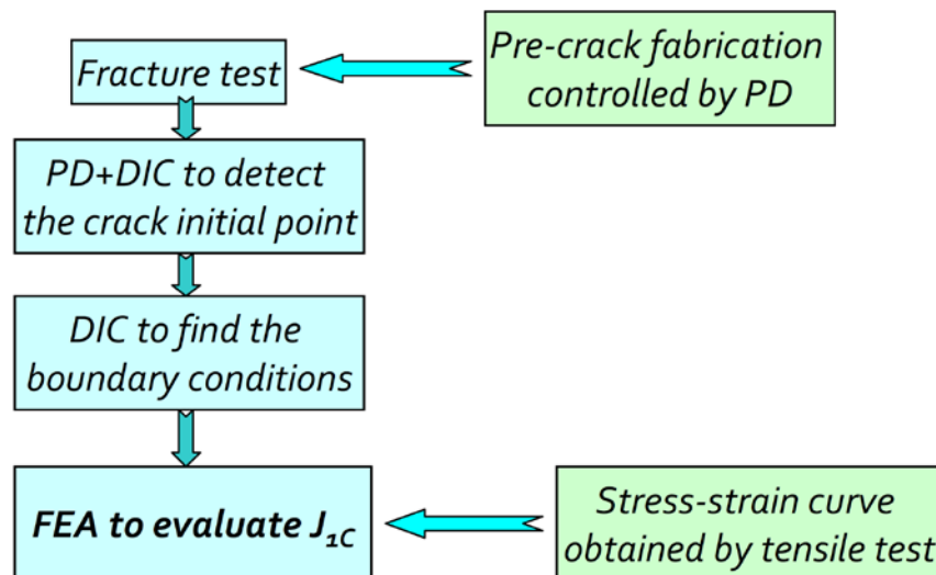
Fig. 1.3 Methodology to get J_{IC} from experiments
