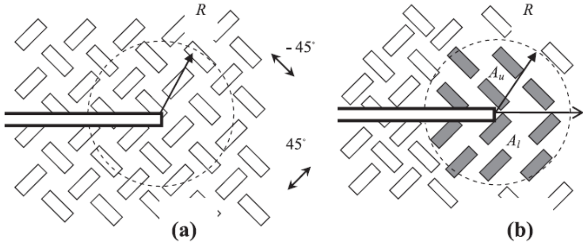
Fig. 2.33 Schematic demonstration of the toughening mechanism due to 90° ferroelastic domain switching near a crack tip: (a) Pre-switching; (b) Post-switching (in dashed circle) [105]
