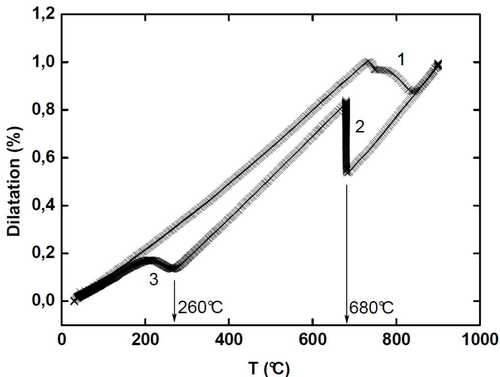
Fig. 5.5 Free dilatation curves of 16MND5 at the isothermal temperature 680^{\circ}\text{C} and then cooling to room temperature by -5^{\circ}\text{C}/\text{s}
