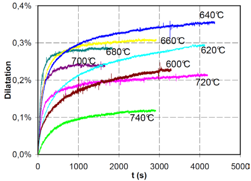
Fig. 5.9 Free dilatation curves of the isothermal transformation before CCT Bc
