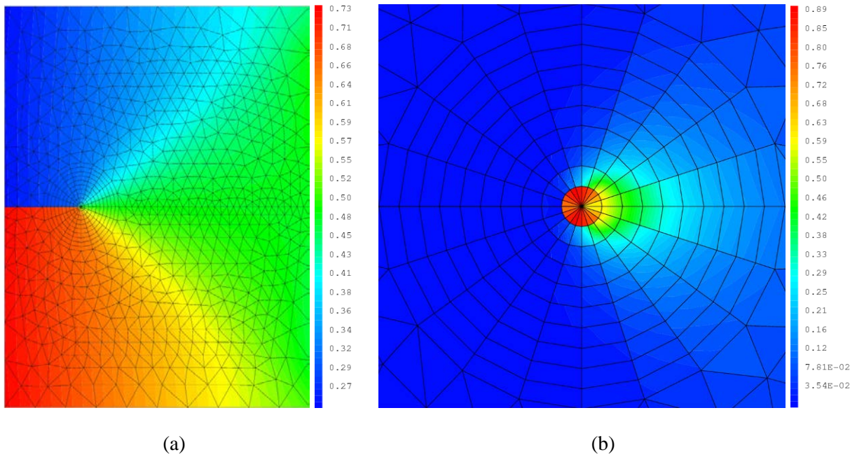
Fig. 3.10 Simulation result, (a) is U_y displacement field (unit: mm), (b) is the accumulated plastic strain around crack tip
