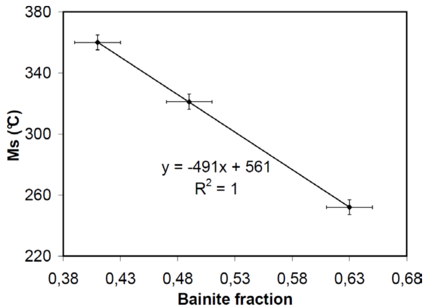
Fig. 5.18 Ms temperature decrease linearly with more bainite fraction produced (Error of T is +/- 5°C and error of fraction is +/- 0.02)
