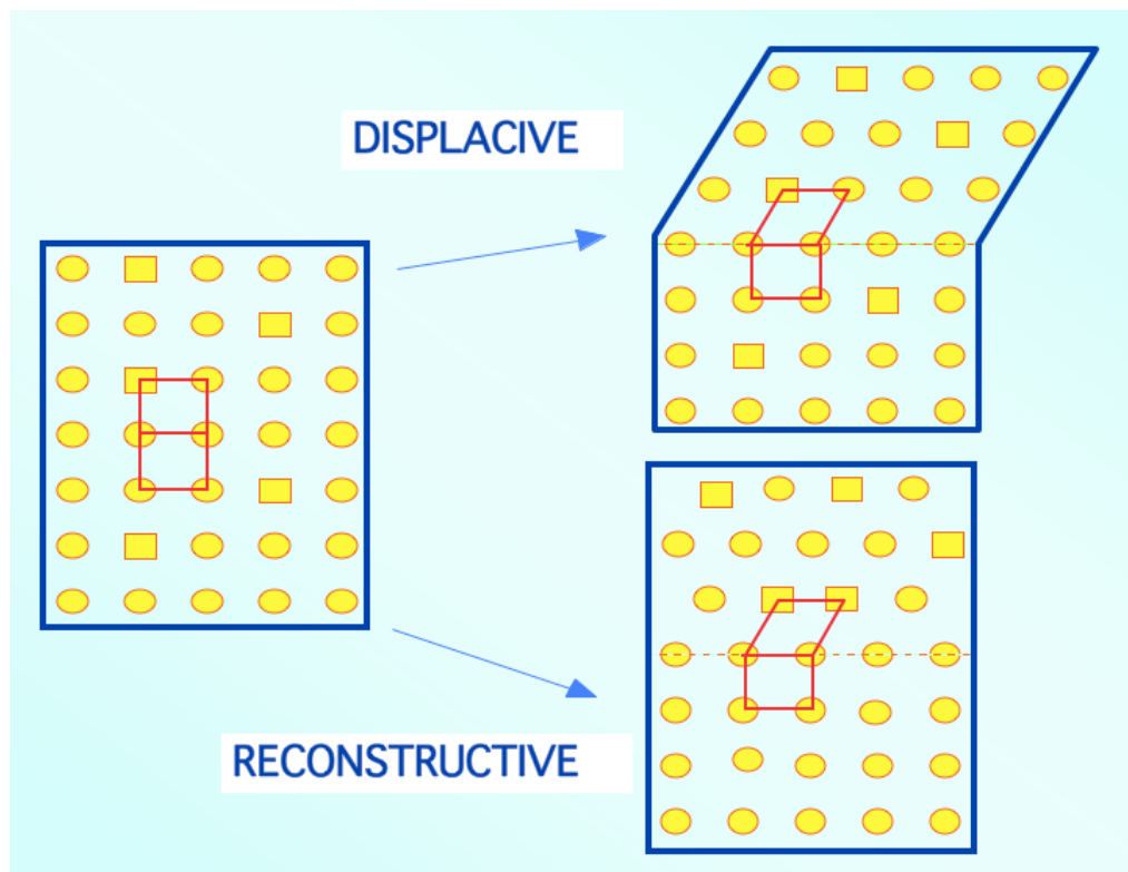
Fig. 2.10 The displacive and reconstructive mechanisms [34]
