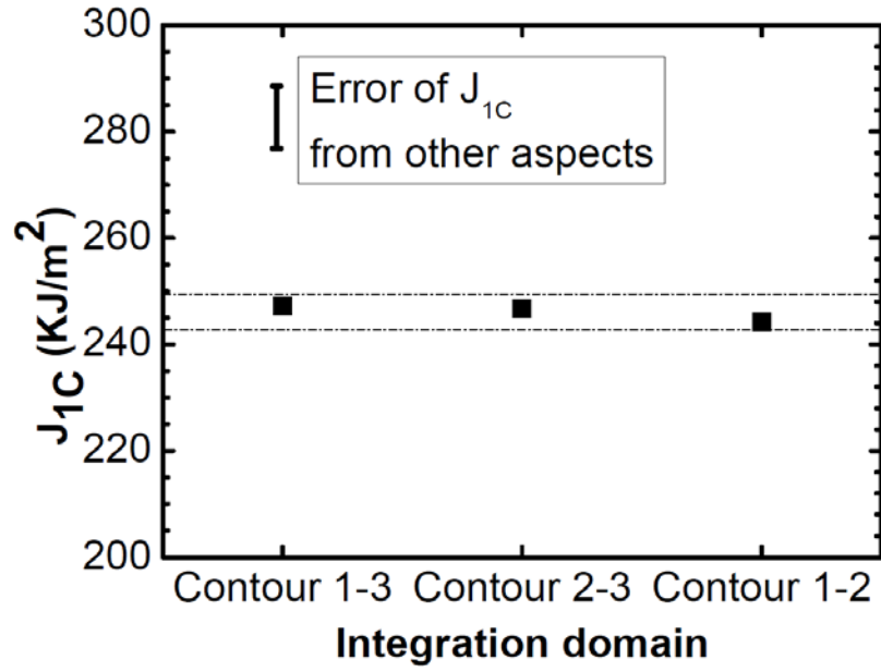
Fig. 3.15 J_{1C} obtained by modified G-theta method for plastic situation (Material: as received 16MND5 low carbon steel)
