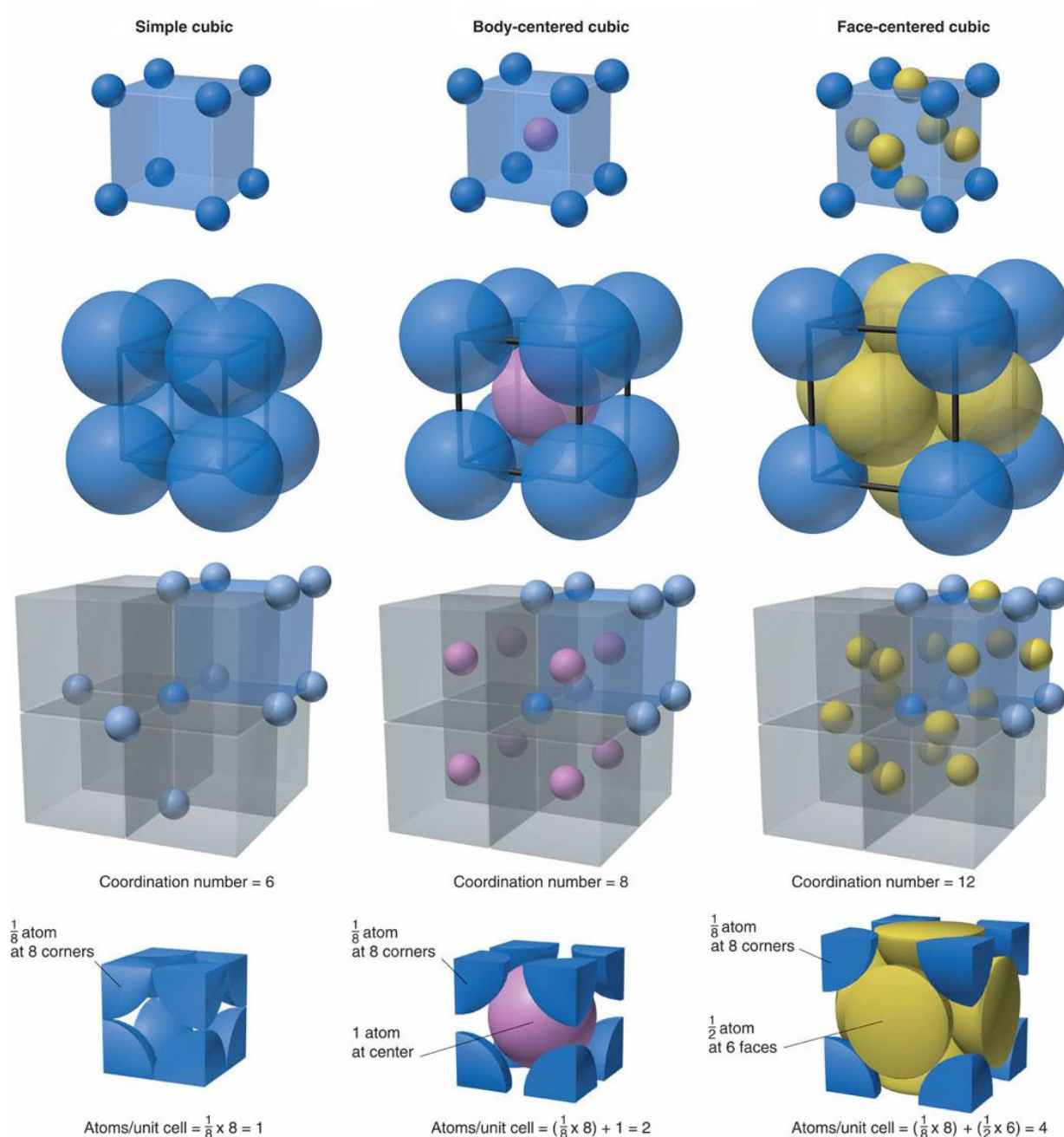
Fig. 2.7 Crystal lattice form [29]
