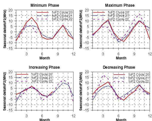
Fig. 4. Seasonal variation of the critical frequency \Delta foF2 , after elimination of the solar influences ( Rz ), during the various phases of the sunspot cycles: minimum phase (top left panel), increasing phase (bottom left panel), maximum phase (top right panel) and decreasing phase (bottom right panel). The red curves correspond to sunspot cycle 20, the dashed blue curves to sunspot cycle 21 and the violet curves to sunspot cycle 22.
