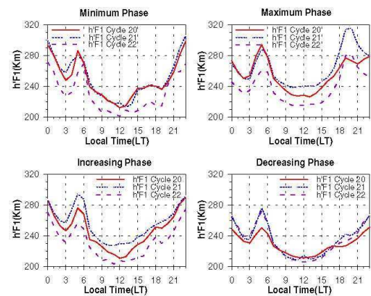
Fig. 11. Similar to Fig. 8 for h'F1 .
