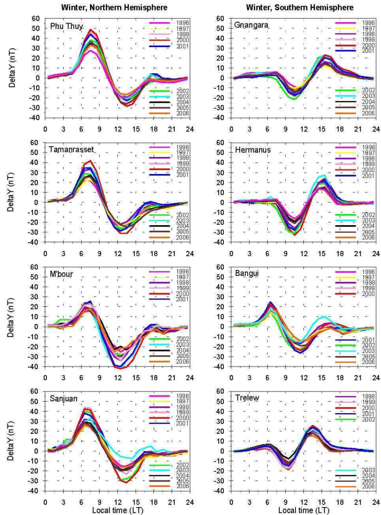
Fig. 12. Similar to Fig. 11 for winter.
