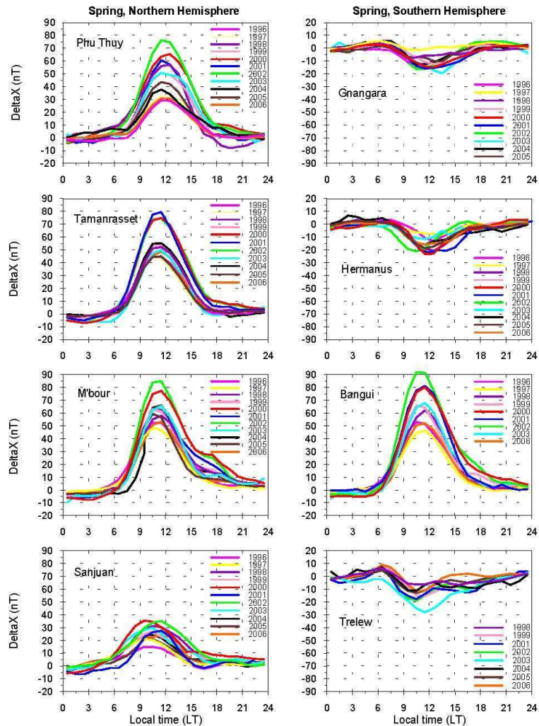
Fig. 10. Seasonal mean diurnal variations of the X component during Spring at Phu Thuy, Gnangara, Tamanrasset, Hermanus, M'Bour, Bangui, San Juan and Trelew from 1996 to 2006 and during quiet magnetic time a_m < 20 nT.
