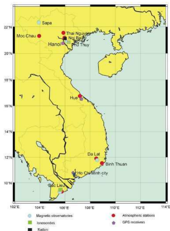
Fig. 2. Map of the Vietnamese network: Ionosondes (green square), GPS receivers (violet pentagon), Magnetometers (blue circles) and Atmospheric stations (red circles).
