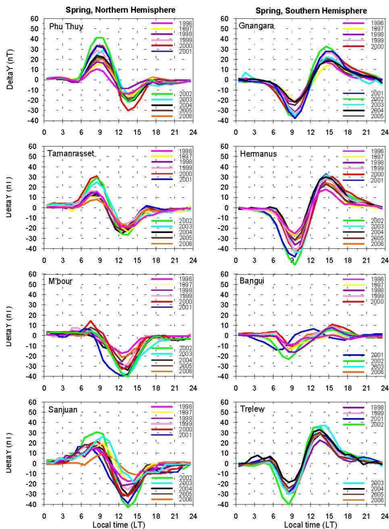
Fig. 11. Seasonal mean diurnal variations of the Y-component during Spring at Phu Thuy, Gngara, Tamanrasset, Hermanus, M'Bour, Bangui, San Juan and Trelew from 1996 to 2006 and during quiet magnetic time am < 20 nT.
