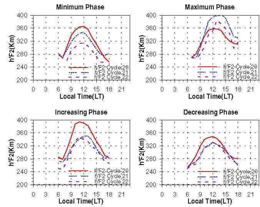
Fig. 10. Similar to Fig. 8 for h'F2 .
