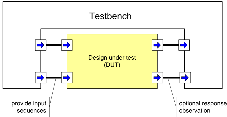
Figure 8.1: Generic Structure of Design Verification.
