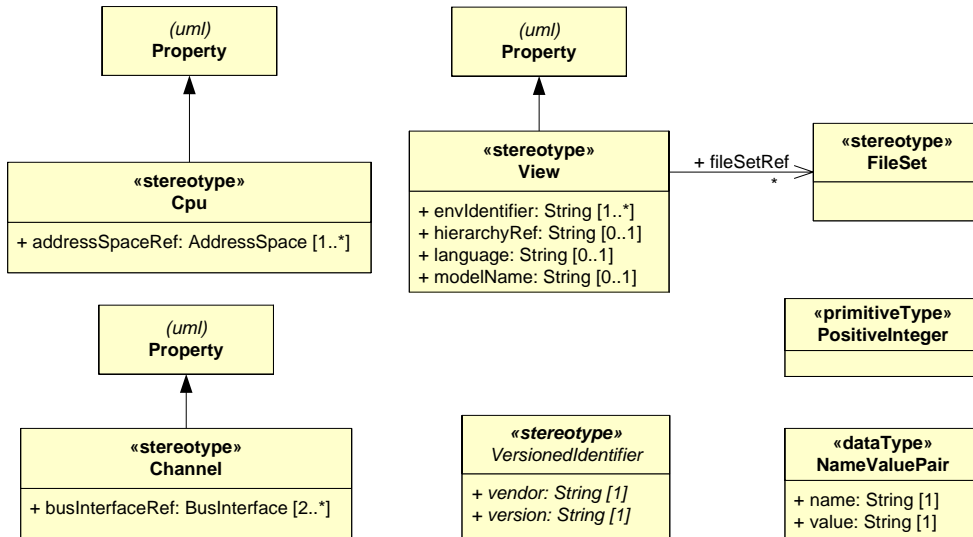
Figure 6.1: VLVN and IP-Xact Component element stereotypes
