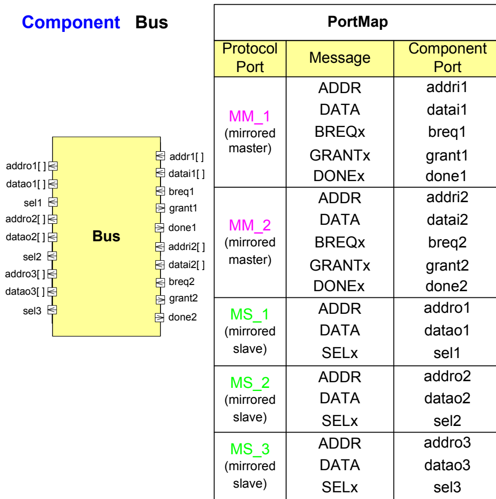
Figure 4.12: Component 'Bus'.
