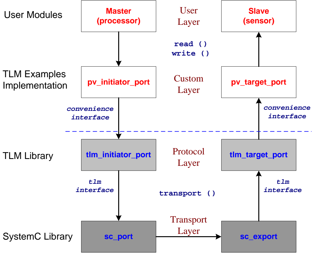
Figure 4.14: Abstract Modeling using TLM Library
