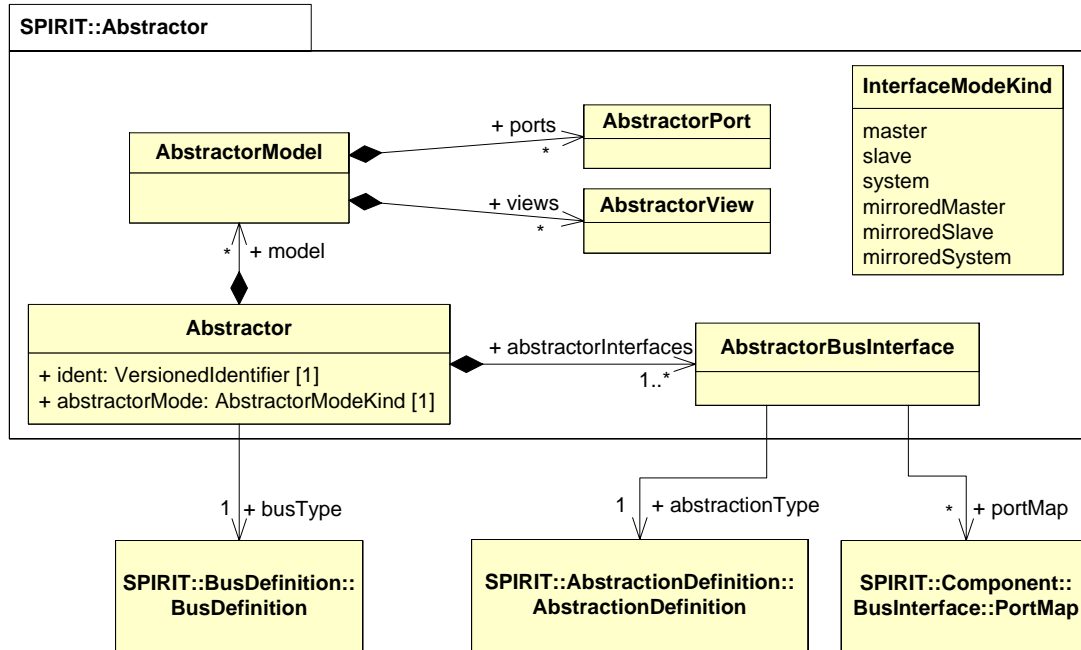
Figure 5.16: IP-Xact Abtractor Metamodel.
