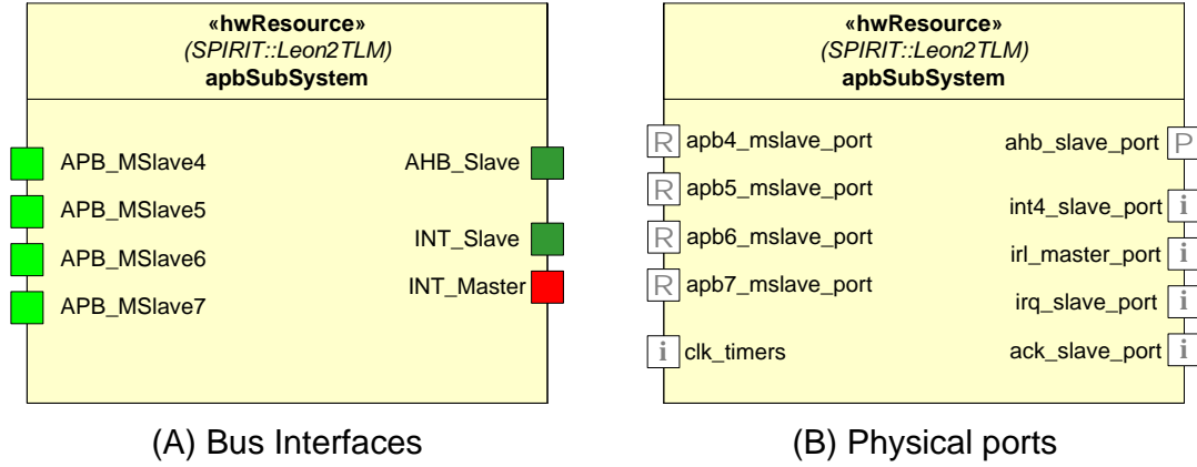
Figure 6.15: AMBA AHB Bus Component in UML.
