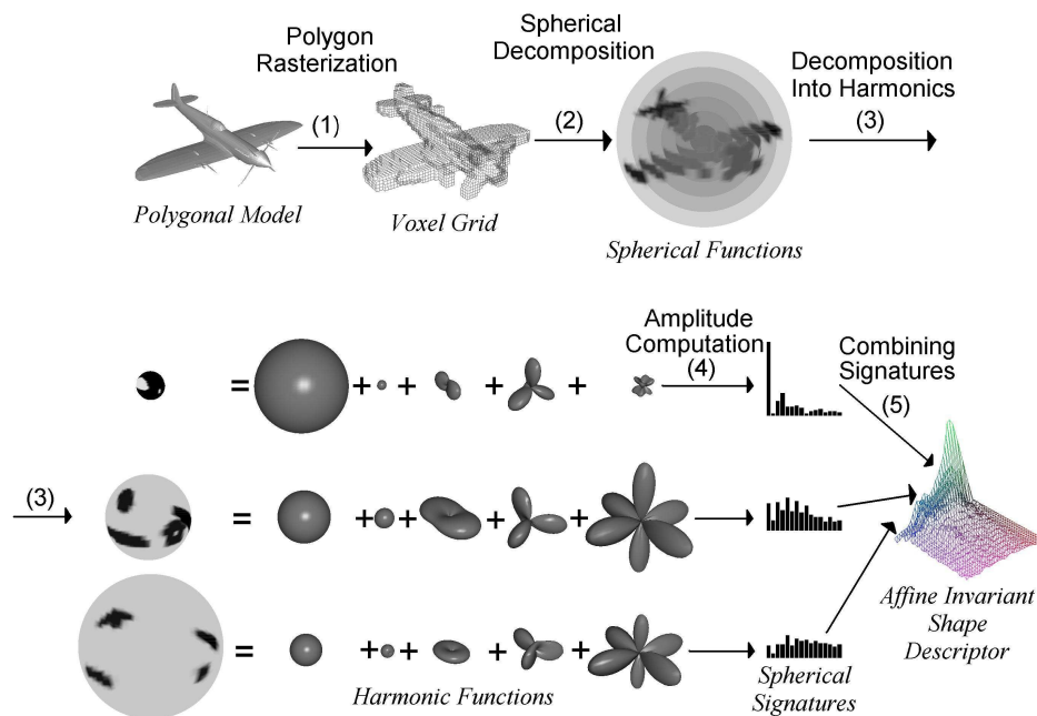
Figure 2.8 – Computing the Harmonic Shape Representation. (Figure taken from Kazhdan and Funkhouser 2002 ACM Press (52)).
