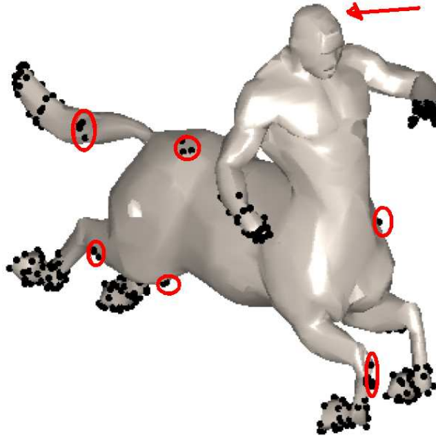
Figure 3.3 – Feature point detected based on the heat kernel. To our concept, feature point detected other than those located on the extremities are undesirable feature points. Also, the method introduced by Bronstein et al.(11) missed to detect feature point located on the top of the head of the centaur. (Figure taken from Bronstein et al.(11))
