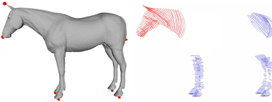
Figure 2.7 – Representation of patches by an indexed collection of curves.
