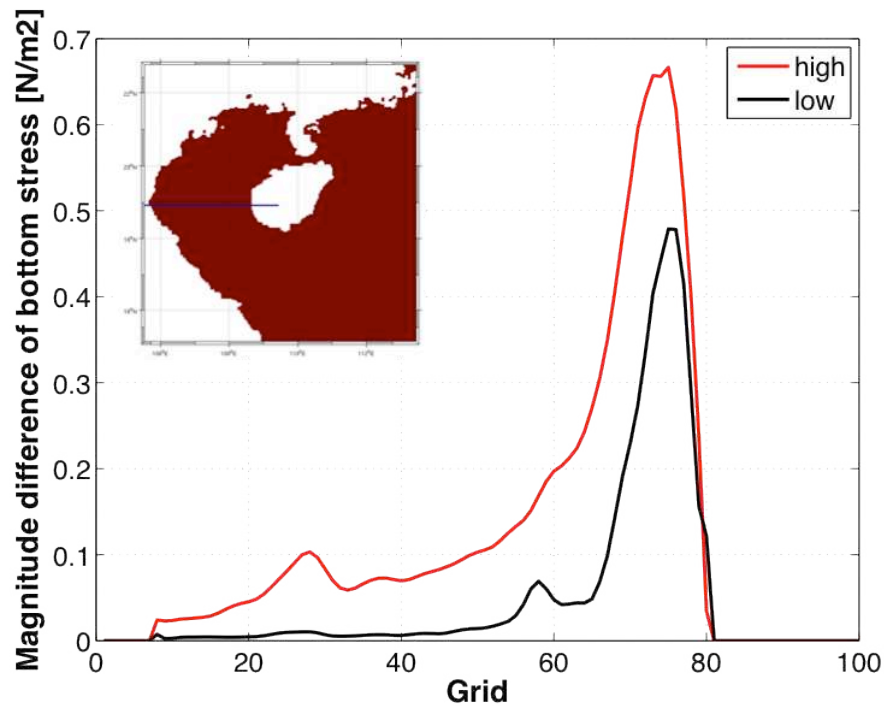
Figure 3.15: Cross section along latitude 18.9°N of bottom frictional stress difference [N/m 2 ] between 3D simulation using logarithmic drag formulation via bottom roughness z_0=0.1 mm and 3D simulation using quadratic drag law with C_D=0.001 . The position of cross section is indicated in the inset panel.
