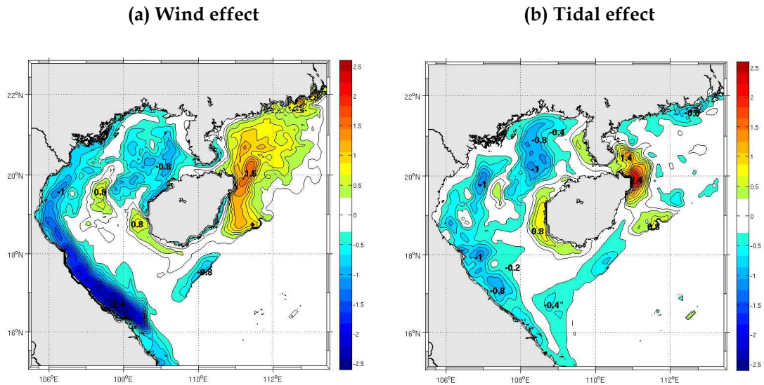
Figure 6.3: (a) February SST difference [°C] between EXP3 and EXP1 (with and without wind forcing); (b) between EXP2 and EXP1 (with and without tides forcing); contour interval 0.2 degree. The oceanic zone deeper than 200 m is not shown.
