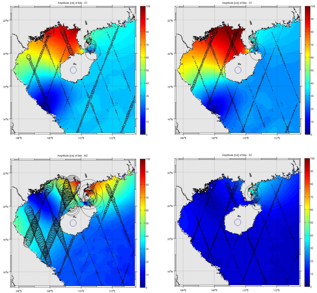
Figure 3.9 -1 st part- Tidal misfits in the Gulf of Tonkin for K1, O1, M2, and S2 constituents: background charts represent the model tidal amplitude in centimeter. The size of black circles is proportional to the RMS error of amplitude between ROMS solution and altimeter data. Reference: 10 cm.
