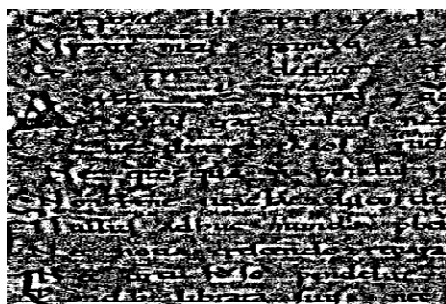
(Niblack, [1986])
