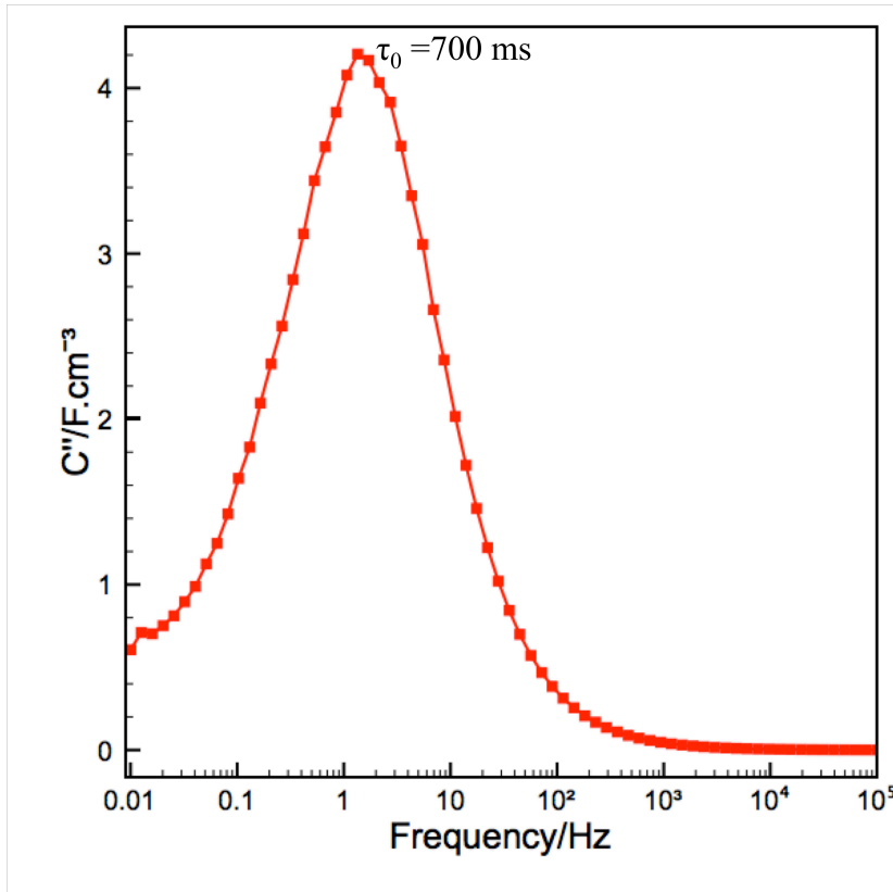
Figure II.13 Evolution of the imaginary part of the stack capacitance of the AC based micro-supercapacitor in 1M \text{NEt}_4\text{BF}_4/\text{PC} electrolyte.
