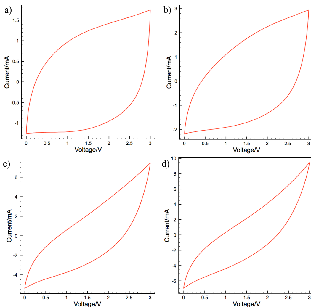
Figure II.14 CV plots of AC based micro-supercapacitor in 1M \text{NEt}_4\text{BF}_4/\text{PC} a) at 500 mV/s, b) at 1 V/s, c) at 5 V/s and d) at 10 V/s within 3V.
