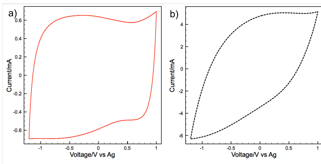
Figure II.8 The CV results of the samples with a) 5s and b) 60s of deposition at 100 mV/s within 2.2 V in 1M \text{NEt}_4\text{BF}_4 in PC.
