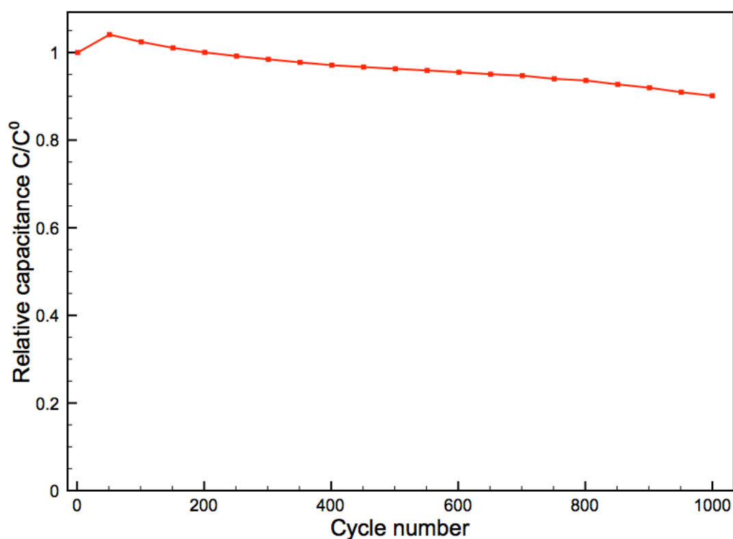
Figure II.31 Cycling test results of OLC based micro-supercapacitor in ILM at 1 V/s.
