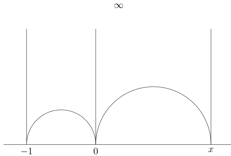
Figure 1.5: The cross-ratio
