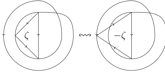
Figure 4.1: Effects of a switch. S^1 is seen as the double cover of \mathbb{P}^1 and so visualized as a circle running twice around the unit circle.
