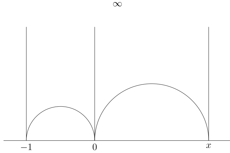
Figure 1.5: The cross-ratio
