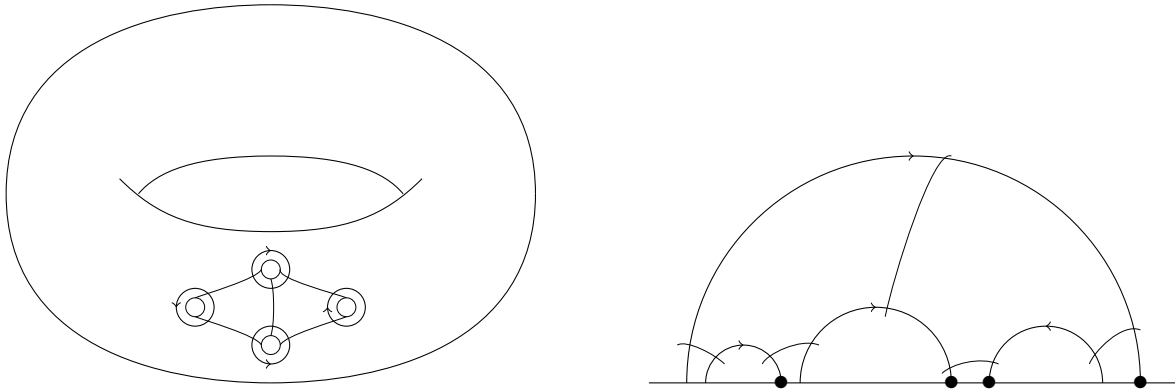
Figure 1.4: Lifting of the triangulation
