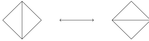
Figure 1.2: A flip.
