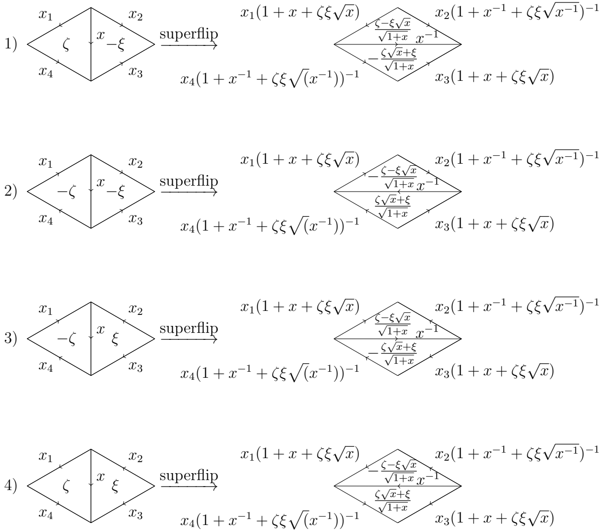
Figure 5.1: Superflips
