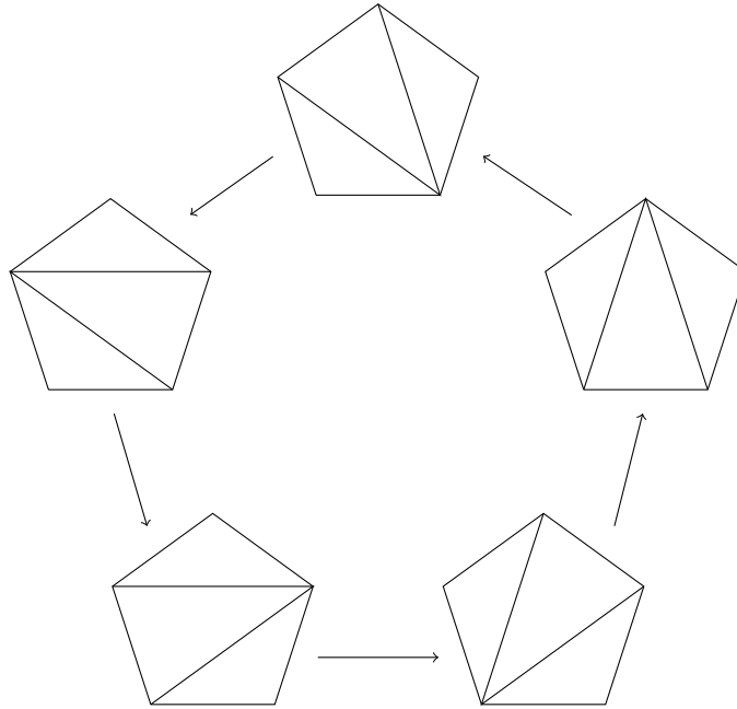
Figure 1.3: Pentagon relation
