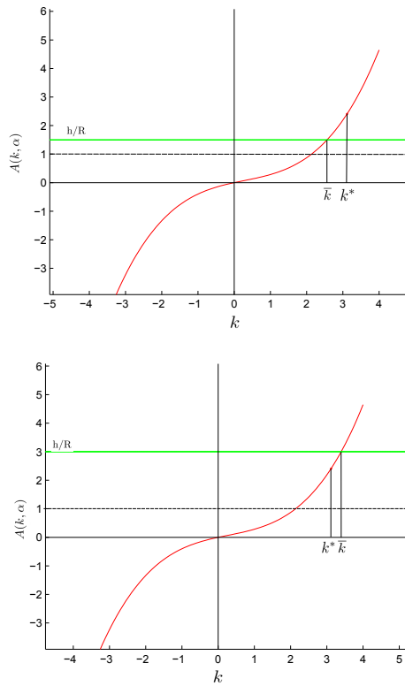
Figure 5.19: Behaviour of A(k, \alpha) for \alpha = \frac{2}{5}\pi and R = 2, h = 3 (left), R = 1, h = 3 (right).
