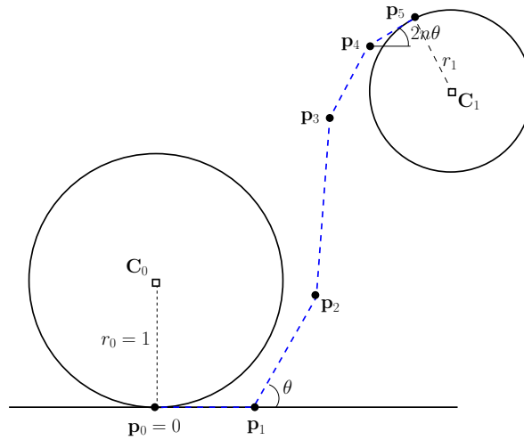
Figure 5.23: Geometrical parameters of an S-shaped ATPH spiral used as G^2 connection between two external circles.
