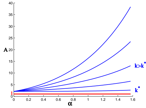
Figure 5.18: Behavior of A(k, \alpha) for \alpha \in (0, \pi/2) .
