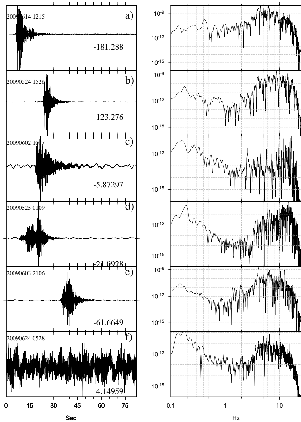
Figure 1.22: Typical unfiltered seismograms, indicating date in the upper left and minimum amplitude in \mu\text{m/s} (left) and their spectra (right), recorded at Ubinas experiment in 2009. a) Explosive, b) VT, c) Tornillo, d) Avalanche or rockfalls e) hybrid and f) Tremor.
