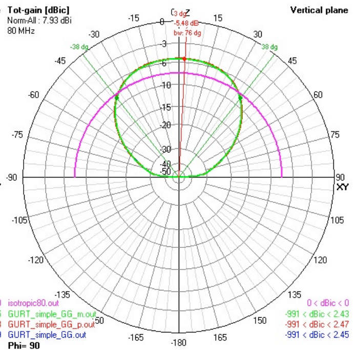
Fig 26b. Simulated beam patterns (at 80 MHz) of the two considered antennas above a realistic ground with varying characteristics: ( \epsilon=18, \sigma=0.9 \text{ mS/m} ) (green), ( \epsilon=20, \sigma=1 \text{ mS/m} ) (red), ( \epsilon=22, \sigma=1.1 \text{ mS/m} ) (blue).
