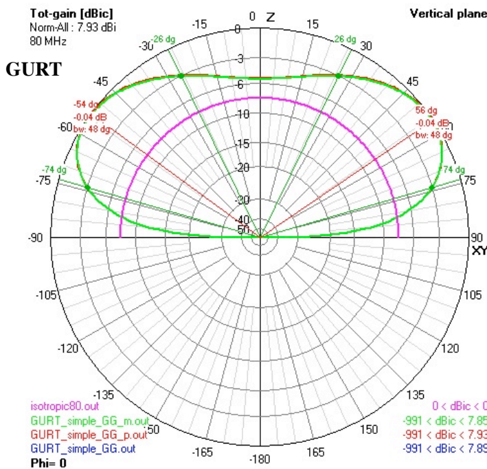
Fig 26b. Simulated beam patterns (at 80 MHz) of the two considered antennas above a realistic ground with varying characteristics: ( \epsilon=18, \sigma=0.9 \text{ mS/m} ) (green), ( \epsilon=20, \sigma=1 \text{ mS/m} ) (red), ( \epsilon=22, \sigma=1.1 \text{ mS/m} ) (blue).
