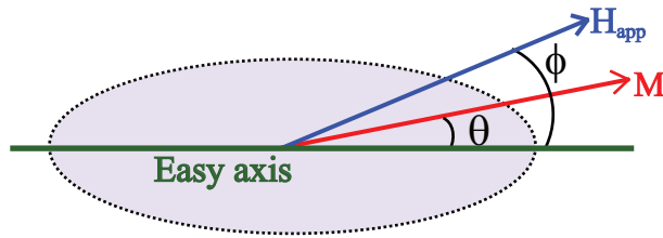
Figure 2.11: Geometry for applied magnetic field, magnetization and easy magnetization axis in the Stoner-Wohlfarth model.
