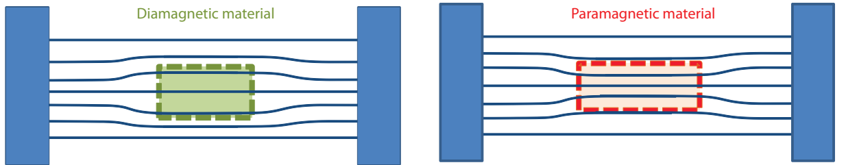
Figure 2.1: Picture of field lines in presence of diamagnetic and paramagnetic materials.
