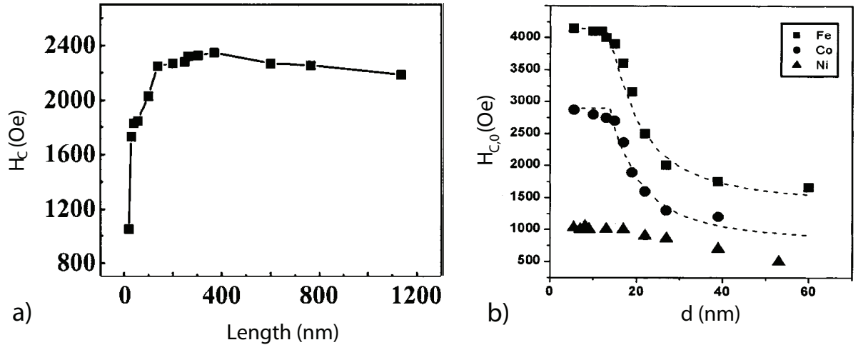
Figure 2.21: Results from Fe, Co and Ni FNW. In (a) the dependence of coercive field with the length for Co nanowires and in (b) the dependence of the extrapolated coercive field at T = 0 K for FNW of Fe, Co and Ni with the nanowire diameter (adapted from (SELLMYER; ZHENG; SKOMSKI, 2001; ZENG et al., 2002))
