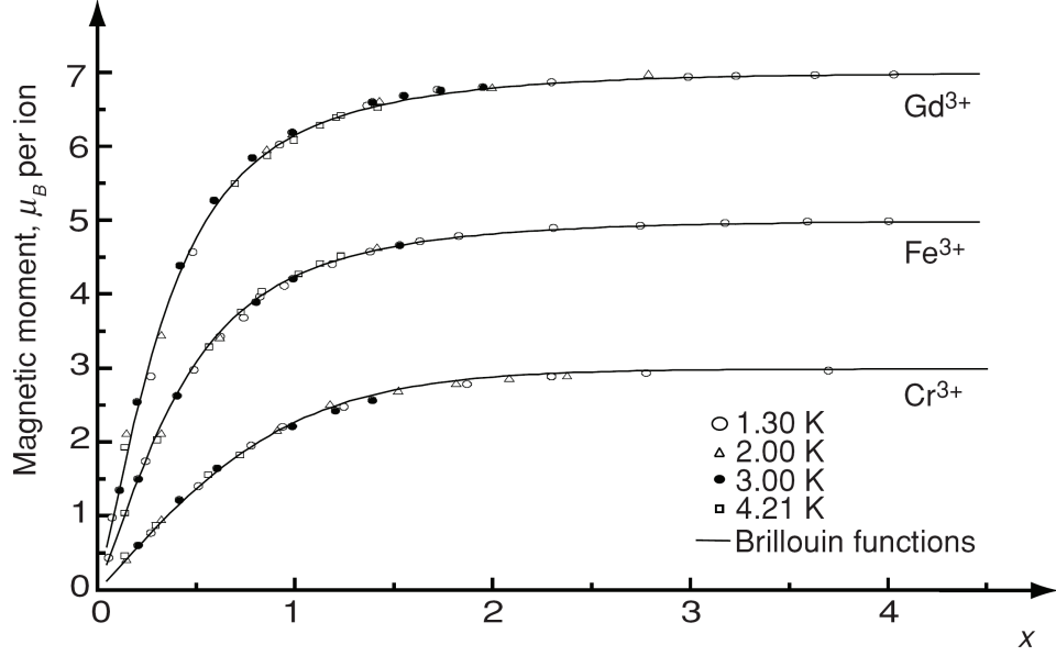
Figure 2.3: Reduced magnetization curves for three paramagnetic salts compared with Brillouin theory predictions. (Reprinted from (COEY, 2010)).
