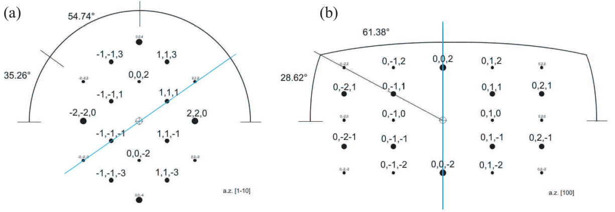
Figure 6.1: Diffraction patterns of cubic CeO 2 (a) and hexagonal Co (b) at a zone axis corresponding to the geometry of HRTEM images. The blue lines represent the [111] direction of CeO 2 and [0001] direction of hcp Co (Adapted from (BONILLA, 2010)).
