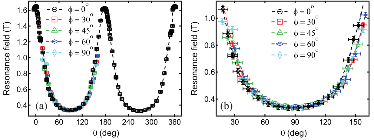
Figure 6.8: Resonance field for \theta -scan for different \phi angles. In (a) results are presented for the full 360 degrees range and (b) shows the same data in a zoom.
