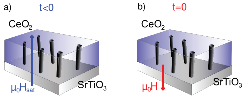
Figure 5.8: Procedure used for magnetic viscosity measurements in Co nanowires assemblies embedded in \text{CeO}_2/\text{SrTiO}_3(001) .
