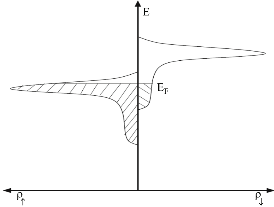
Figure 2.7: Schematic spin-split bands in the ferromagnetic model of Stoner (Reprinted from ref (NOLTING; RAMAKANTH, 2009)).
