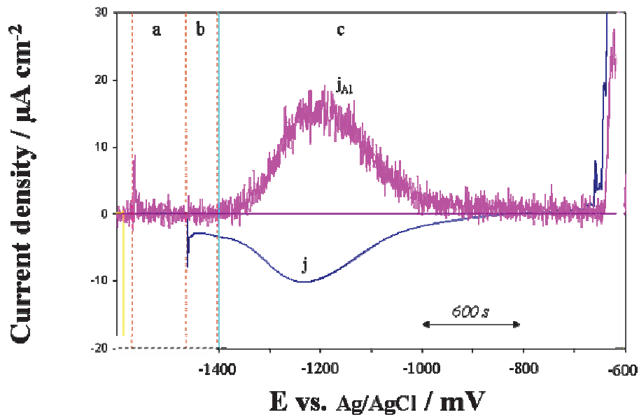
Figure 6.1. 99.99% Al (AA1199): AESEC polarization curves in 30 g/l NaCl solution at pH = 6.1. The curve is divided into period (a) open circuit exposure to electrolyte; (b) imposed potential of -1400 mV vs. Ag/AgCl; (c) anodic potential sweep at 0.5 mV/s. Prior to (a) a blank solution was pumped into the plasma, bypassing the flow cell, to define the background intensity level.
