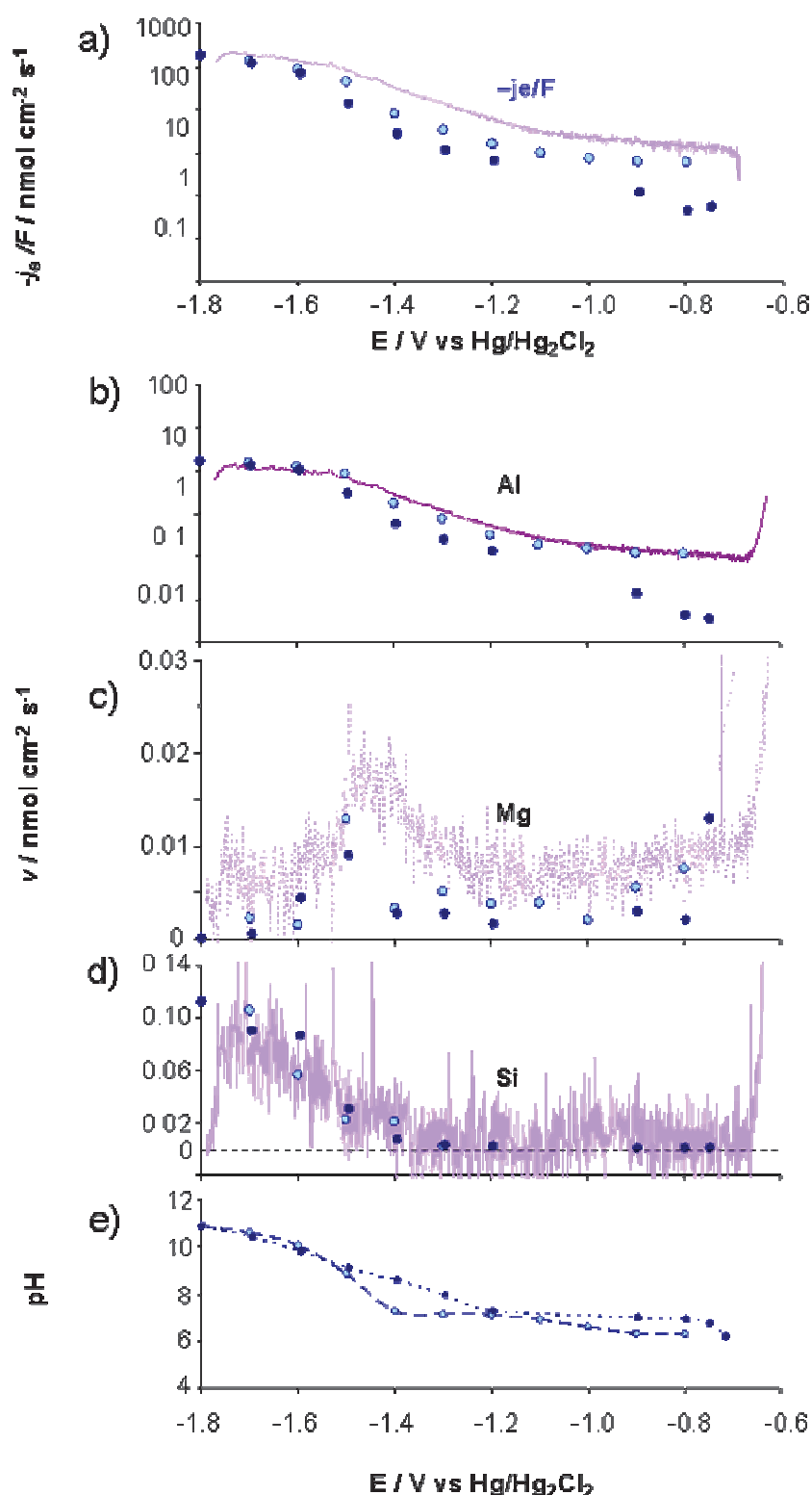
Figure 7.2. Typical AESEC polarization curves for AA6061 alloy in 3% NaCl, initially neutral, electrolyte. Dissolution profiles are shown for the hydroxide formation rate, v_{OH} = i_e / (A F) (a), Al (b), Mg (c) and Si (d). Continuous lines represent potentiodynamic curves obtained at 1 \text{ mV s}^{-1} . Discrete points represent potentiostatic measurements obtained by direct potential step (filled circles) and with preactivation (empty circles); (e) gives the pH of the electrolyte measured downstream from the flow cell, obtained during the potentiostatic experiments.
