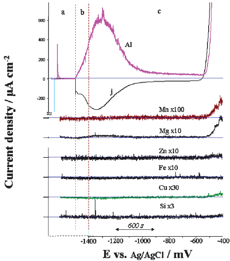
Figure 6.4 AA2214: AESEC polarization curves in 30 g/l NaCl solution at pH = 6.1. The curve is divided into period (a) open circuit exposure to electrolyte; (b) imposed potential of -1400 mV vs. Ag/AgCl; (c) anodic potential sweep at 0.5 mV/s.
