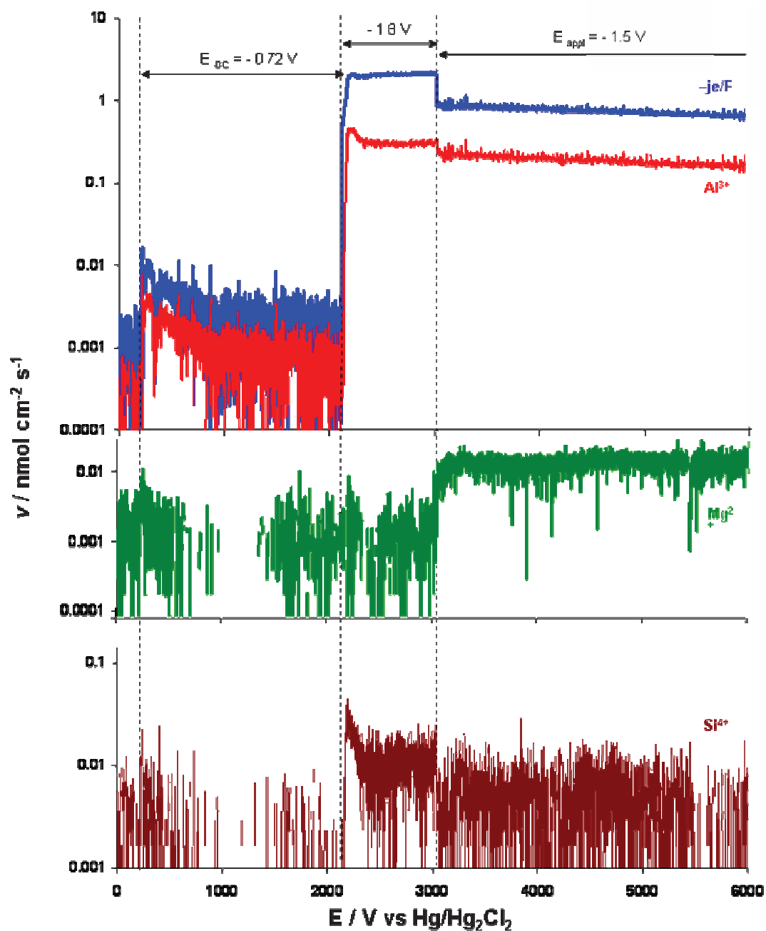
Figure 7.1. The typical elemental dissolution profile during applied cathodic potential followed by activation of the surface by -1.8 V during 900 seconds.
