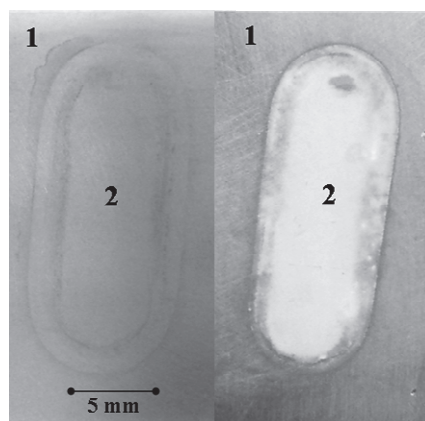
Figure 8.6. General view of aluminum sample after the polarization experiment in 3% NaCl solution (a) and in 3% NaCl + 5 ppm MgCl 2 (b) demonstrating visible formation of white corrosion product in presence of Mg 2+ . The unreacted area (outside of the cell) is indicated as 1 and the exposed in the AESEC experiment area is indicated as 2.
