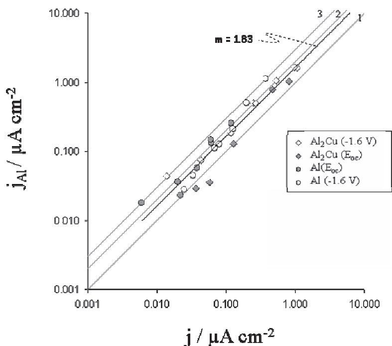
Figure 6.8. j_{\text{Al}} as a function of j , integrated during the final 100 s of the potential step experiments for 99.99% Al (circles) and \text{Al}_2\text{Cu} (diamonds). Potential step experiments were performed in both the anodic (empty) and cathodic (filled) directions. Straight lines indicate m=1 , m=2 , and m=3 as indicated. A least squares fit to the entire data set is also shown indicating a slope of 1.83.
