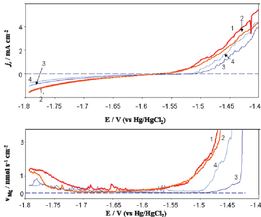
Figure 8.8. Polarization curve (a) and Mg dissolution rate evolution (b) for Mg without (1 – fresh polished surface, 2 – after 40 min exposure to air) and with 5 ppm of Al 3+ in the solution (3 – fresh polished Al, 4 – after 40 min exposure to air).
