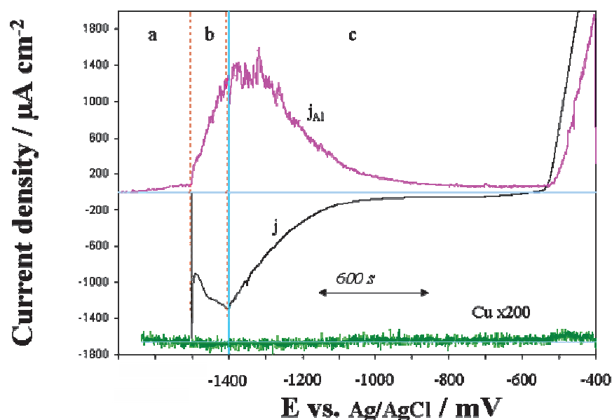
Figure 6.2. Synthetic \text{Al}_2\text{Cu} : AESEC polarization curve in 30 g/l NaCl solution at pH = 6.1. The curve is divided into period (a) open circuit exposure to electrolyte; (b) imposed potential of -1400 mV vs. Ag/AgCl; (c) anodic potential sweep at 0.5 mV/s.
