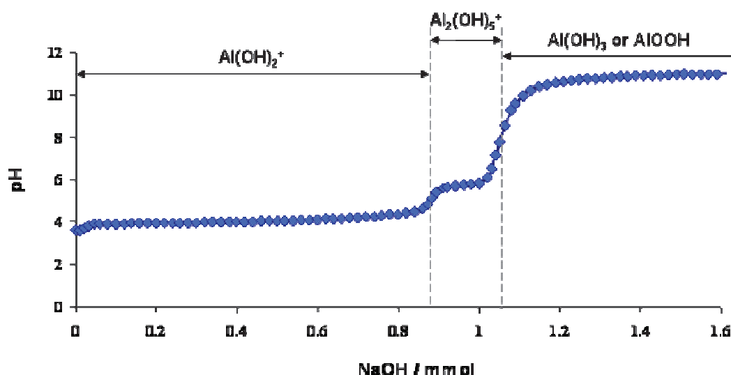
Figure 6. The definition of the stoichiometry of Al reaction with hydroxide during titration experiment of 0.4 mmol of \text{Al}^{3+} by NaOH.
