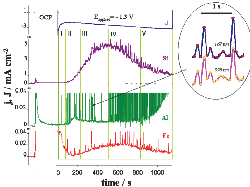
Figure 5.6. Total electrochemical current J and the elemental dissolution currents j_{\text{Si}4+} , j_{\text{Al}3+} , j_{\text{Fe}3+} measured by AESEC during spontaneous reaction and under applied cathodic potential ( E_{\text{applied}} ) -1.3 V vs. Ag/AgCl as indicated. See text for more details.
