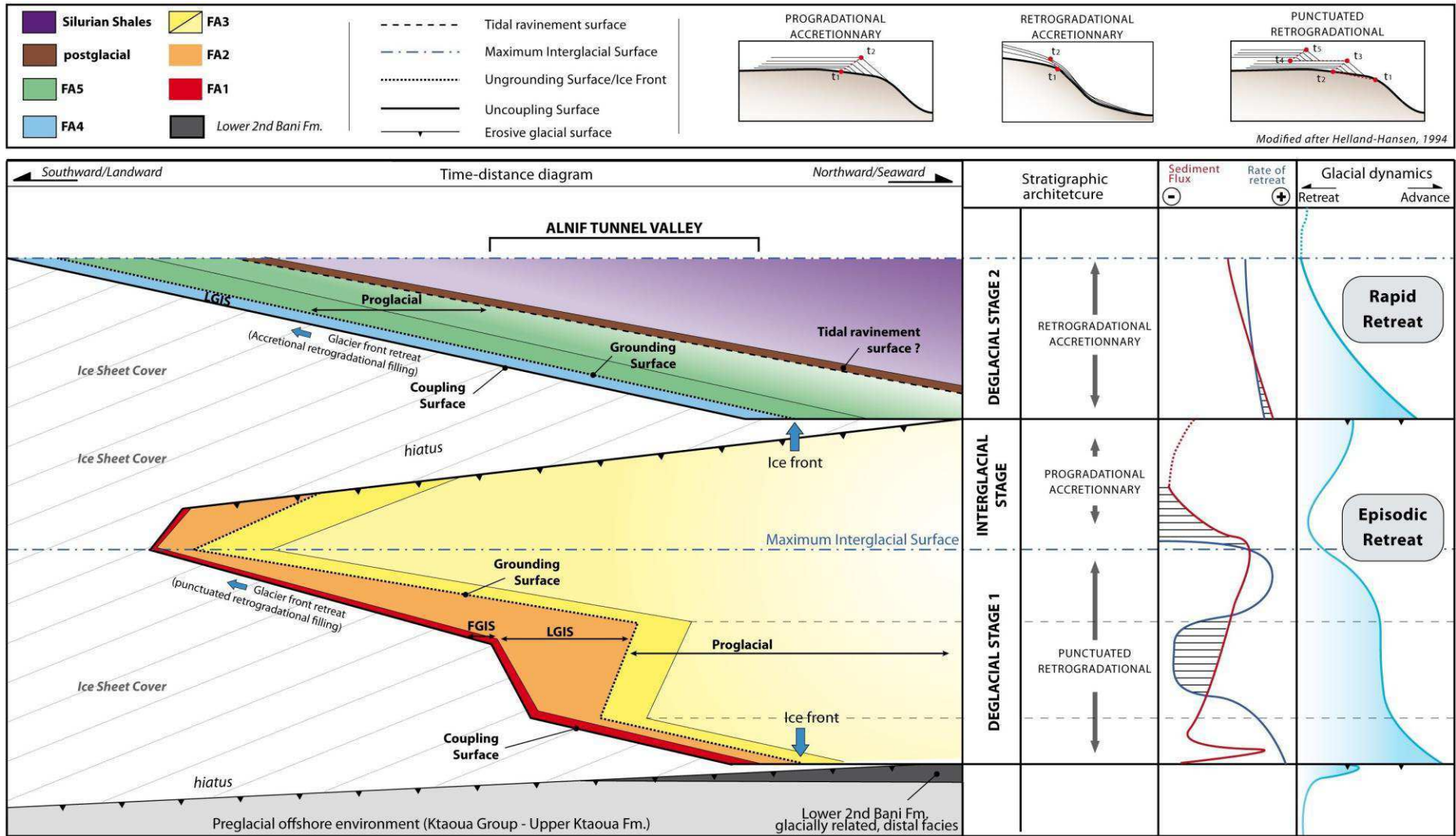
Figure 16: Time-distance diagram based on the tunnel valley infill characteristics, variations of sediment fluxes/supply, rate of retreat and interpreted glacial dynamics. Major facies associations are reported together with depositional environments (FGIS: Fully grounded ice-sheet; LGIS: Lightly grounded ice-sheet; GM: Glaciomarine; PG: Proglacial), together with the major depositional stages.
