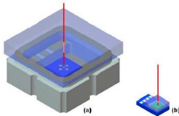
Figure 1.15 Laser trimming [51]
