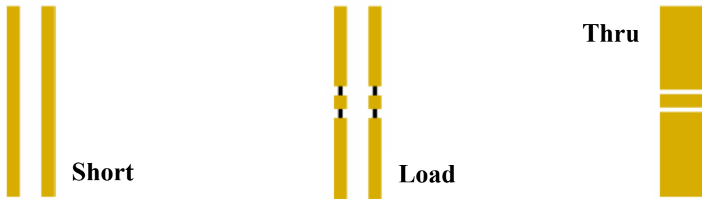
Figure 4.2 Standard de type SOLT
