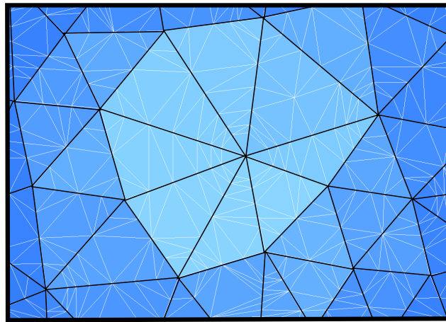
Figure 6.5 – Non-matching grids in 3D, with matching geometry. (luminance codes for the 3D). The black triangles represent the BEM meshes, whereas the white the FEM's.
