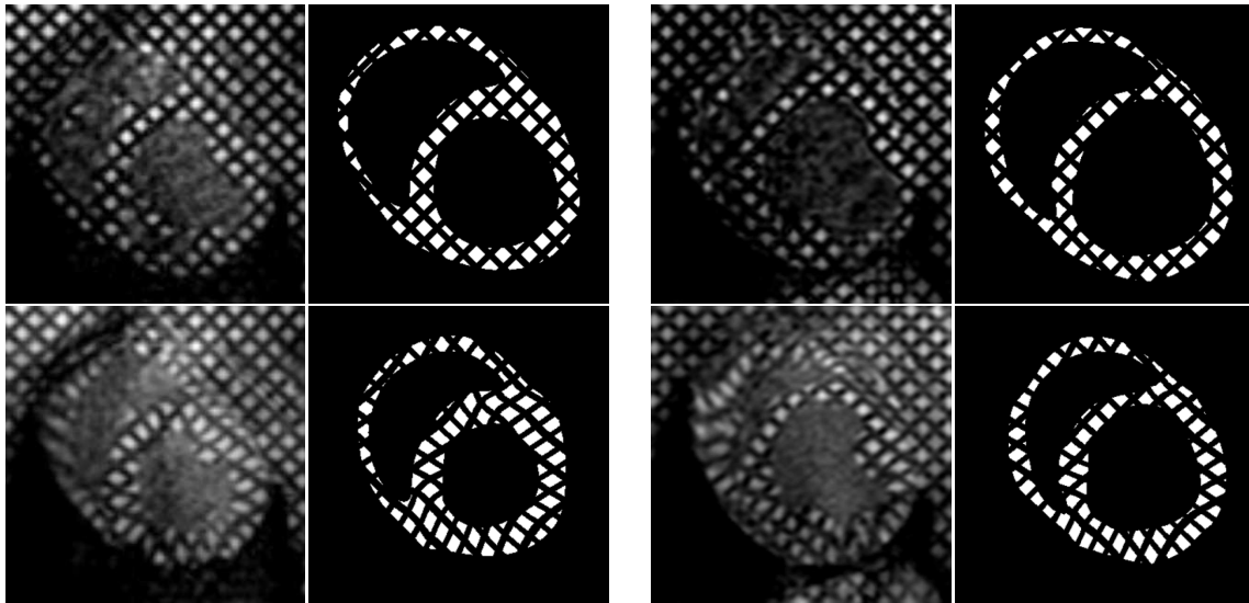
Figure 6.8: Comparison of MR and synthetic tagged images for baseline (left four images) and T0+10 stage (right four images). End-diastolic time frames are displayed in the upper row, end-systolic time frames in the lower row.
