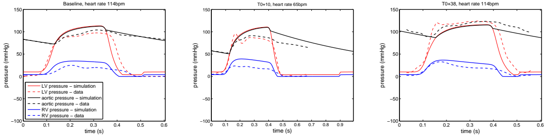
Figure 8.2: Comparison of output pressures of the direct model (solid lines) and the measured values (dashed lines) for each stage of the infarction.
