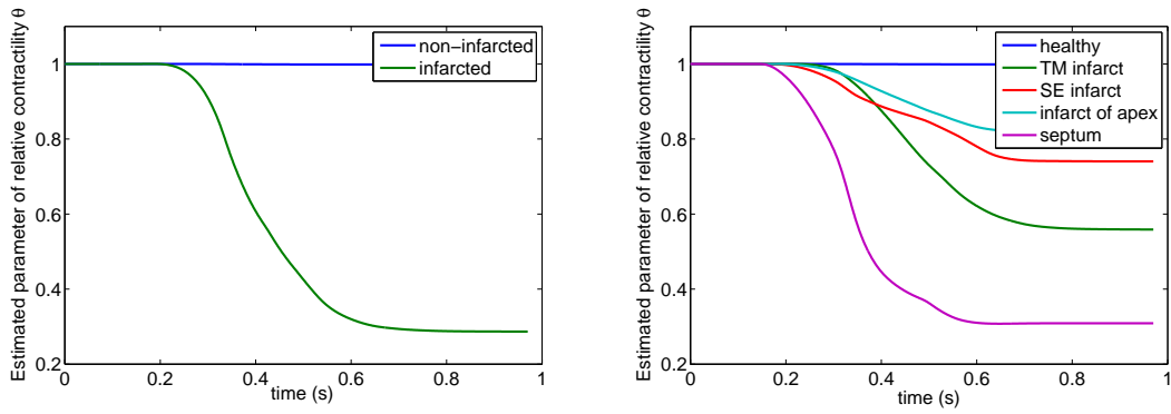
Figure 7.25: Results of estimation of the contractility parameters using synthetic observations in KCL014.
