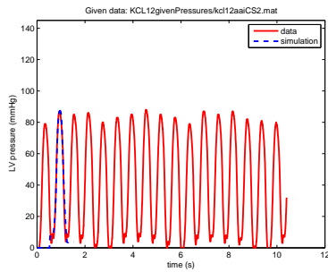
(a) LV pressure in measurement (red line) and in simulation (blue dashed line)
