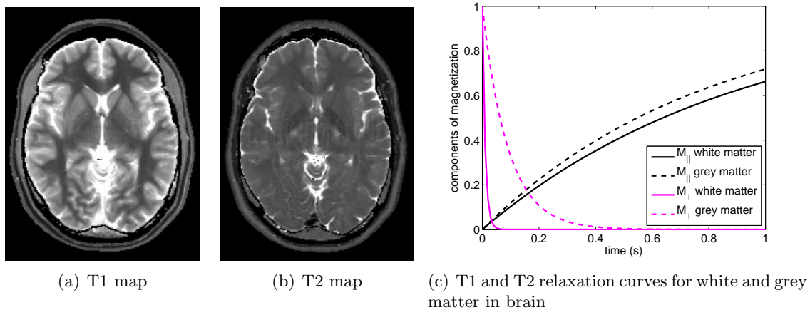
Figure 3.3: Relaxation constants in brain (time constants of T1 and T2 relaxations).
