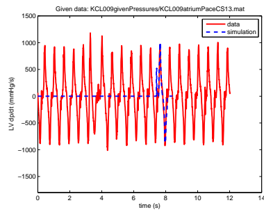
(b) LV dp/dt in measurement (red line) and in simulation (blue dashed line)
