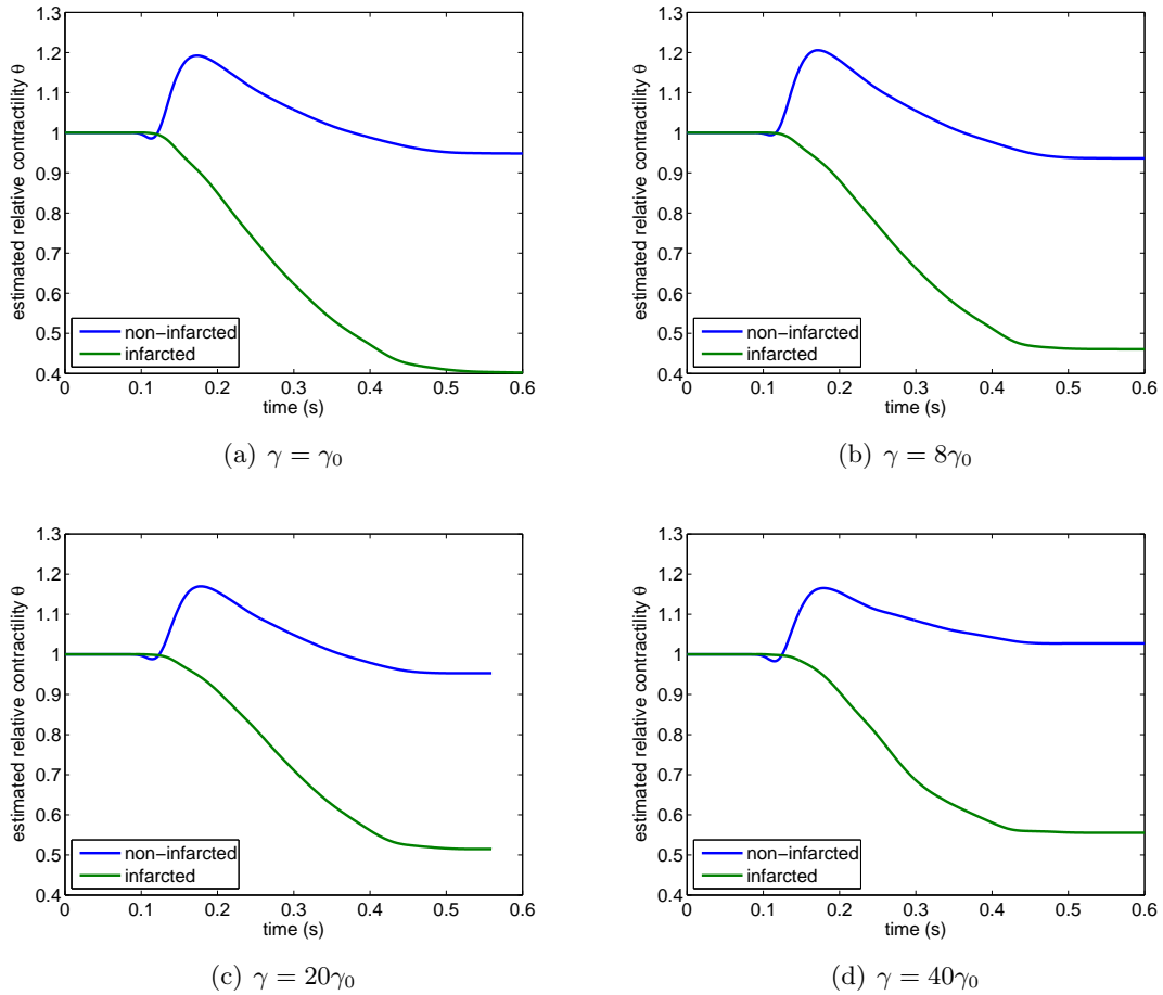
Figure 8.10: Parameter of relative contractivity \theta estimated in a 2-region mesh of stage T0+38 with the non-infarcted and the infarcted region using real observations, with different values of the state estimation gain \gamma .
