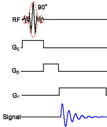
Figure 3.9: A spatial encoding in a single slice selected by the slice selection gradient G_S , which is applied together with the RF pulse. A line in the k-space is selected by the phase encoding gradient G_\phi . The frequency encoding (readout) gradient G_f is applied during the whole period of signal sampling, and the corresponding line in the k-space is filled.
