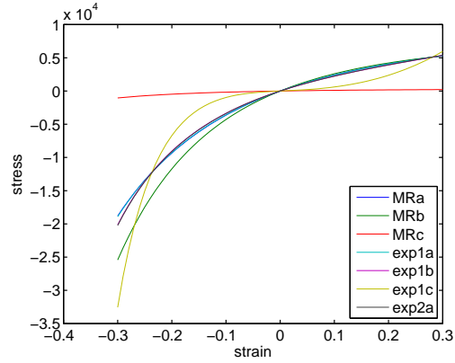
Figure 5.4: Examples of stress–strain curves for several material laws. Note, that the exponential material has a softer response for small strains. The parameters of the materials are in Table 5.1.
