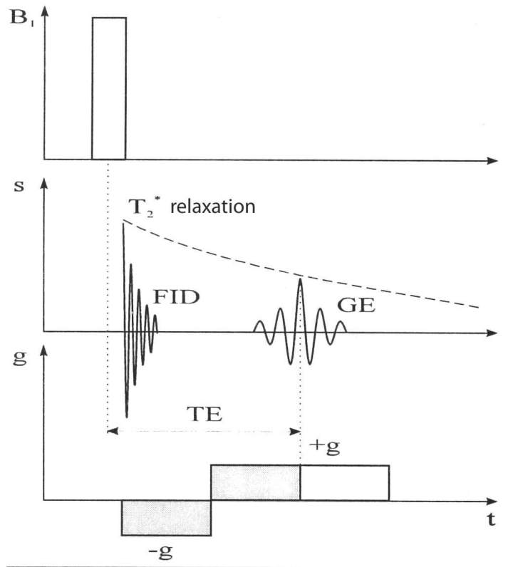
Figure 3.7: Settings of Gradient Echo sequence (GE). From [110].
