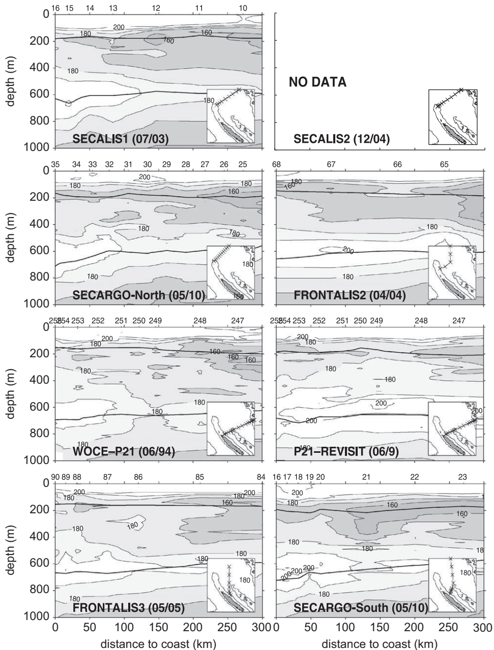
Fig. 6. Same as Fig. 5, but for oxygen concentration (contour every 10 \mu\text{mol/kg} ). The 25.0 (oxygen minimum) and 27.0 (oxygen maximum) isopycnals are indicated by the thick black lines.
