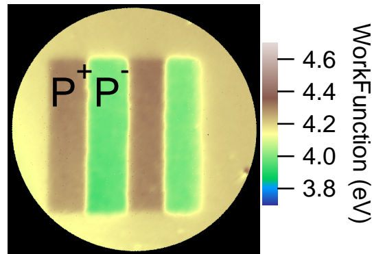
Figure A.4: Work function \Phi_S map of a domain-patterned 70 nm thin \text{BiFeO}_3 film.
