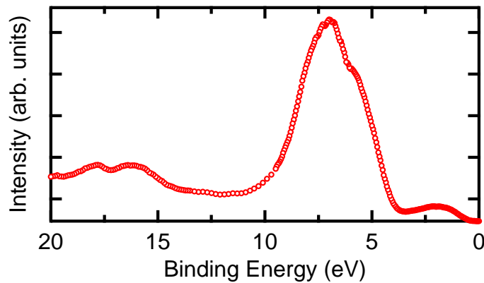
Figure 3.29: Angle-averaged valence band spectrum of the BaTiO 3 single crystal.
