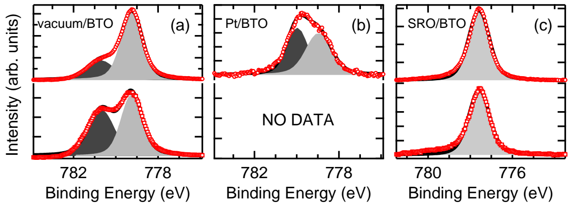
Figure 4.22: Ba3d_{5/2} core-level spectra of a BTO layer for different interface configurations and take off angles. Top panels show the normal emission (red circles) and bottom panels show the grazing emission (red squares) data for the (a) vacuum/BTO, (b) Pt/BTO and (c) SRO/BTO interface.
