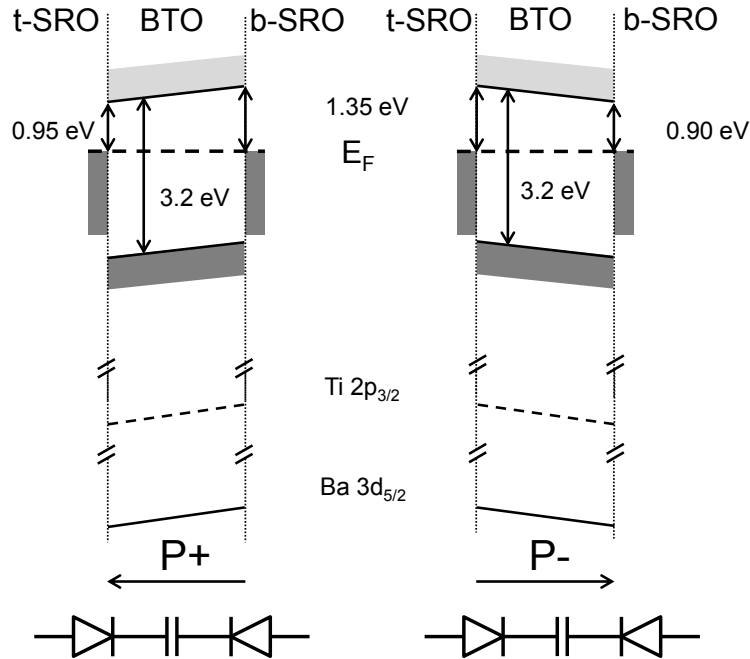
Figure 4.24: Band lineup for the P^+ (left) and P^- (right) polarization states. t-SRO (b-SRO) stands for top (bottom) SRO electrode. Since, photoemission does not give access to the bottom interface, the barrier heights at the bottom interface are purely hypothetical.
