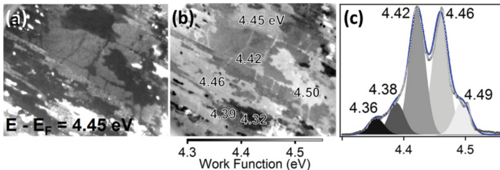
FIG. 5. (Color online) (a) Threshold image at E - E_F = 4.45 eV with a 53 \mu\text{m} field of view showing clear intensity contrast due to work function variation across the surface. (b) Work function map of the FoV obtained from a pixel by pixel analysis of the threshold spectra. (c) Histogram of the work function values in (b) showing five distinct Gaussian distributions, corresponding to five distinct work function values.
