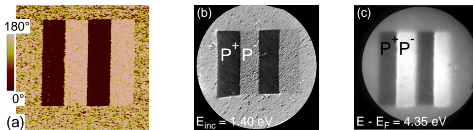
Figure 3.9: (a) PFM phase image of written P + /P - domains. Each domain is 20 \times 5 \mu\text{m}^2 , (b) LEEM raw image for E_{\text{inc}} = 1.40 \text{ eV} , (c) PEEM raw image at E - E_{\text{F}} = 4.35 \text{ eV} (the three images have been acquired on the 70 nm BFO film).
