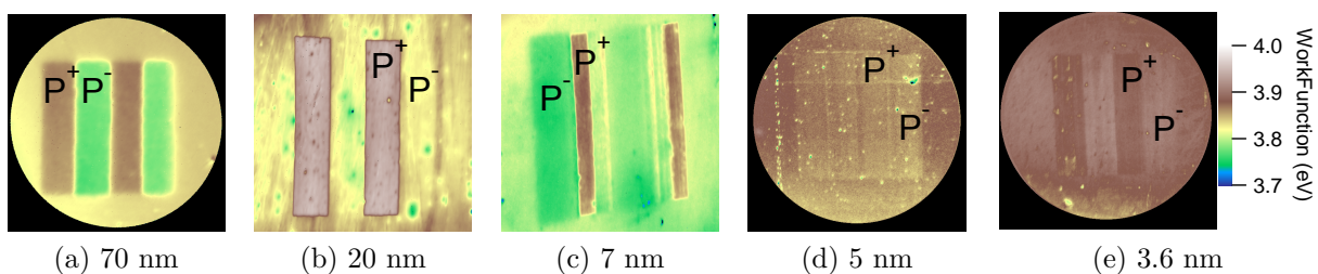
Figure 3.12: Work function maps for every thickness. A drop in workfunction contrast occurs between 7 and 5 nm.
