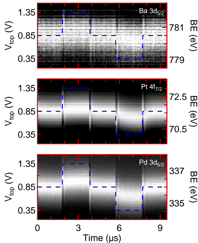
Figure 4.12: Photoemitted electron intensity as a function of time and binding energy (BE) for the three core-levels \text{Pd } 3d_{5/2} , \text{Pt } 4f_{7/2} and \text{Ba } 3d_{5/2} . The blue dotted curve shows the pulse train.
