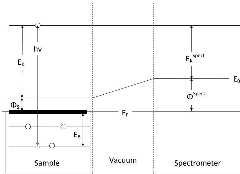
Figure 1.7: Energy alignment of a metallic sample connected to the spectrometer in thermodynamic equilibrium (both have the same Fermi energy E_F ) The energy scale in the spectrometer (of work function \Phi^{\text{Spect}} ) has to be calibrated in order to obtain the correct binding energies E_B of electron photo-emitted from the sample (of work function \Phi_S ) with a kinetic energy E_K . E_0 is the vacuum energy level.
