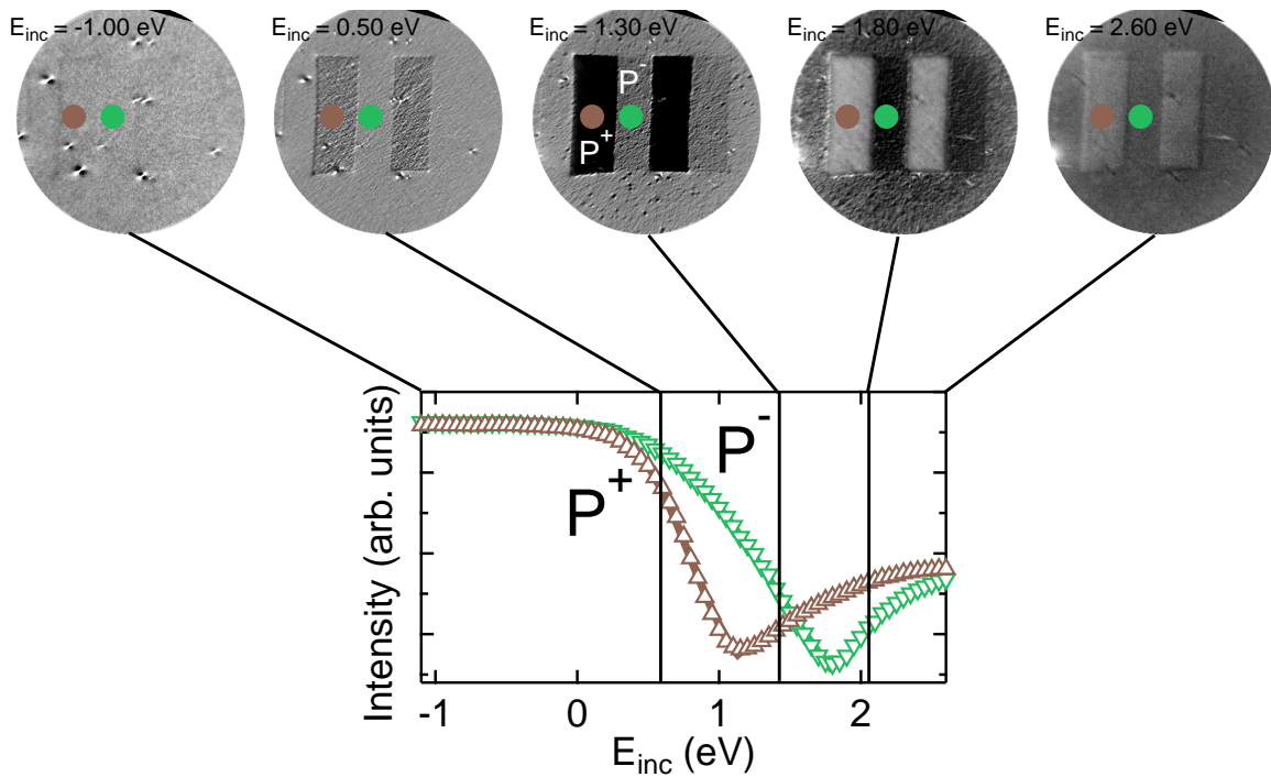
Figure A.6: Typical LEEM image serie on a domain-patterned 70 nm thin \text{BiFeO}_3 film. The reflectivity spectrum (triangles) is constructed by taking the mean intensity value from a \text{P}^+ (brown) or \text{P}^- (green) region. Then, the spectra can be fitted using an error function (solid lines).
