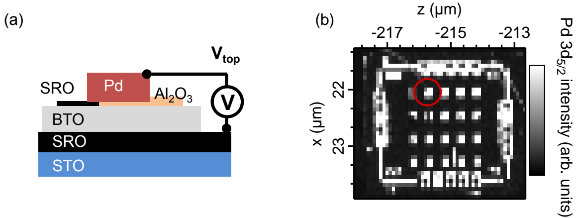
Figure 4.19: (a) Schematic of the capacitor, (b) Pd 3d intensity map for the SRO/BTO/SRO/STO sample showing 20 identical SRO/BTO/SRO capacitors ( (300 \times 300) \mu\text{m}^2 ) on the (5 \times 5) \text{ mm}^2 surface, allowing location of the wired capacitor (red circle). The wire is even visible in this case.
