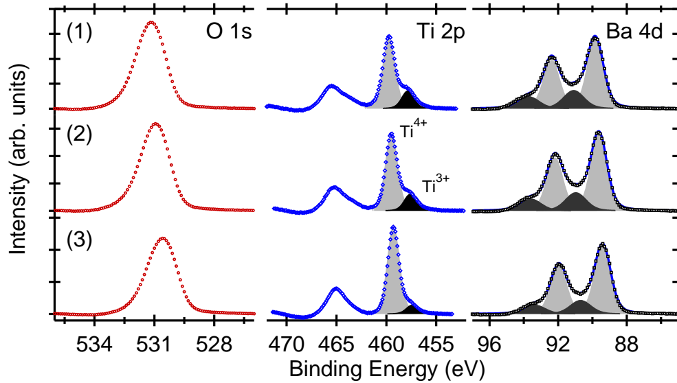
Figure 3.21: XPS spectra at 650 eV photon energy after each annealing step. Steps are described in Table 3.2
