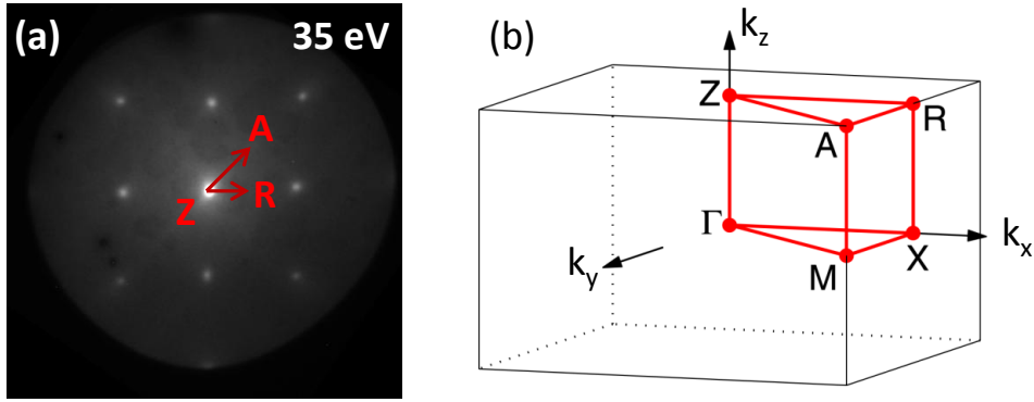
Figure 3.28: (a) 1 \times 1 LEED pattern of the BaTiO 3 single crystal and (b) Brillouin zone of a cubic structure with the high-symmetry points [195]
