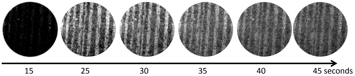
Figure 3.23: PEEM images at (E - E_F) = 3.90 eV under mercury lamp illumination. The grayscale range is the same for every image to show the loss of contrast with time.
