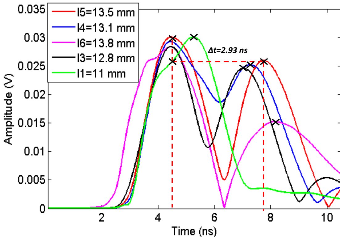
Fig.3. 31 : Some of the de-embedded C-section response measured for different lengths l ( \omega = 3.5 GHz). One of the tags is represented in Fig.3. 25 (b).
