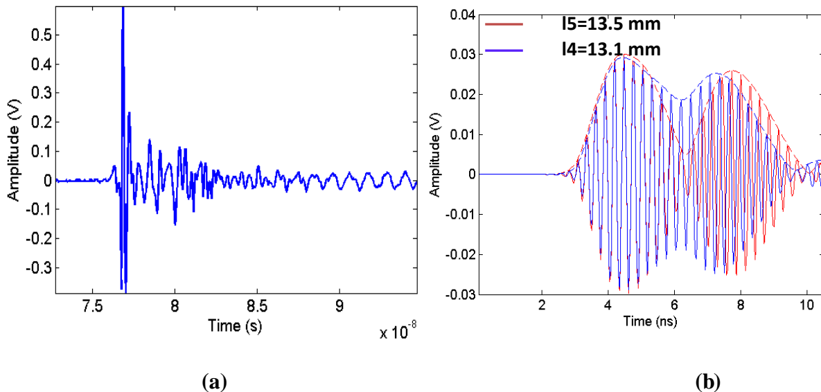
Fig.3. 30 : Tag response before and after numerical filtering. a) Backscattered tag ( l_4=13.1 mm) response. b) Filtered signals at f(11)=3.5 GHz, along with their envelopes for two different tags ( l_4=13.1 mm & l_5=13.5 mm).
