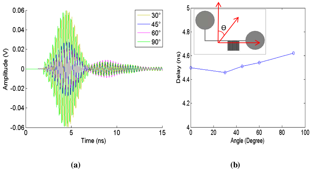
Fig.3. 35: Simulated results for the tag with different orientations. a) Simulated backscattered results obtained when the tag is rotated for different angles \Theta . b) Obtained delayed between structural mode and tag mode as a function of angle. Insight: tag with coordinates.
