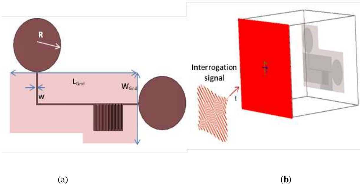
Fig.3. 23 : Structure of the chipless tag with simulation model. a) Tag layout with different design parameters; R=13 mm, w=0.7 mm, L_{gnd}=70 mm, W_{gnd}=34 mm. b) Simulation model with a plane wave as an excitation signal.
