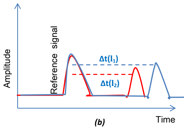
Fig.1. 2 : Principle of operation of time domain chipless RFID system and time domain encoding. a) Chipless RFID system. b) Principle of encoding.
