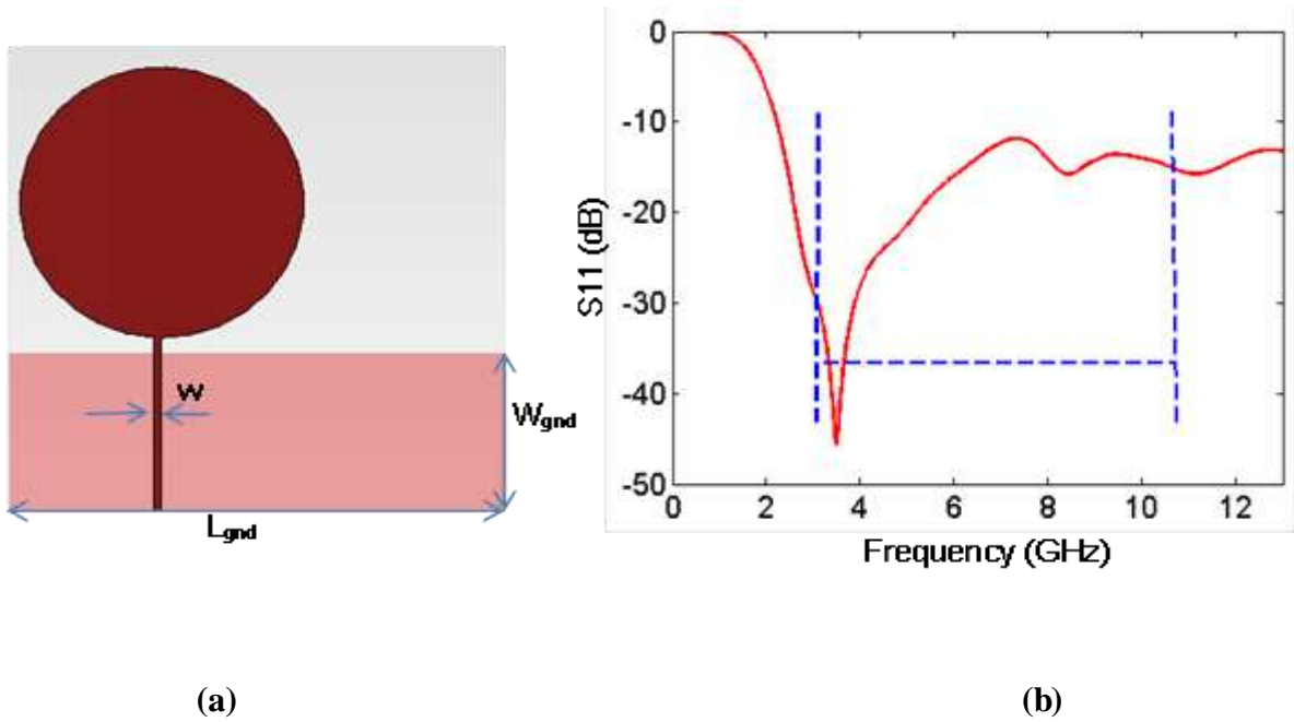
Fig.3. 20 : Structure of the UWB antenna and the simulated S11. a) Antenna layout, b) simulated S parameter. The UWB band is marked in between the dotted blue lines w=0.7 mm, L_{gnd}=45.3 mm, W_{gnd}=14.97 mm; \epsilon_r=3.55 , \tan\delta=0.0027 , h=0.8 mm.
