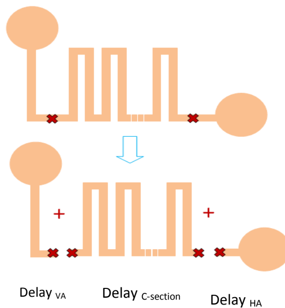
Fig.3. 28 : Principle used to extract the group delay and hence the tag information which contains antennas.
