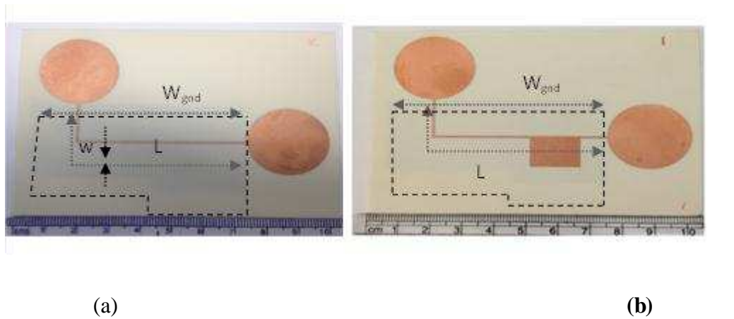
Fig.3. 25 : The reference tag and chipless tag used. a) Reference tag. b) Chipless tag with 10 C-sections; bottom ground plane is marked as dashed lines. W_{\text{gnd}}=70 mm, L=79.1 mm, w=0.7 mm.
