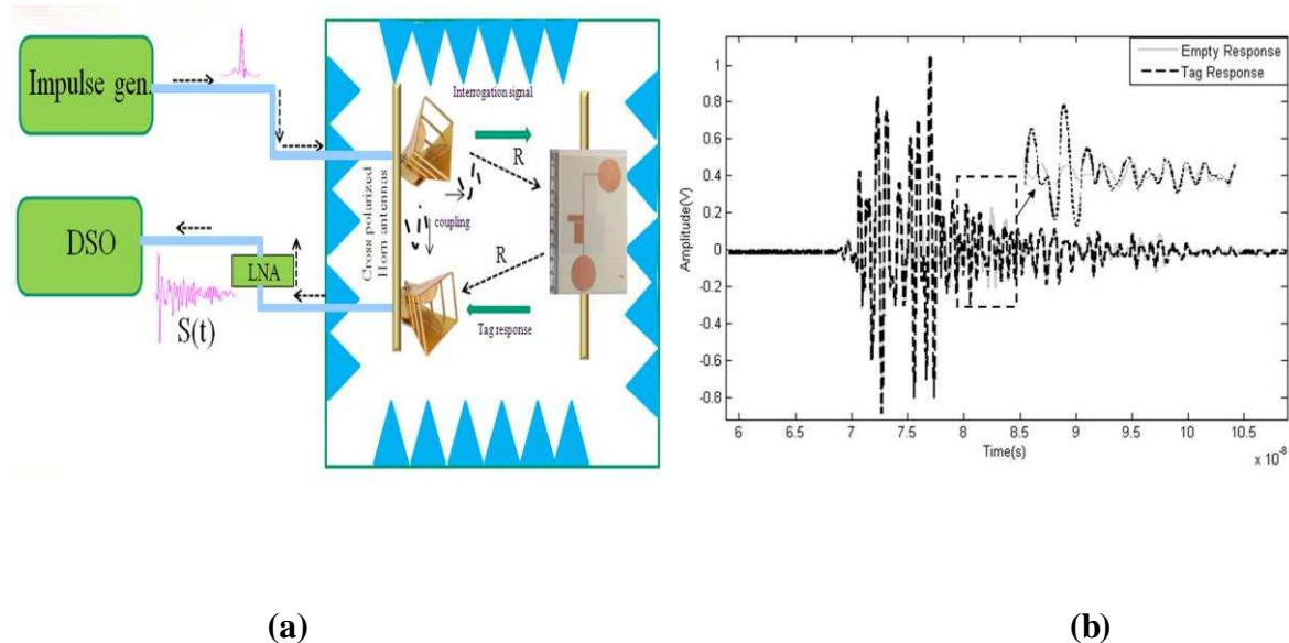
Fig.4. 8 : Experimental set up together with empty ad tag responses. a) Measurement Set-Up. b) The measured empty response and tag response, insight view: zoomed version of the two responses.
