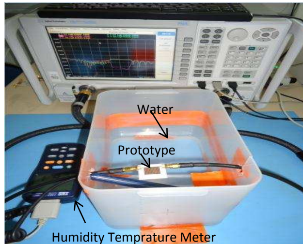
Fig.6. 4 : Measurement set-up for the sensor tag prototype.
