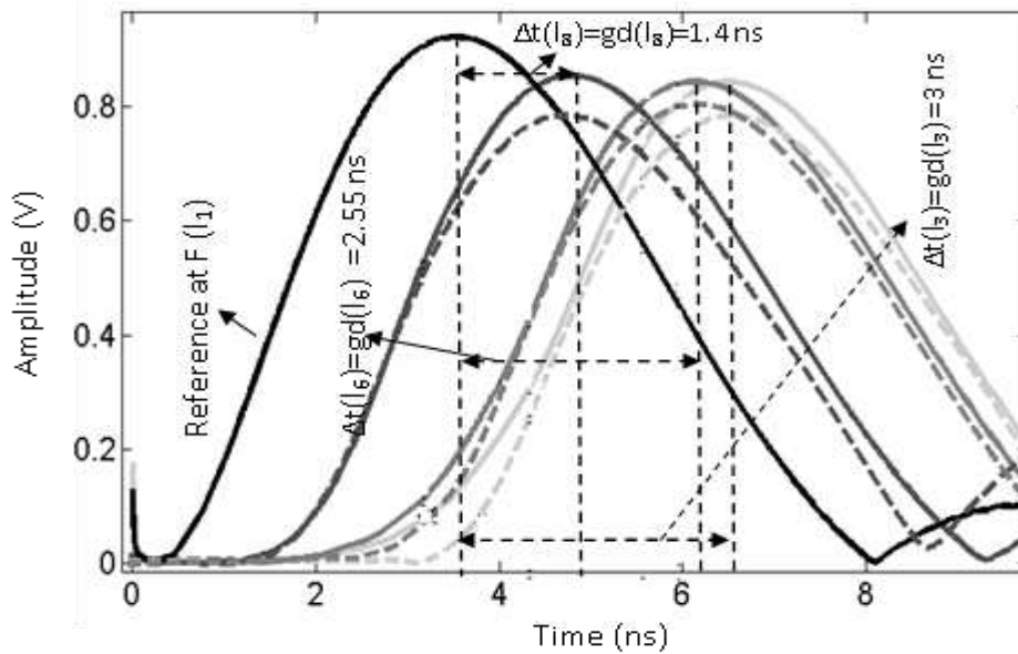
Fig.3. 18 : Simulated (solid line) and Measured (dashed line) time delay for single group of 10 C-section as a 2-port network; The reference signals are superimposed. l_5 = 13.1 mm, l_6 = 12.8 mm, l_8 = 11 mm, g = 0.1 mm, w' = w = 0.7 mm; \epsilon_r = 3.55 , \tan\delta = 0.0027 , h = 0.8 mm.
