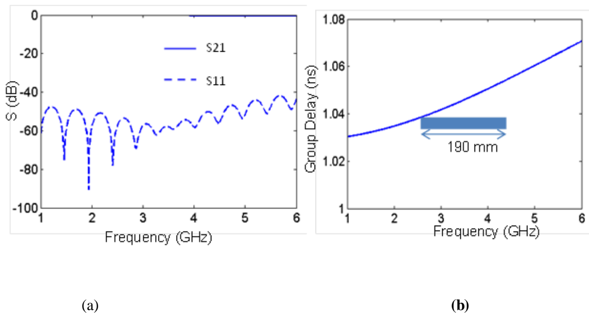
Fig.3. 3 : Simulated S-parameter and delay produced by a linear transmission line. a)S-parameter b) corresponding group delay for 50 \Omega line impedance (at 1.8 GHz). Theoretical delay as per eq. (6) is 1.02 ns. L_{Total}=19 cm, w=1.7 mm, \epsilon_r= 3.55 , \tan\delta=0.0027 , h=0.8 mm.
