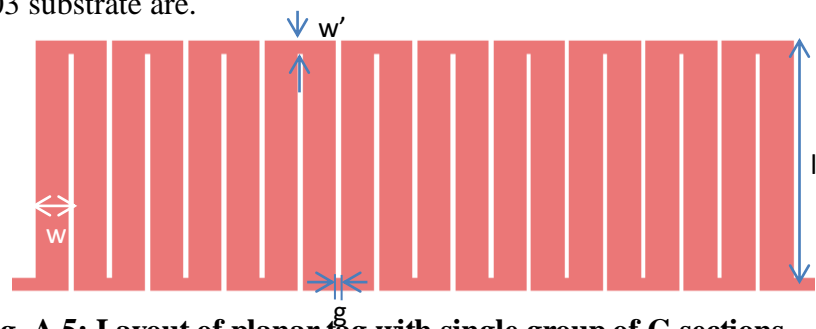
Fig. A.5: Layout of planar tag with single group of C-sections.
