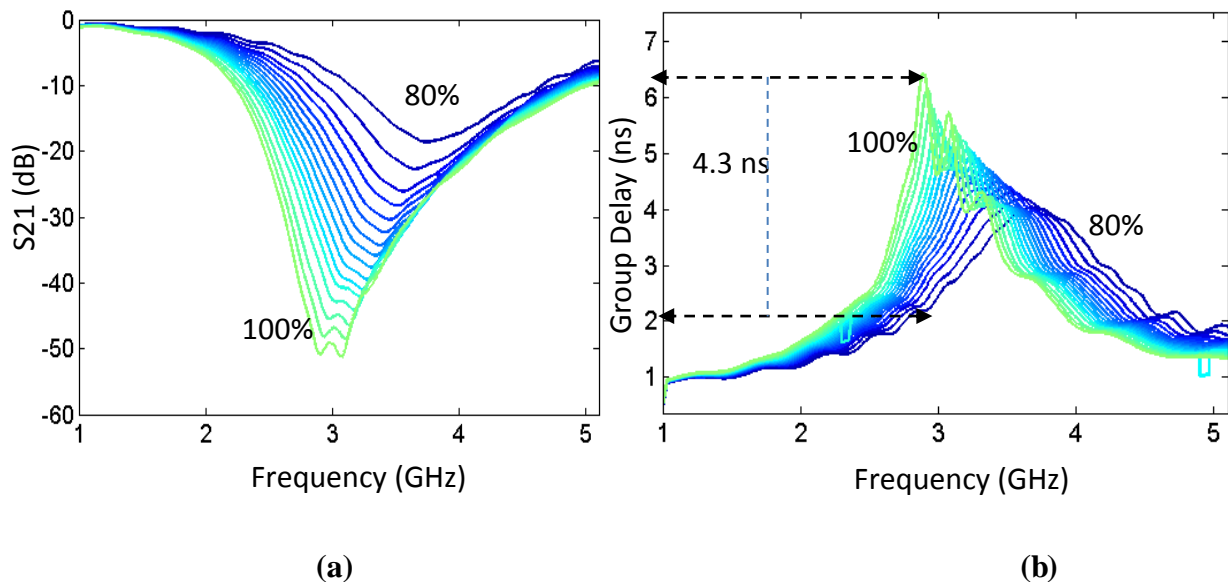
Fig.6. 9 : Repeatability test conducted after 4 days. Measured S_{21} and group delay after increasing the ambient temperature inside the plastic box as 24°C-29°C for an RH variation of 80%-100%. a) S_{21} magnitude, b) group delay.
