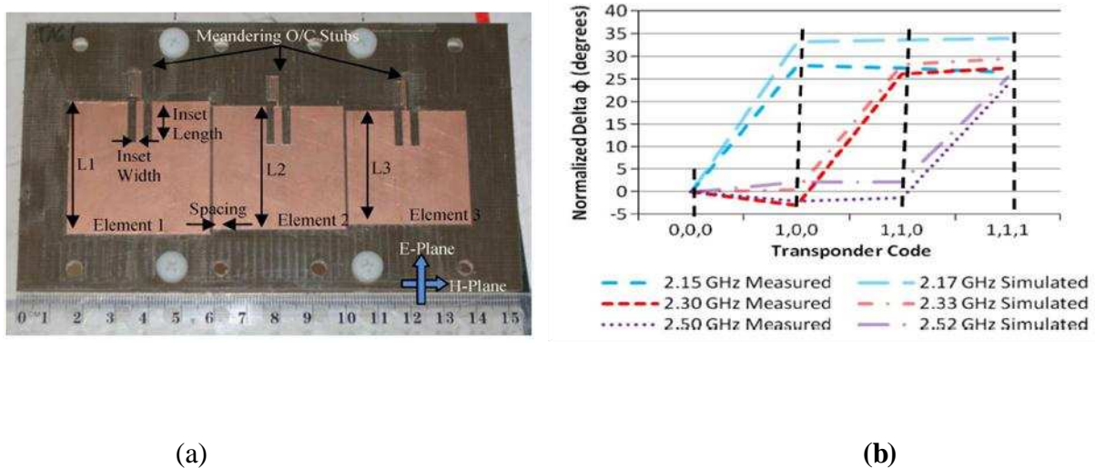
Fig.2. 8: Proposed chipless RFID system and its phase response given in [38]. a) The chipless RFID tag contains three stub loaded microstrip patch antennas. b) Corresponding phase response. The tag has 15 cm length.
