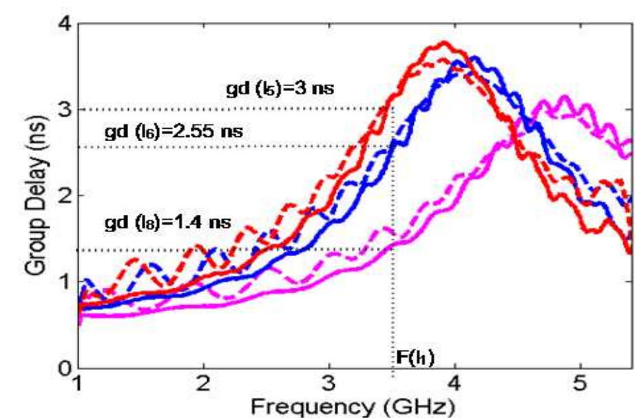
Fig.3. 17 : Simulated and measured (measurement using VNA)group delay for single group of 10 C-section as a 2-port network (see Fig.3. 13); l_5=13.1 mm, l_6=12.8 mm, l_8=11 mm, g=0.1 mm, w'=w=0.7 mm; \epsilon_r=3.55 , \tan\delta=0.0027 , h=0.8 mm.
