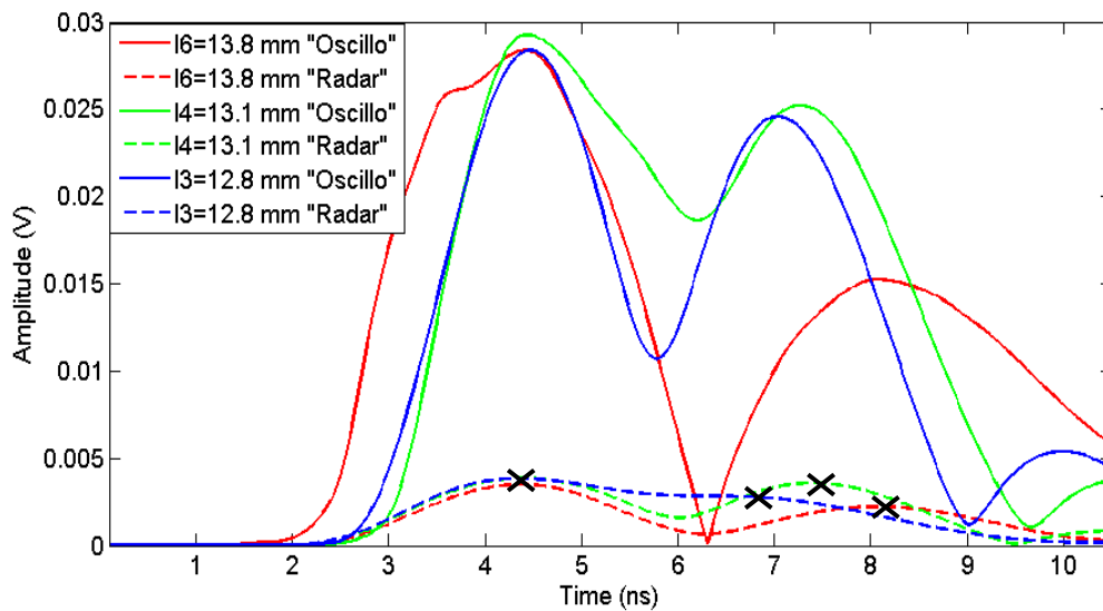
Fig.3. 32 : Some of the de-embedded C-section response measured for different lengths at F (l) = 3.5 GHz. “Oscillo” stands for results using digital oscilloscope and “radar” stands for results using a commercially available UWB radar which can serve like a chipless RFID reader. One of the chipless tag is represented in Fig.3. 25.
