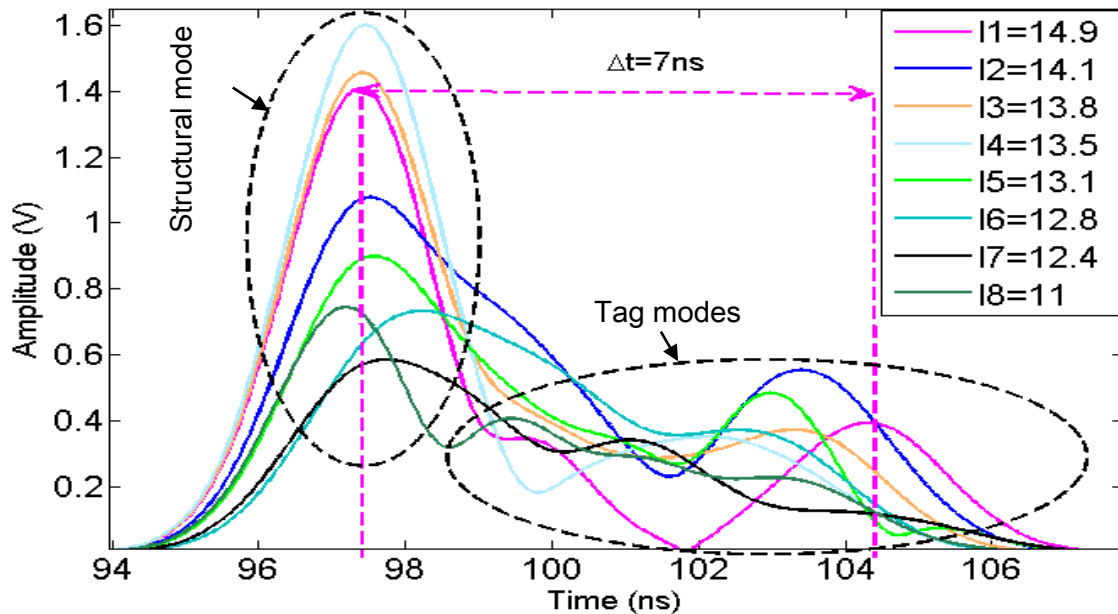
Fig.3. 34 : Measured delays of chipless tag obtained using wavelet approach for single group of 10 C-section with different lengths l1-18 mm at f (l1) = 3.5 GHz. This measurement was done without a reference tag.
