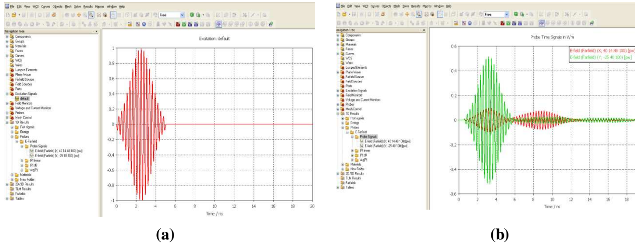
Fig.A.4: The user defined excitation signal and the corresponding back scattered response. a) Excitation signal b) Back scattered signal collected by the far-field probe placed at a particular distance.
