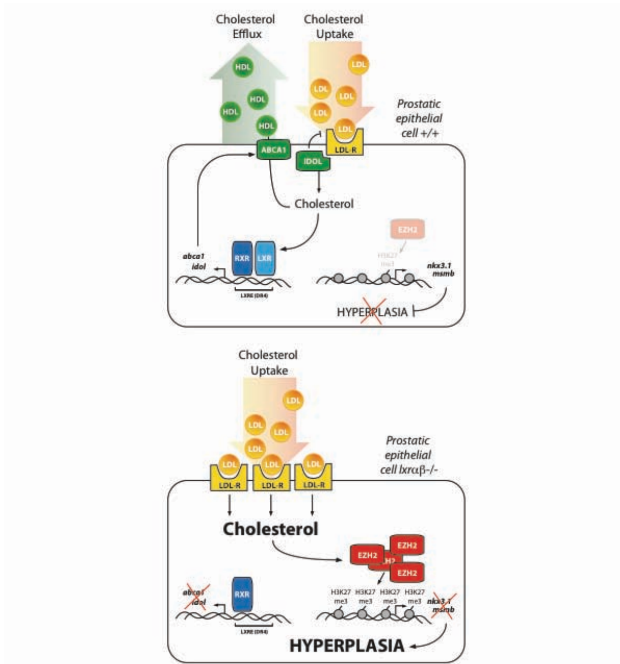
Figure 6: Model of connection between cholesterol homeostasis and regulation of tumor suppressors gene expressions, nkx3.1 and msmb . The upper panel depicts a normal situation when prostatic epithelial cell regulates cholesterol uptake, efflux and storage in order to tightly regulated the amount of cholesterol in the cell. The lower panel recapitulates consequences of LXR ablation and HCD exposure resulting in neoplastic-like lesions.
