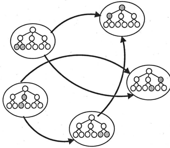
Figure 2.4: Illustration of the Tree-Based Exploration parallel model.
