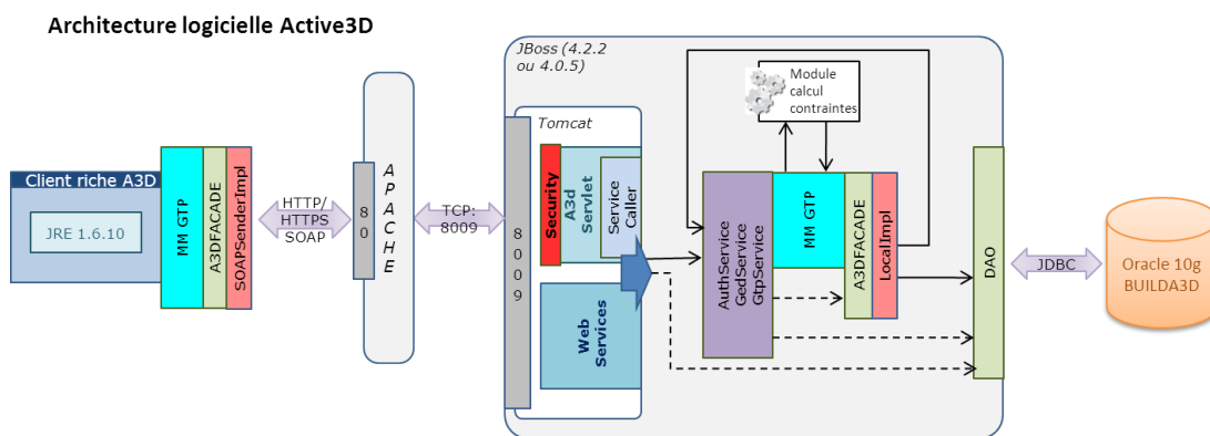
Figure 71. Architecture logicielle 3-tier Active3D
