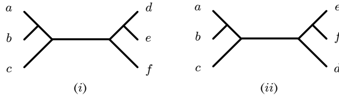
Figure 3.7: Example of greedy consensus trees for the forest depicted in Figure 3.4 - The tree (i) is obtained if the split de|abcf is preferred to the split ef|abcd , otherwise we obtain the tree (ii).
