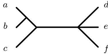
Figure 3.6: Example of semi-strict consensus tree for the forest depicted in Figure 3.4 - The semi-strict consensus trees contains the split ab|cdef which, although not contradicted by any tree, is not included neither in the strict consensus tree nor in the majority-rule consensus tree. For this forest the semi-strict and the Nelson-Page consensus trees (Section 3.2.1.6) are identical.
