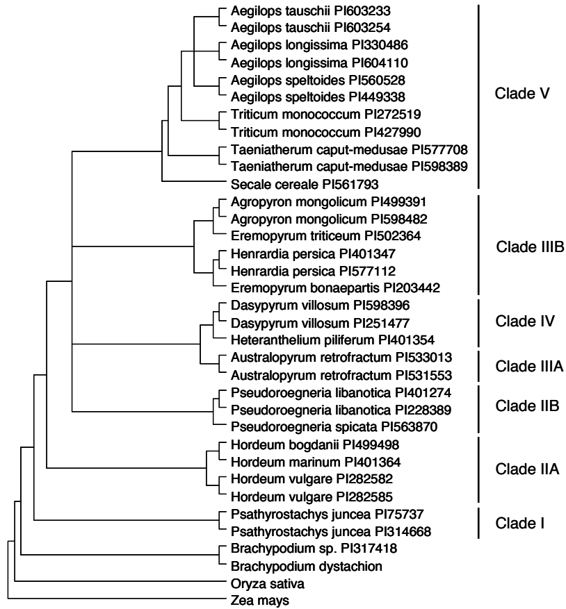
Figure 4.20: PhySIC_IST supertree obtained with the analysis of the 2,700 ML bootstrap trees (100 trees per gene) - Clades are named as in Figure 4.19.
