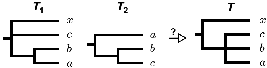
Figure 4.3: An example showing why properties \text{PC} and \text{PI} have to be preferred to properties \text{PC}' + \text{PI}' - Contradictions in the source trees can lead to arbitrary resolution. An example where the presence of contradictions in the source trees (namely, ab|c in T_1 versus bc|a in T_2 ) can lead to the inference of arbitrary clades (namely, excluding x from the clade a, b, c in the supertree T ). This problem is detected by \text{PI} but not by \text{PI}' nor \text{PC}' .
