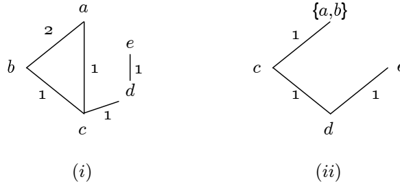
Figure 3.13: Example of the MC supertree algorithm - for the forest \mathcal{F} comprised of two trees T_1 = (((a, b), c), (d, e)) and T_2 = ((a, b), (c, d)) ; w is the constant function w : \{1, 2\} \rightarrow \{1, 1\} . (i) the graph \mathcal{G}(\mathcal{F}, w) . (ii) the graph \hat{\mathcal{G}}(\mathcal{F}, w) . The MC supertree for this forest is the tree ((a, b), c, d, e) .
