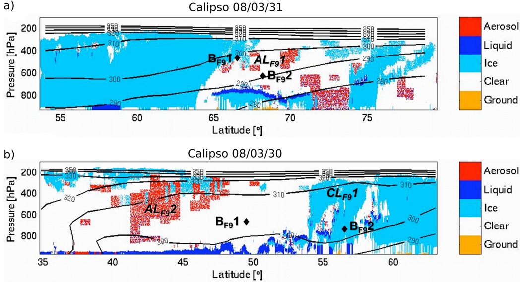
Figure 3.9 Dardar Mask track section observed on 31 March (a) at 13:50:00 UTC and on 30 March (b) at 13:05:00 UTC, 2008 from the synergistic Cloudsat radar and CALIPSO lidar, with FLEXPART air masses (B F9 1 and B F9 2) positions ( \diamond ).
