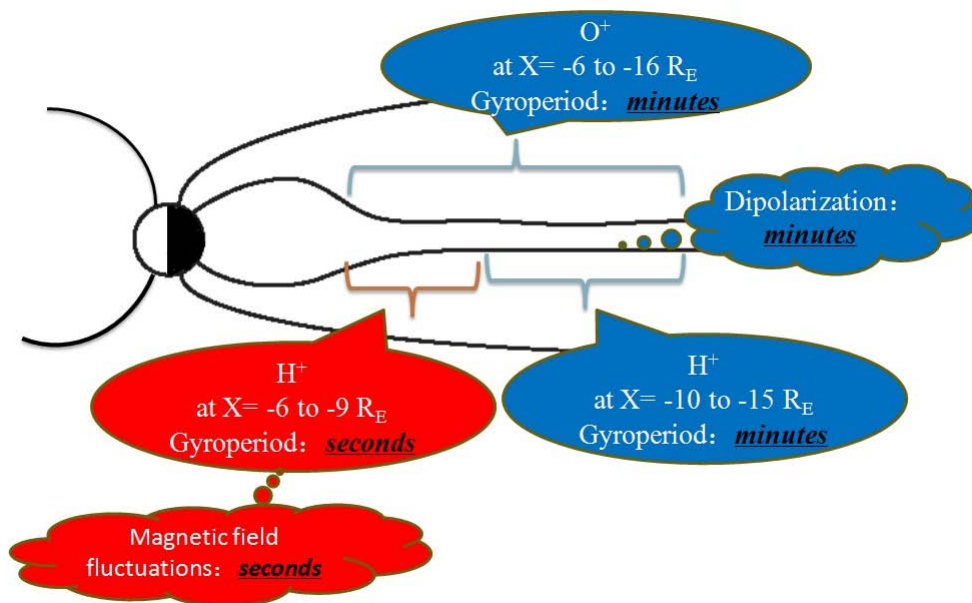
Fig.2.6 Occurring regions of nonadiabatic acceleration for H^+ and O^+ ions
