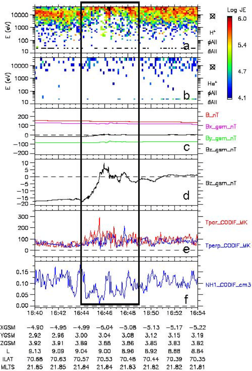
Fig.3.4 The energy-time spectrograms by CIS/CODIF data of SC4 on 30 October 2006. Panel (a) is the H + energy flux. Panel (b) is the He + energy flux. Panel (c) is the magnetic field magnitude and the three components in GSM coordinates. Panel (d) shows along the B z component. Panel (e) shows the parallel and perpendicular temperatures. Panel (f) is the proton number density.
