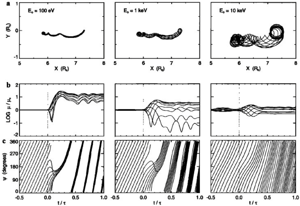
Fig.2.4 Computed trajectories of equatorially trapped \text{O}^+ ions in the time-dependent T-89 model: (a) trajectory projection in the equatorial plane, (b) magnetic moment (normalized to the initial value) versus time, (c) gyration phase versus time. The ions are launched from a guiding center position at 7.3 R_E with distinct gyration phases (from 0^\circ to 360^\circ by steps of 45^\circ ) and distinct energies: (from left to right) 100 eV, 1 keV, and 10 keV. In Fig.2.4c, the time is normalized to the dipolarization timescale (taken from Fig.2 of [Delcourt et al. , 1997]).
