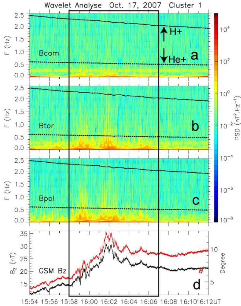
Fig.3.27 Wavelet analyses for magnetic field of SC1 in the field-aligned coordinate system on 17 October 2007 (a, b, c). The black dotted and dashed lines represent the gyrofrequencies of \text{H}^+ and \text{He}^+ . The black and red lines in Panel (d) show the magnetic field B_z component and the magnetic elevation angle \theta in GSM coordinates.
