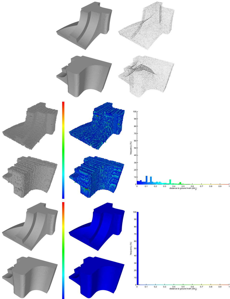
Figure 2.4: fandisk data set : comparison of visibility-based reconstructions over different data-driven complexes. First and second rows: ground truth model and input point cloud. Third and fourth rows: reconstruction over an adaptive region-based octree. Fifth and sixth rows: reconstruction over a Delaunay triangulation. The graphs on the right are histograms of the distance to ground truth of the reconstructions.
