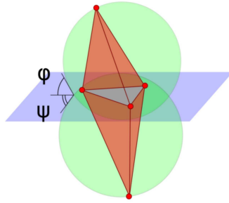
Figure 3.7: Soft 3D \beta -skeleton : a facet of the triangulation, its two adjacent tetrahedra (red) and their circumscribing spheres (green). Their angles \phi and \psi with the plane (blue) of the facet influence the weight of this facet.
