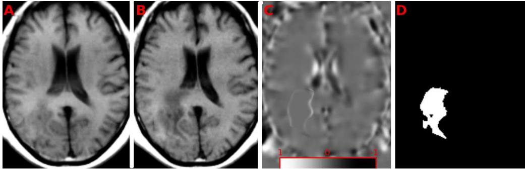
Figure 9.3: Mass effect analysis. A,B) Two-years follow-up sequence of T1 MRIs for a low-grade glioma patient, C) divergence scalar map associated to the longitudinal deformation, D) prior mask for the tumor.
