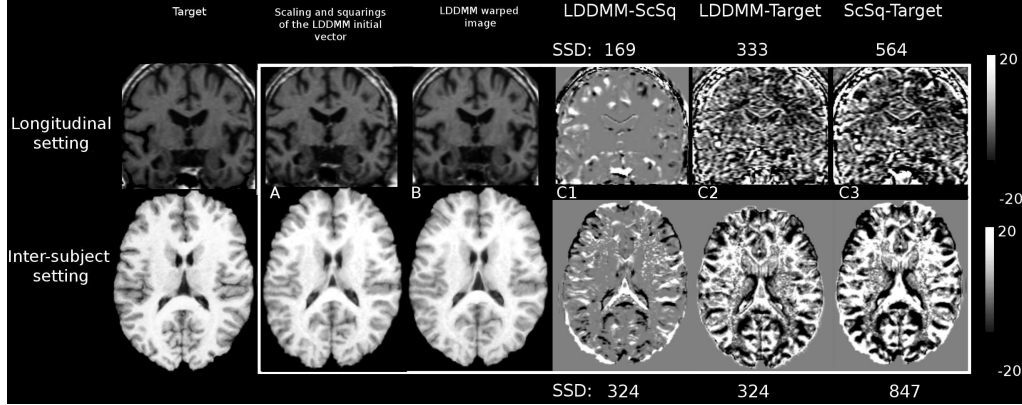
Figure 4.5: Lie group exponential (scaling and squaring) applied to the LDDMM initial vector for the intra and the inter-subject registration. From left to right: Target image, A) resulting warped source image with the scaling and squaring, B) warped source imaged with the LDDMM, and differences between C1) LDDMM and Scaling and Squaring warped images, C2) LDDMM warped and target images and C3) scaling and squaring warped and target images. We note that although the scaling and squaring provides worse matching with respect to the target, the resulting warped image is still close to the LDDMM one.
