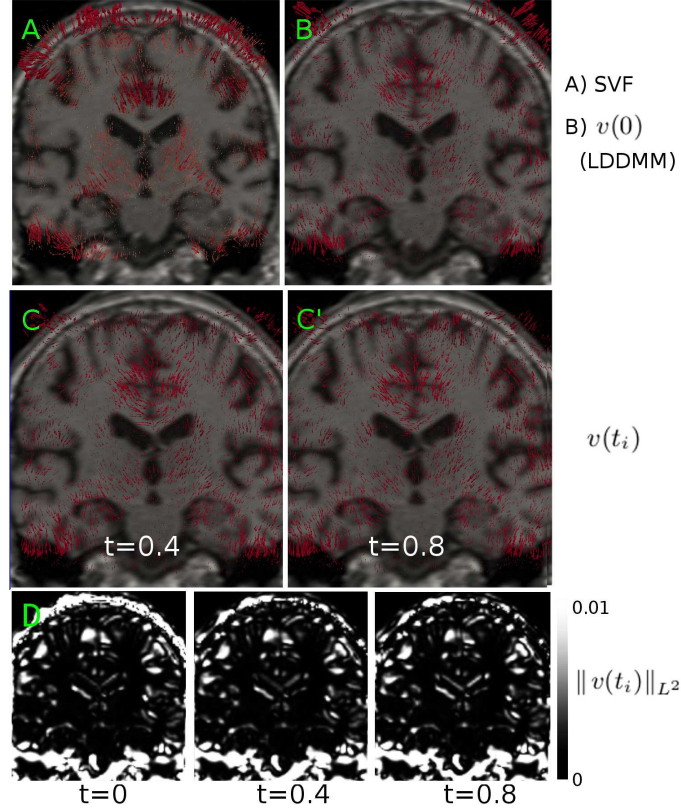
Figure 4.2: Intra-subject registration. Tangent representation for the intra-subject longitudinal deformation estimated by A) the SVF, and B) the LDDMM (initial tangent vector v(0) ) settings. C,C') LDDMM time varying velocity field v(t_i) at time points t_i = 0.4 and 0.8 , and D) associated magnitude measured by the L^2 norm.
