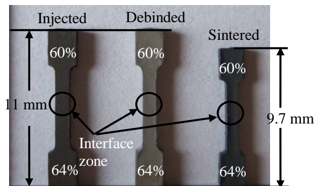
Figure 75. Beam-bending test specimens injected with two different feedstocks (60% for one half and 64% for the other half) after the injection, debinding and sintering stages
