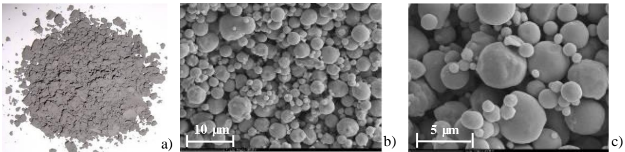
Figure 27. 316L stainless steel powders ( D_{50}=3.4\ \mu\text{m} ) used in the proposed investigations
