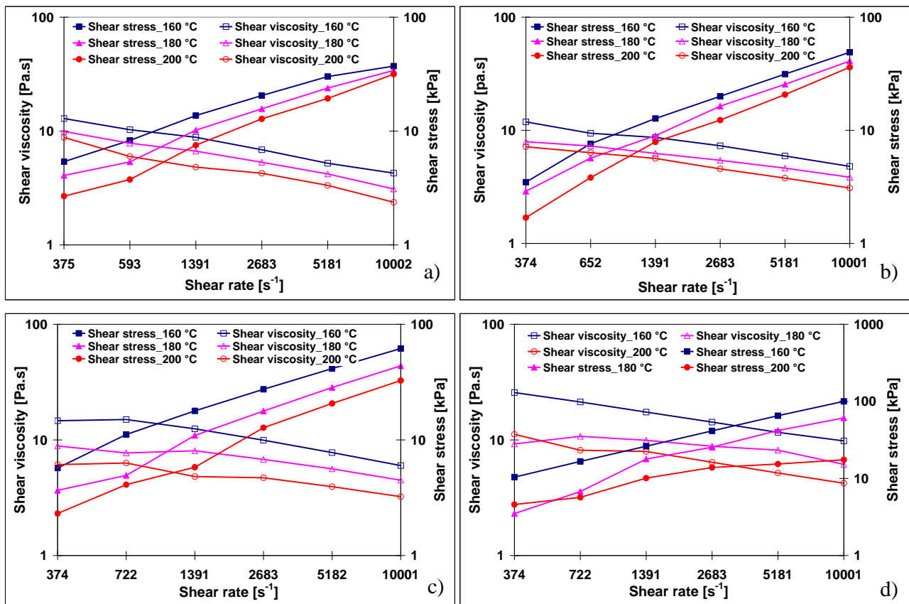
Figure 52. Shear viscosity and shear stress vs. shear rate for the 316L stainless steel feedstocks ( D_{50}=3.4 \mu\text{m} ) at different temperatures with powder volume loadings of a) 60%, b) 62%, c) 64% and d) 66% according to formulation F3.
