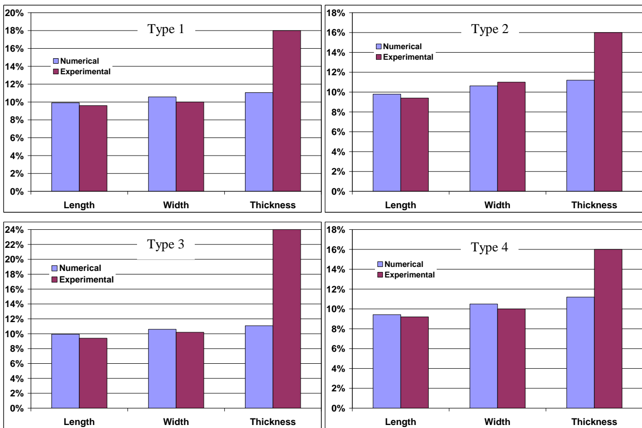
Figure 101. Comparison between the experimental and the numerical shrinkages of the four types of micro specimen (316L stainless steel, D_{50}=3.4 \mu\text{m} , formulation F3, powder volume loading=62%) after the sintering stage (heating rate=5 °C/min)
