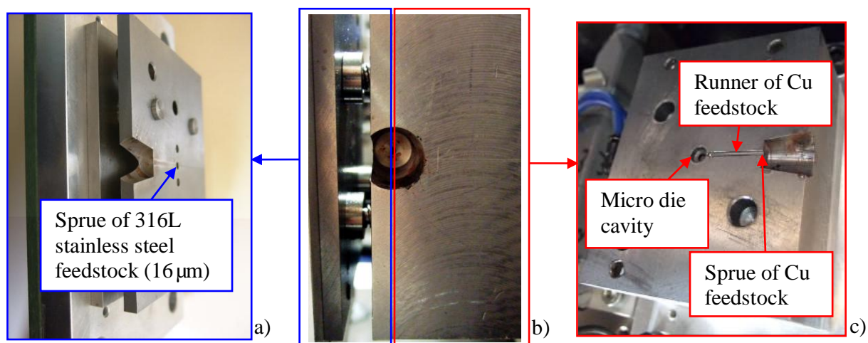
Figure 67. Three-plate mold for bi-material injection moulding dedicated to the injection of feedstocks based on 316L stainless steel (16 µm) and Cu powder according to formulation F3, a) fixed plate side; b) three plate mould in closed state and c) mobile plate side
