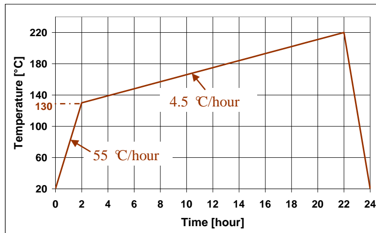
Figure 71. Debinding cycle involved in the thermal debinding stage
