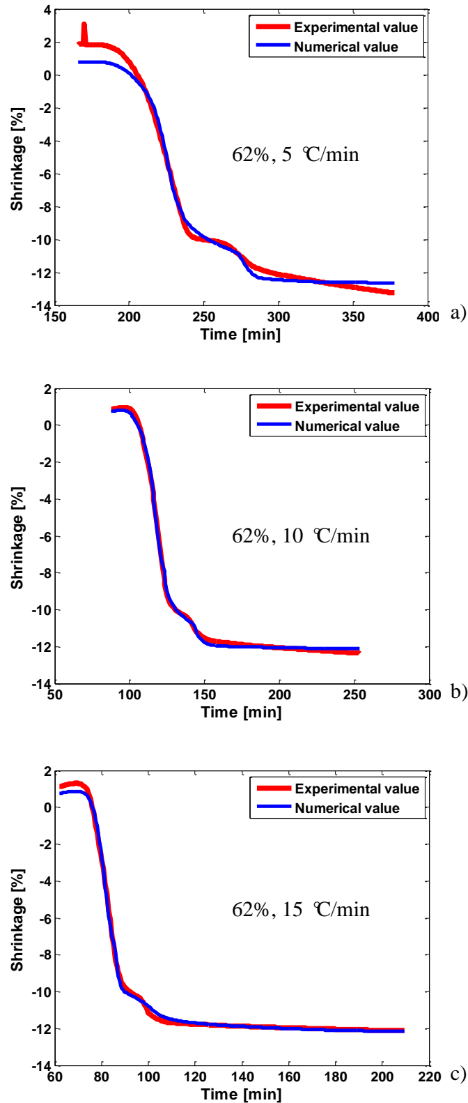
Figure 91. Comparison between experimental shrinkages in vertical dilatometer during the sintering stages with different heating rates and identified ones for 316 L stainless steel feedstock ( D_{50}=3.4 \mu\text{m} , formulation F3, powder volume loading is 62%)
