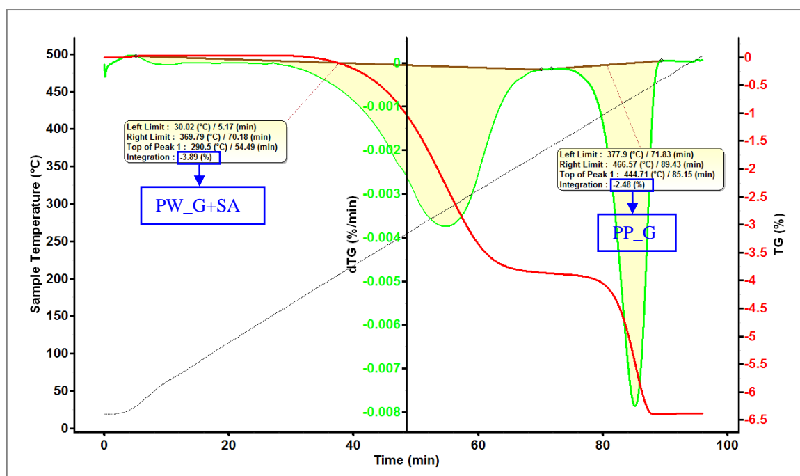
Figure 62. TGA results of the split specimens from micro injection with 316L stainless steel feedstock ( D_{50}=3.4 \mu\text{m} , formulation F3, powder volume loading=62%)
