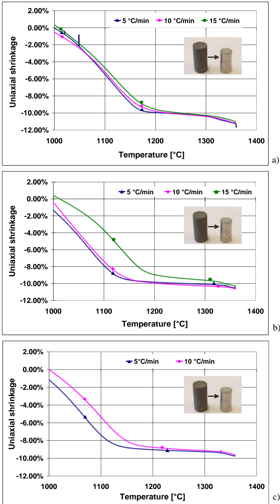
Figure 89. Uniaxial shrinkage \lambda vs. temperature from free sintering test in vertical dilatometer for 316 L stainless steel feedstock ( D_{50}=3.4 \mu\text{m} , formulation F3) with the powder volume loading of a) 62%; b) 64%; c) 66%
