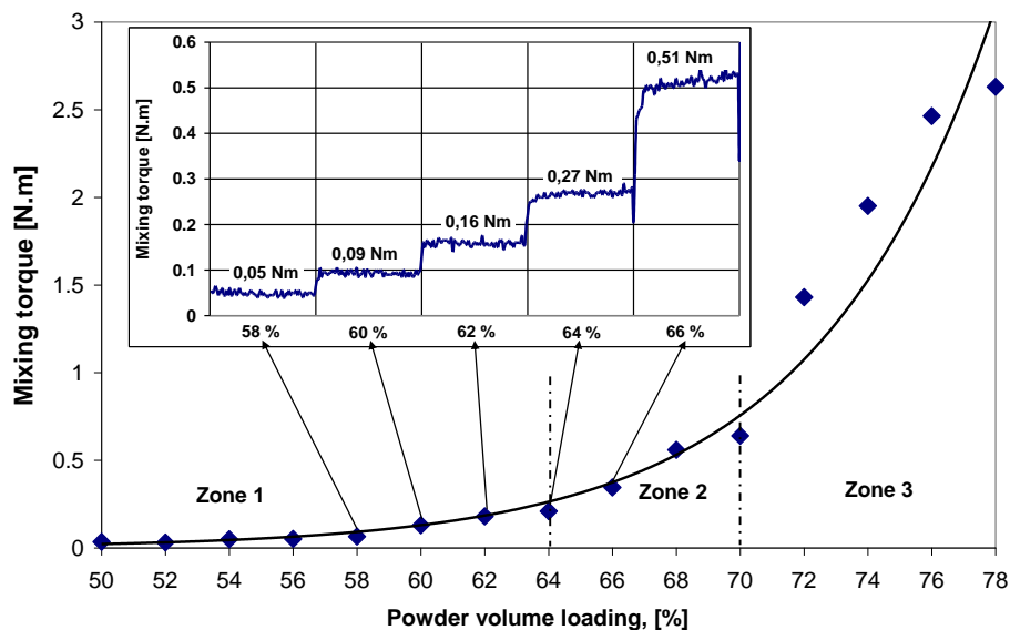
Figure 43. Mixing torque vs. powder volume loading obtained through the continuously rising powder loading technique (316L stainless steel powder, D_{50}=3.4 \mu\text{m} , feedstock formulation F3, mixing temperature=160 °C, mixing time=30 min)
