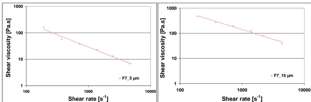
Figure 42. Shear viscosity vs. shear rate corresponding to feedstock formulations F7 (group #3)
