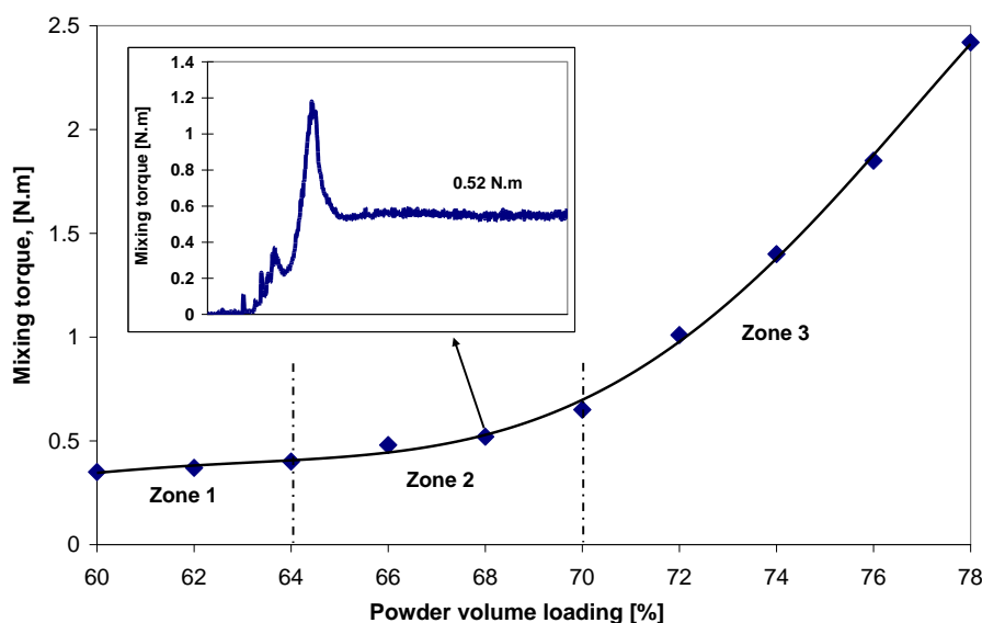
Figure 44. Mixing torque vs. powder volume loading related to the mixing tests by separately rising powder loading (316L stainless steel powder, D_{50}=3.4 \mu\text{m} , feedstock formulation F3, mixing temperature=160 °C, mixing time=30 min)
