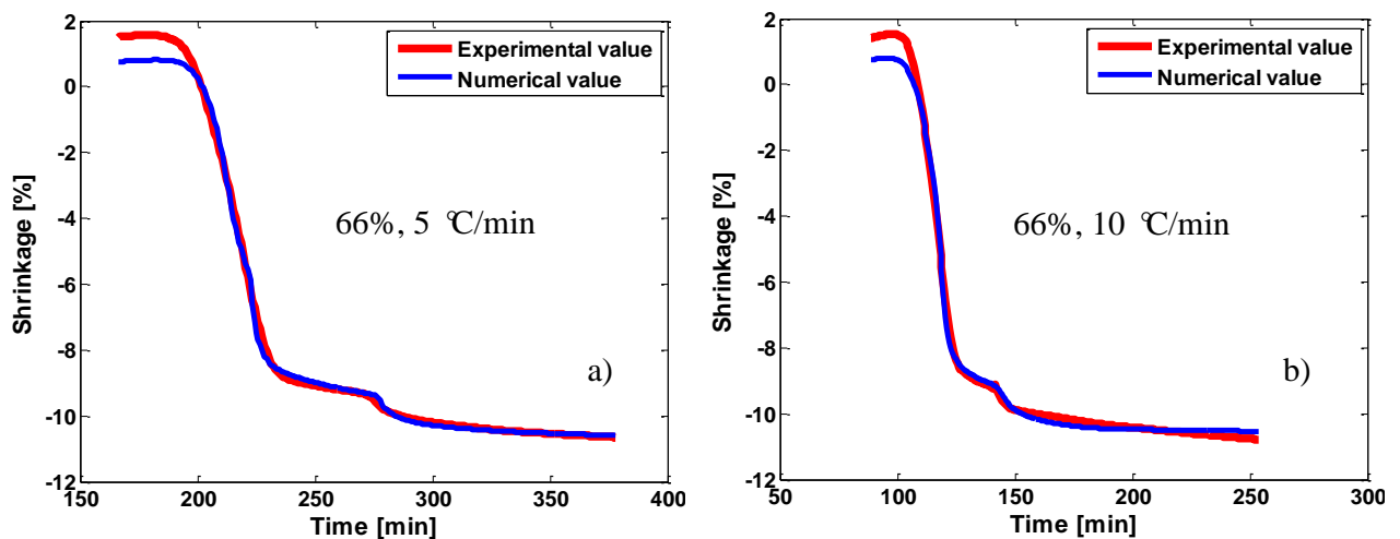
Figure 93. Comparison between experimental shrinkages in vertical dilatometer during the sintering stages with different heating rates and identified ones for 316 L stainless steel feedstock ( D_{50}=3.4 \mu\text{m} , formulation F3, powder volume loading is 66%)
