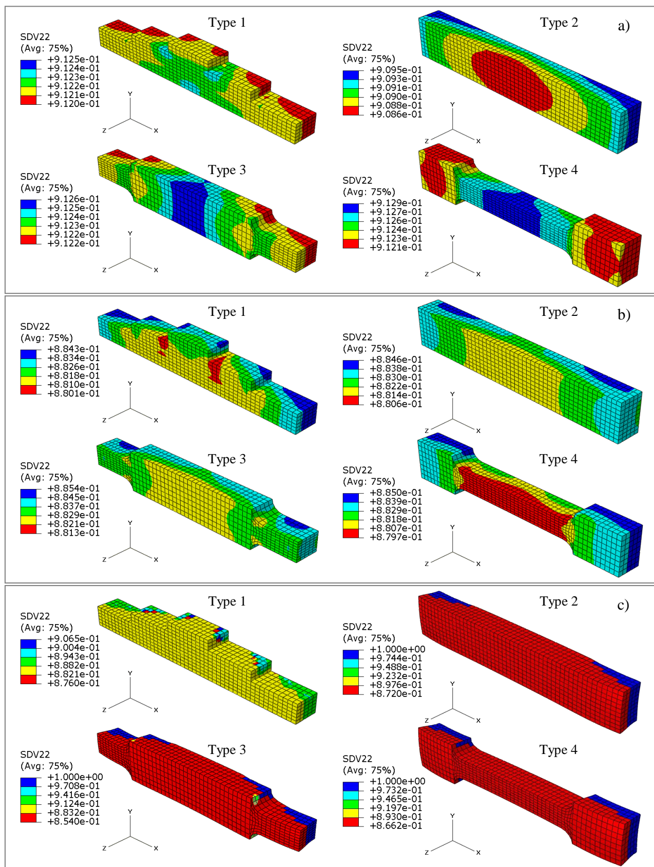
Figure 117. Numerical relative densities of the four types of micro-specimen (316L stainless steel, D_{50}=3.4 \mu\text{m} , formulation F3, powder volume loading=64%) after the sintering stage with heating rate of a) 5 °C/min, b) 10 °C/min and c) 15 °C/min
