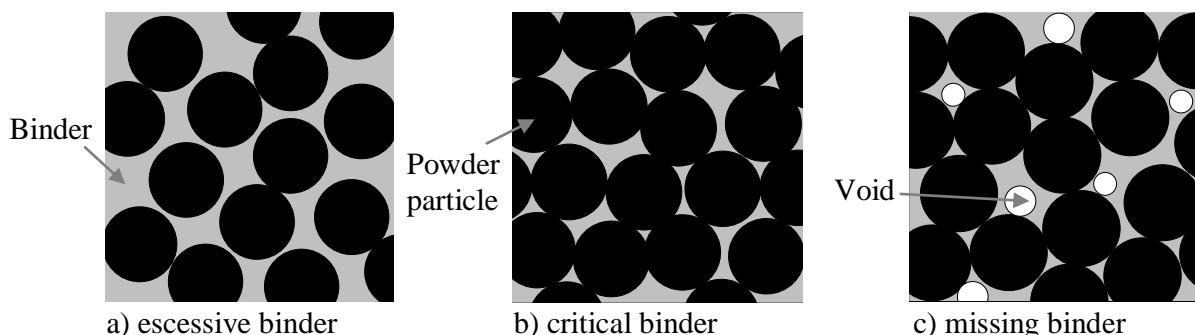
Figure 48. Three possible situations in a powder-binder mixture [23]: a) excess of binder, b) critical binder concentration, and c) voids due to insufficient binder
