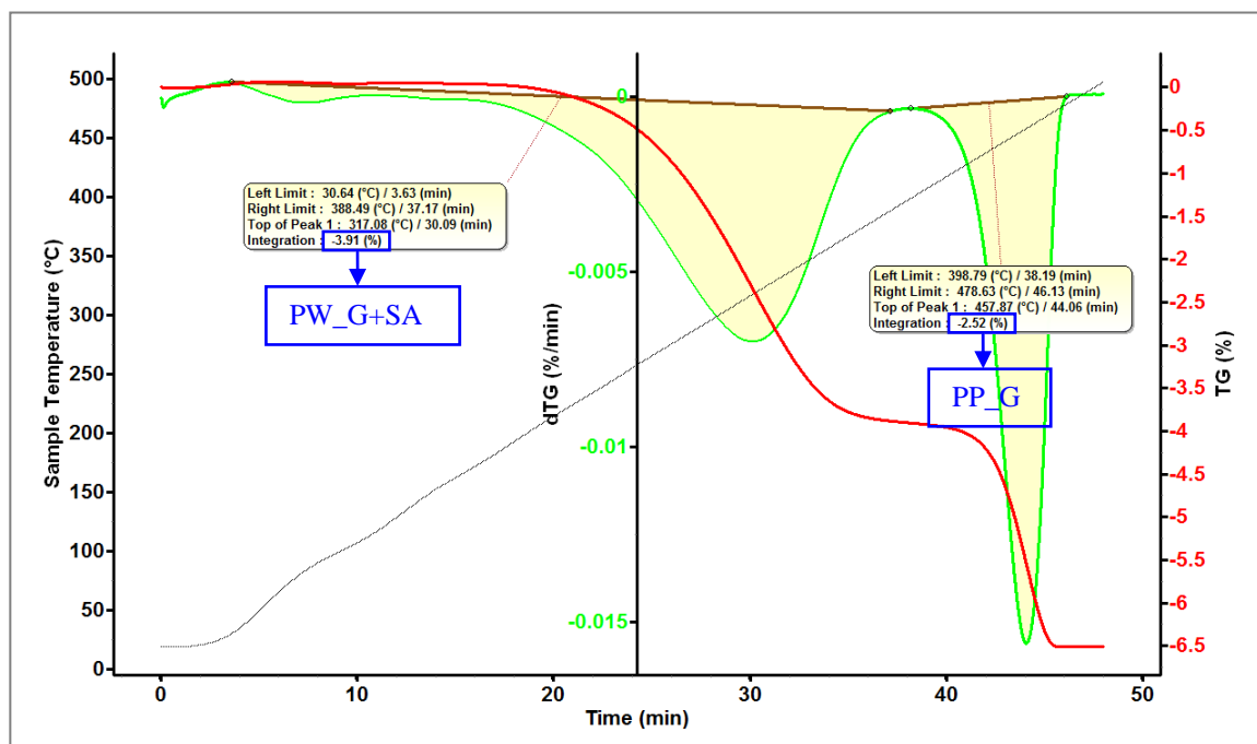
Figure 61. TGA results for the entire specimens from micro injection with 316L stainless steel feedstock ( D_{50}=3.4 \mu\text{m} , formulation F3, powder volume loading=62%)
