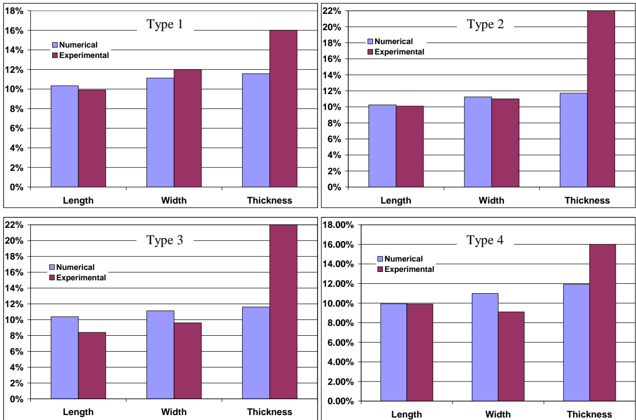
Figure 106. Comparison between the experimental and the numerical shrinkages of the four types of micro specimen (316L stainless steel, D_{50}=3.4 \mu\text{m} , formulation F3, powder volume loading=62%) after the sintering stage (heating rate=10 °C/min)
