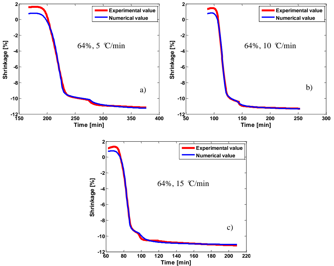
Figure 92. Comparison between experimental shrinkages in vertical dilatometer during the sintering stages with different heating rates and identified ones for 316 L stainless steel feedstock ( D_{50}=3.4 \mu\text{m} , formulation F3, powder volume loading is 64%)
