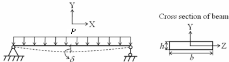
Figure 83. Simply supported beam model for beam-bending tests
