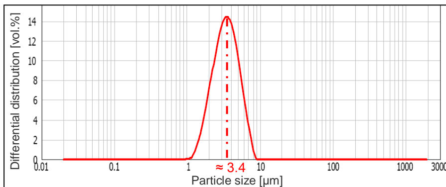
Figure 28. Particle size distribution for 316L stainless steel powders ( D_{50}=3.4\ \mu\text{m} ) used in the related investigations
