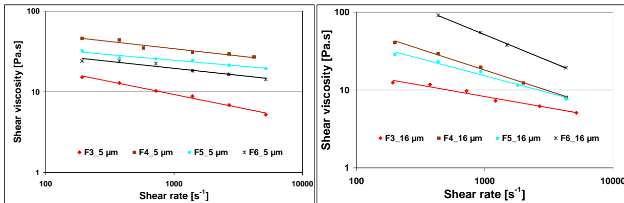
Figure 41. Shear viscosity vs. shear rate corresponding to feedstock formulations F3, F4, F5 and F6 (group #2)
