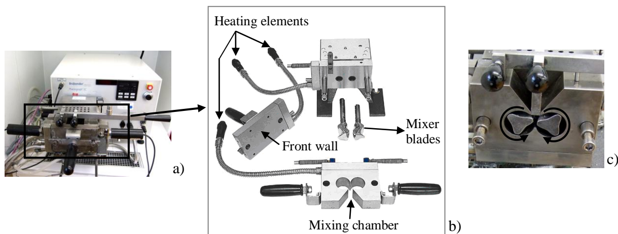
Figure 33. Brabender ® twin-screw mixer W 50 EHT, a) general view of the mixer; b) assembly of mixing chamber; c) the two mixer blades and their counter-rotation towards each other
