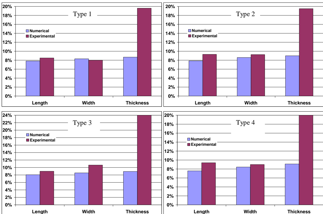
Figure 108. Comparison between the experimental and the numerical shrinkages of the four types of micro specimen (316L stainless steel, D_{50}=3.4 \mu\text{m} , formulation F3, powder volume loading=62%) after the sintering stage (heating rate=15 °C/min)
