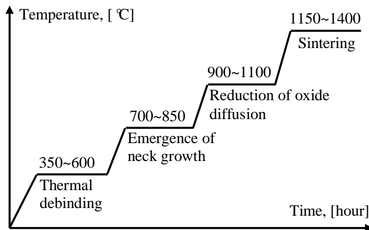
Figure 19. Typical (solid state diffusion) kinetic sintering cycle for stainless steel feedstock with four segments
