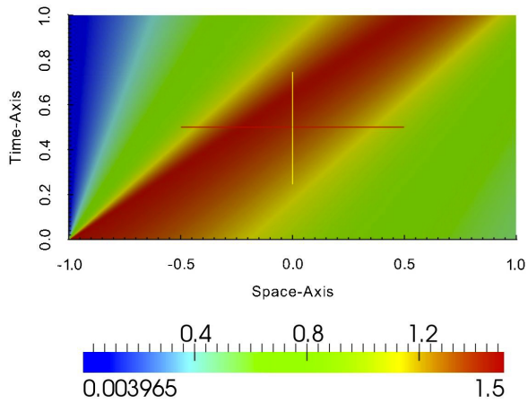
Figure V.9 – Burgers with u_3^0
