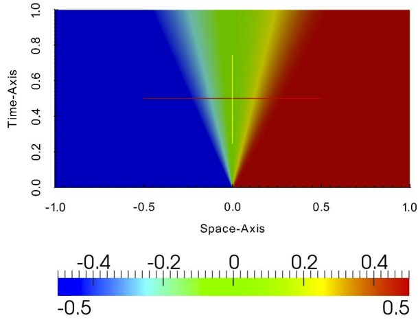
Figure V.1 – Burgers with u_1^0
