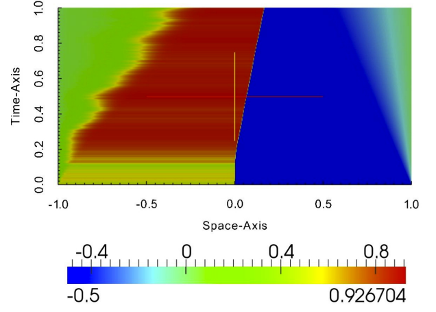
Figure V.6 – Stochastic Burgers with u_2^0
