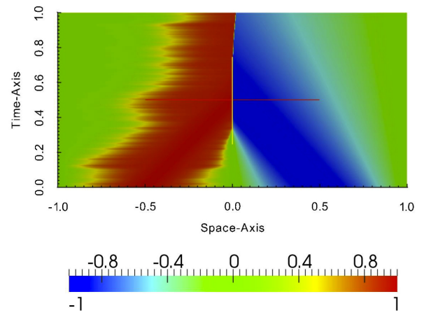
Figure V.14 – Stochastic Burgers with u_4^0
