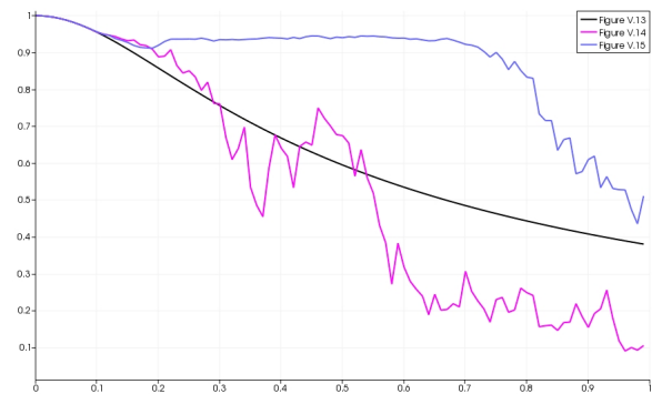
Figure V.16 – Pathwise for x = -0.5
