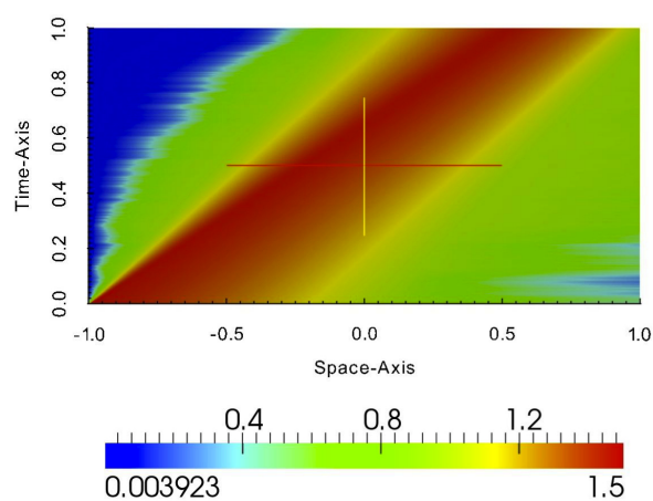
Figure V.10 – Stochastic Burgers with u_3^0
