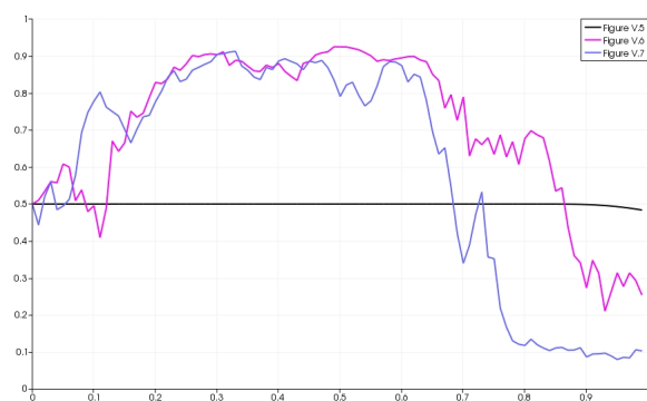
Figure V.8 – Pathwise for x = -0.5
