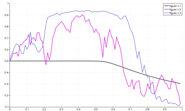
Figure V.4 – Pathwises for x = 0.3
