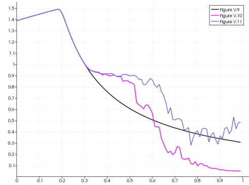
Figure V.12 – Pathwise for x = -0.7
