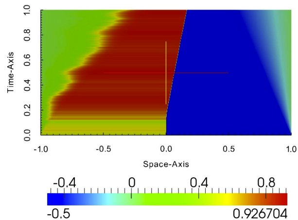
Figure V.6 – Stochastic Burgers with u_2^0
