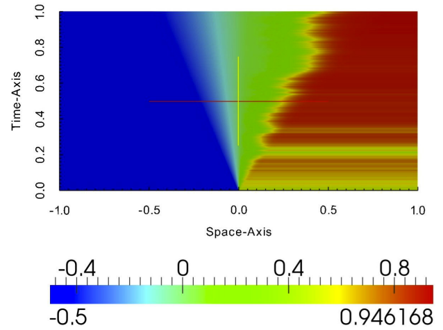
Figure V.2 – Stochastic Burgers with u_1^0
