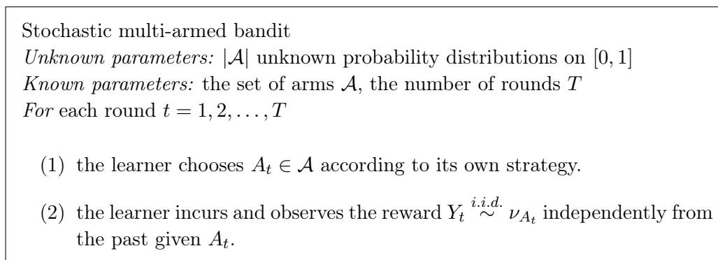
Figure 1.1: The stochastic multi-armed bandit game.
