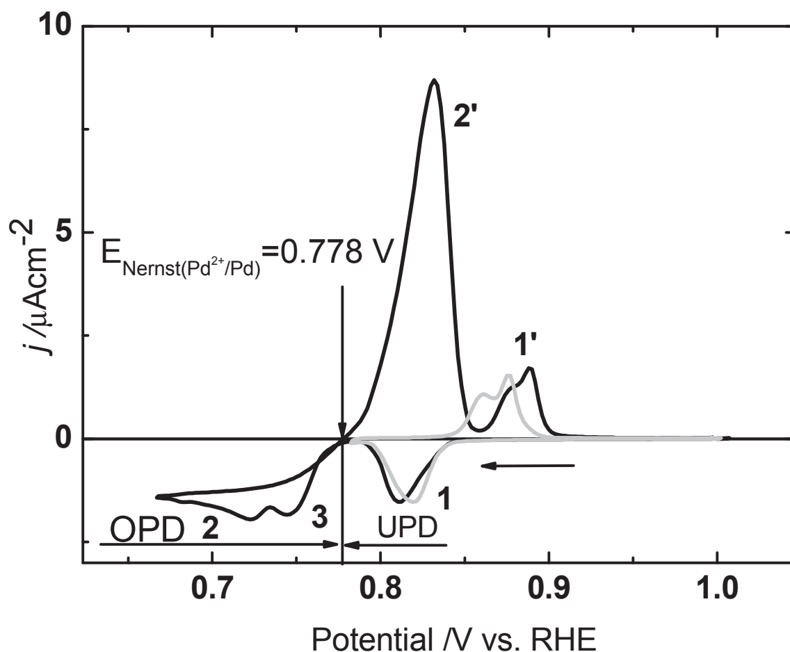
Figure II.3: Cyclic voltammograms of Au(111) in 0.1 M \text{H}_2\text{SO}_4 + 0.1 mM \text{PdCl}_2 + 3 mM \text{HCl} . Black line: 1 st cycle; light grey line: 2 nd cycle. Scan rate: 0.1 \text{ mV}\cdot\text{s}^{-1} .
