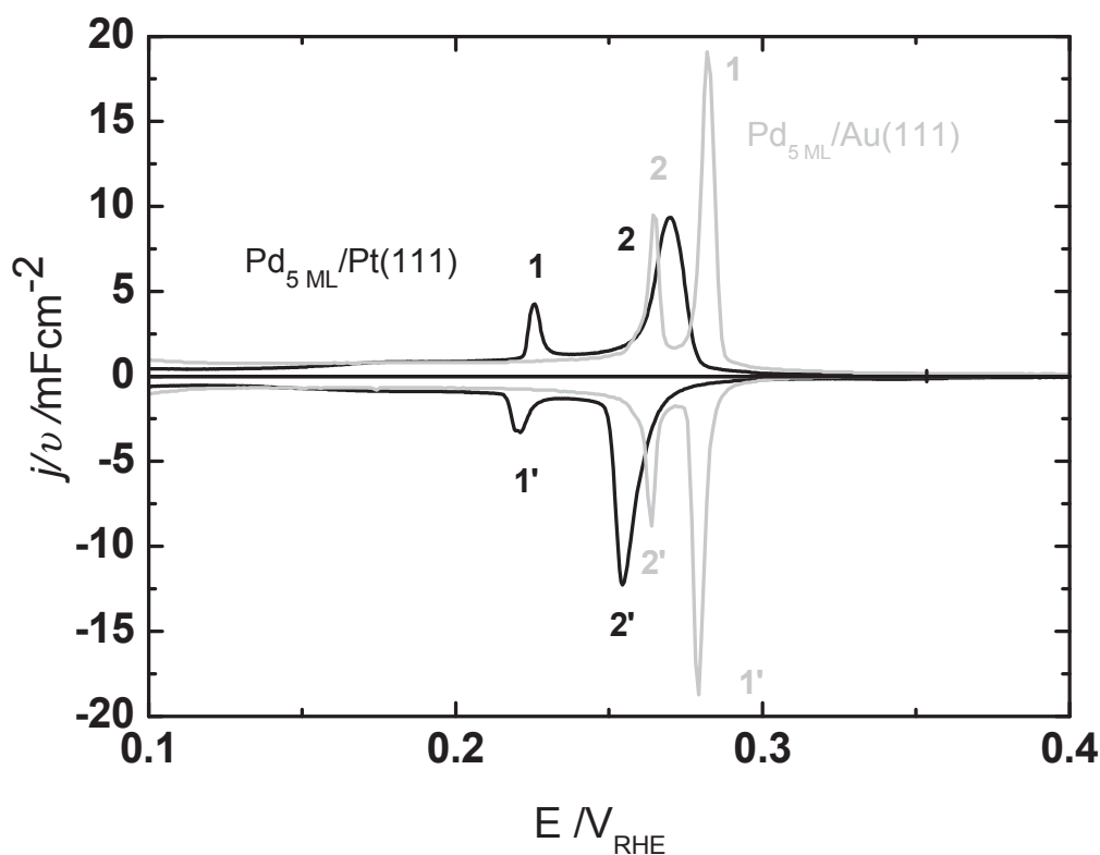
Figure II.29: CV for the Pd 5 ML /Au(111) (light grey line), Pd 5 ML /Pt(111) (black line) [1] in 0.1 M H 2 SO 4 .
