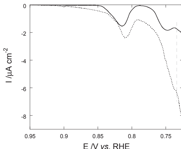
Figure III.13: Voltammetric Pd deposition in \text{PdCl}_2 10^{-4} \text{ M} + \text{HCl } 3 \cdot 10^{-3} \text{ M} + \text{H}_2\text{SO}_4 0.1 \text{ M} at 0.1 \text{ V} \cdot \text{s}^{-1} : comparison between currents measured in a classical glass cell in hanging meniscus configuration and in the in situ SXR electrochemical cell.
