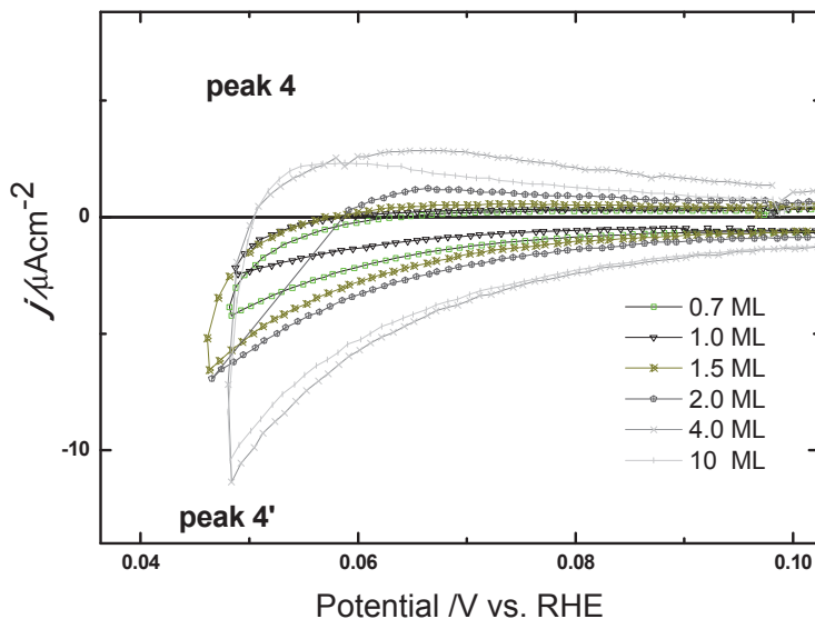
Figure II.23: Voltammograms of Pd x ML/Au(111) in 0.1 M H 2 SO 4 . Same data as Figure II.18, enlarged scale. Sweep rate: 1 mV·s -1 .
