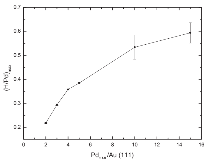
Figure IV.17: Maximum hydrogen insertion rate (\text{H/Pd})_{\text{max}} as a function of Pd/Au(111) film thickness.
