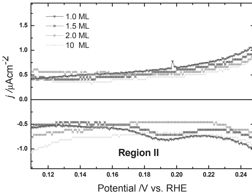
Figure II.19: Voltammograms of Pd x ML /Au(111) in 0.1 M H 2 SO 4 . Same data as
