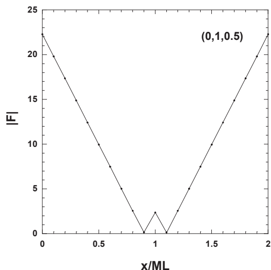
Figure III.10: Pd x ML/Au(111): simulated structure factor for the (0,1,0.5) reflexion in the case of layer-by-layer pseudomorphic growth.
