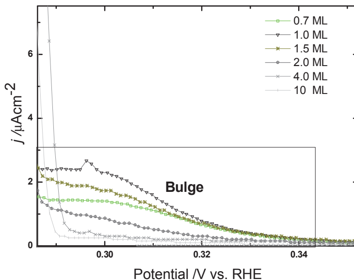
Figure II.22: Voltammogram of Pd x ML/Au(111) in 0.1 M H 2 SO 4 . Same data as Figure II.18, enlarged scale. Sweep rate: 1 mV·s -1 .
