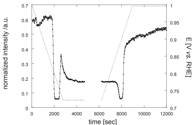
Figure III.11: In situ SXR diffraction signal recorded at (1,0,0.5) during Pd deposition and dissolution in PdCl 2 10 -4 M + HCl 3·10 -3 M + H 2 SO 4 0.1 M. Each point corresponds to 17 s recording. Deposition is made with potential scan from 0.998 down to 0.723 V vs. RHE at 0.1 mV·s -1 , followed by chronoamperometry at this last value potential. Potential is maintained at 0.723 V vs. RHE till 6210 s (data have not been recorded between 4700 and 6200 s). Dissolution is made with a scan up to the initial potential value at the same rate. Continuous line with circles: normalized diffracted signal; dashed line: potential value.
