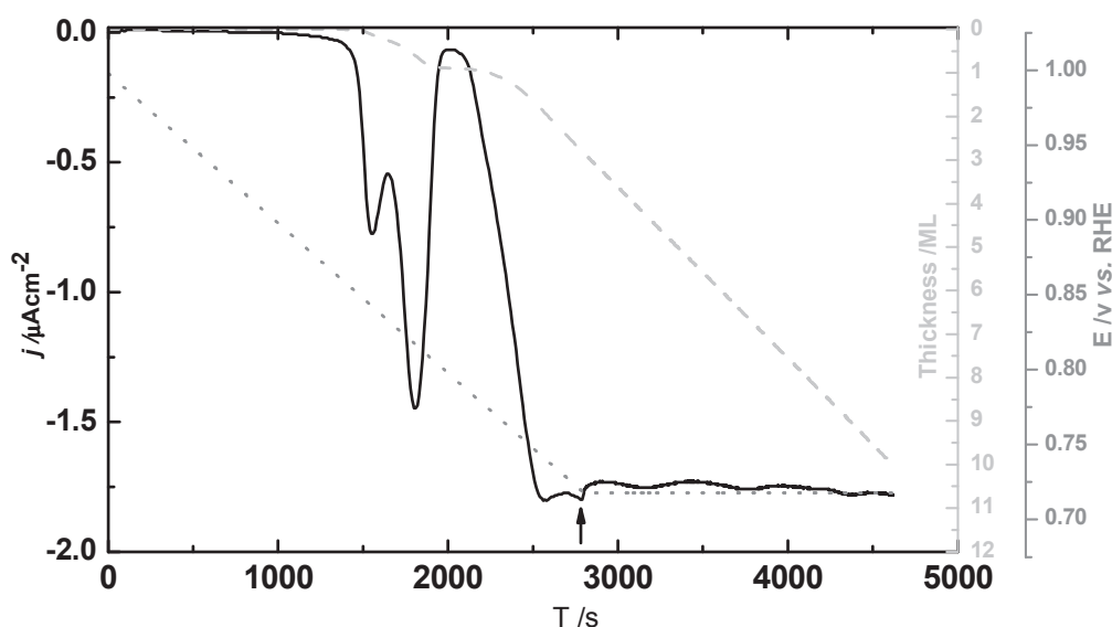
Figure II.9: Typical deposition curve in 0.1 M H 2 SO 4 + 0.1 mM PdCl 2 + 3 mM HCl solution. Au(111) electrode is dipped into the solution at 0.998 V vs. RHE. The potential is swept down to 0.718 V vs. RHE with a scan rate of 0.1 mV·s -1 and hold at 0.718 V vs. RHE until the desired amount of Pd is deposited. Solid line: current; dashed line: integrated charge; dotted line: applied potential; Arrow indicates the onset of CA deposition.
