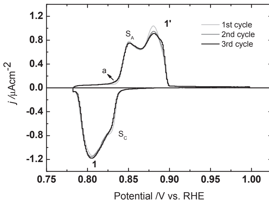
Figure II.7: Cyclic voltammograms of Au(111) in 0.1 M H 2 SO 4 + 0.1 mM PdCl 2 + 3 mM HCl; sweep rate: 0.1 mV·s -1 .
