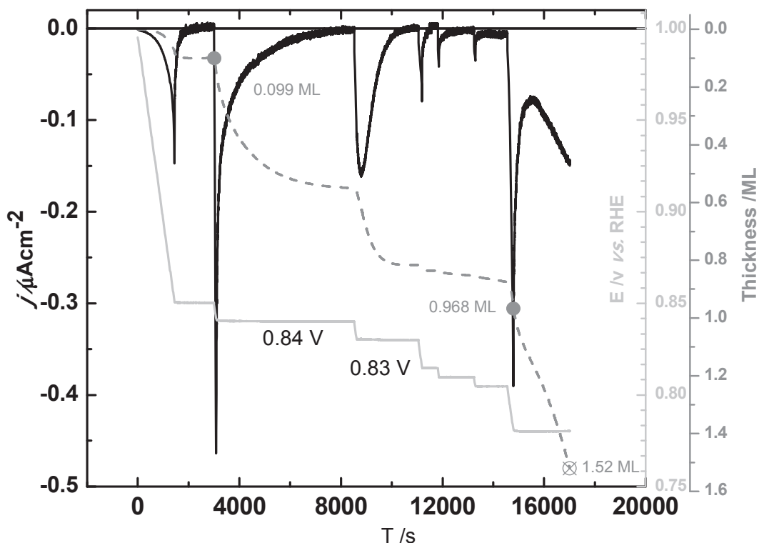
Figure III.2: Pd deposition on Au (111) in 0.1 M \text{H}_2\text{SO}_4 + 0.1 mM \text{PdCl}_2 + 3 mM \text{HCl} . Current (solid line), equivalent thickness (dash line) and applied potential (grey line; scan parts at 0.1 \text{ mV}\cdot\text{s}^{-1} ).
