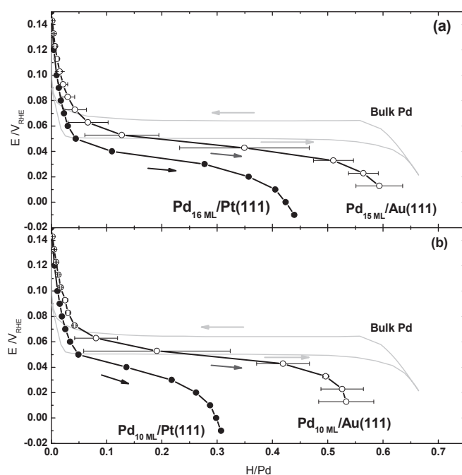
Figure IV.18: H insertion isotherms of Pd bulk [1] (continuous light grey line), Pd x ML /Au(111) (open circles) and Pd x ML /Pt(111) [7] (close circles) for about 15 ML (a) and 10 ML (b) as equivalent thickness.
