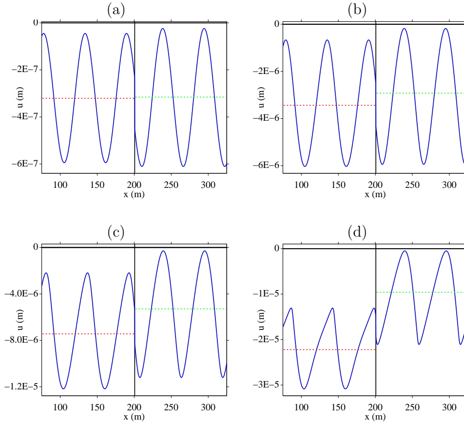
Figure 6.5: Model 1 (6.22): snapshots of the elastic displacement for various amplitudes v_0 of the incident elastic velocity: 10^{-4} m/s (a), 10^{-3} m/s (b), 2 \times 10^{-3} m/s (c), and 5 \times 10^{-3} m/s (d). The vertical solid line denotes the location \alpha = 200 m of the crack. The dotted horizontal lines denote the mean value of the elastic displacement on both sides of \alpha .
