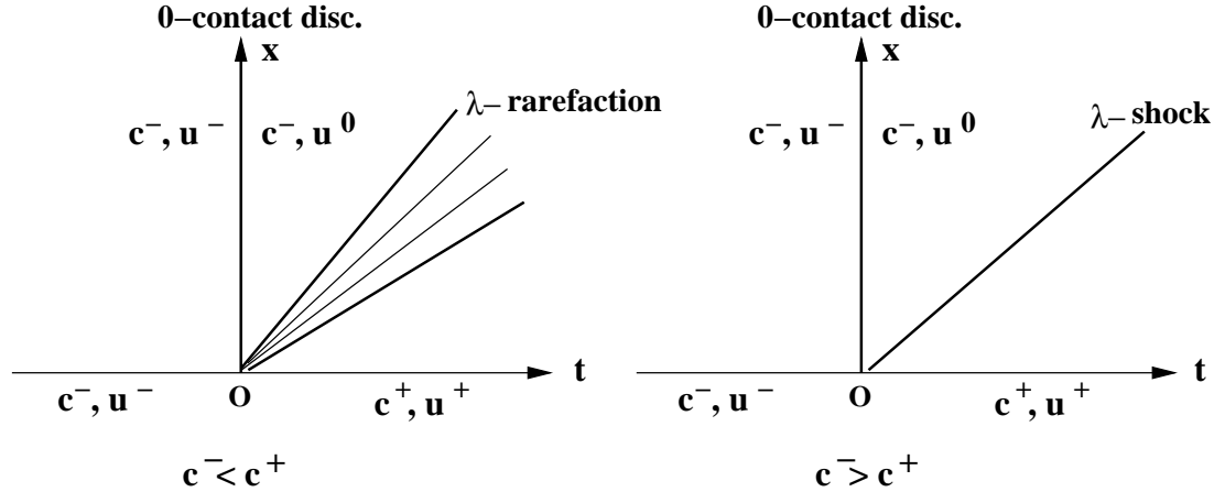
Figure 4.2: solution of the Riemann problem when f'' > 0 .
